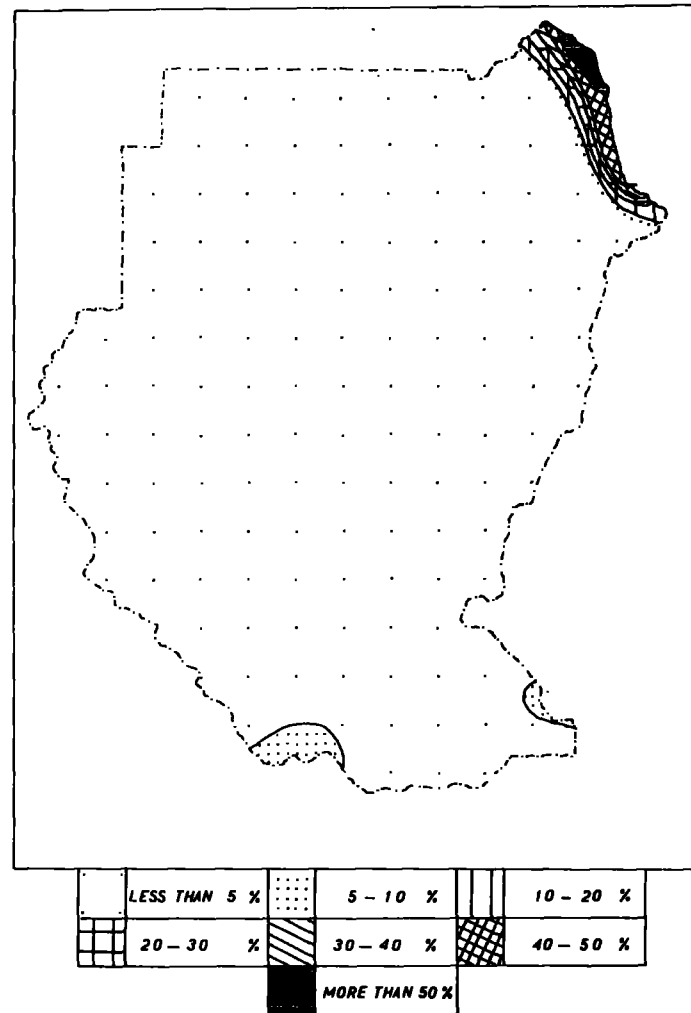
Fig. 39 November isomers
