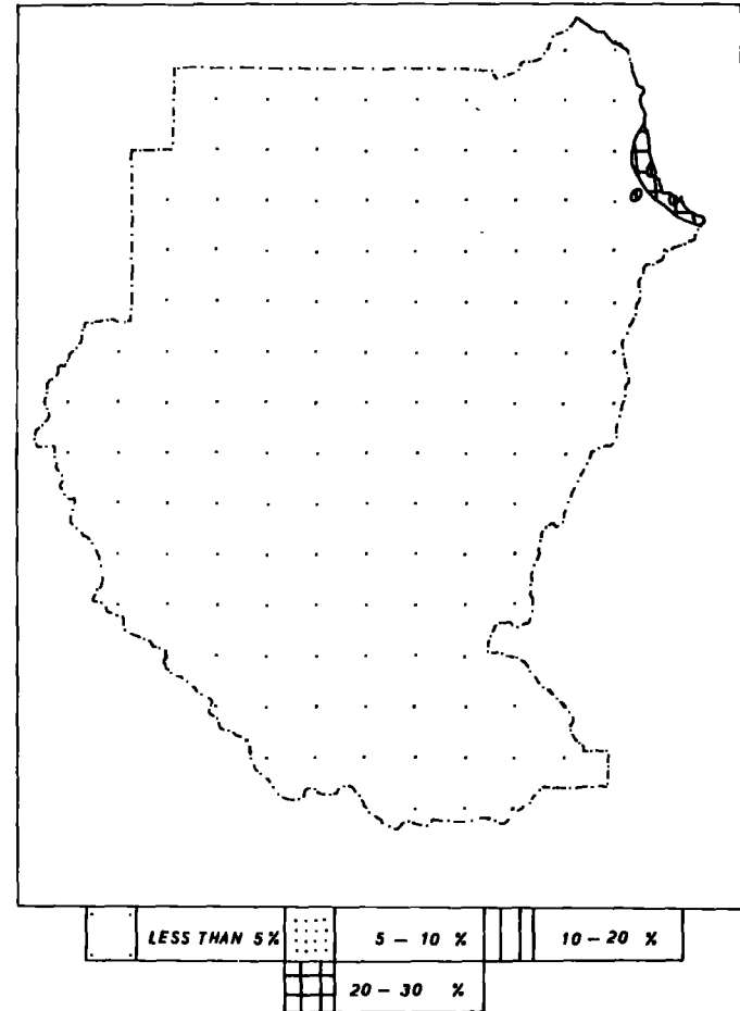
Fig. 41 December isomers
