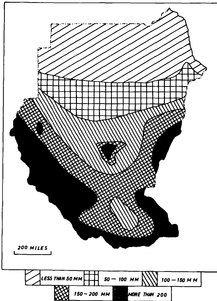
Fig. 32 August isohyets
