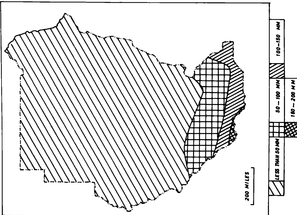
Fig. 23 April isohyets
