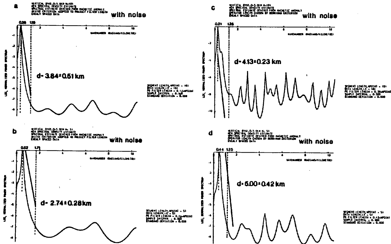
Figure 3.13 Natural logarithm; normalised MEM spectral density estimates for the vertical dyke model (Figure 3.6d) with random noise. (a) Profile length = 30km, Akaike criterion, (b) Profile length = 15km, Akaike criterion, (c) Profile length = 30km, Berryman criterion, (d) Profile length = 15km, Berryman criterion. Line of regression and depth estimate indicated for each graph.
