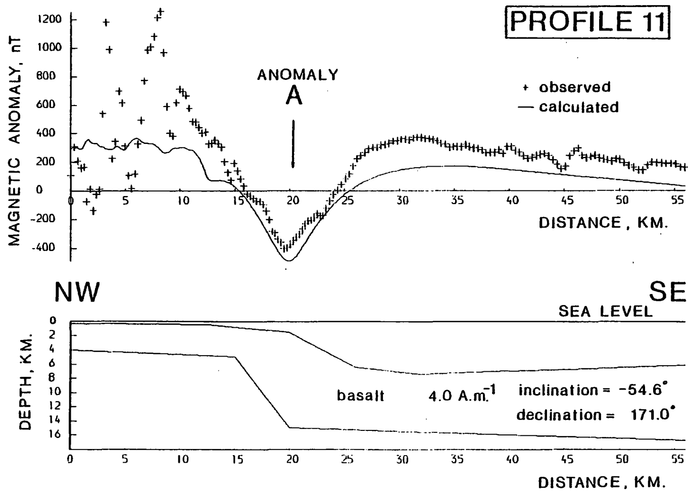
Figure 5.8 Interpretation of magnetic anomaly A along profile 11 as evidence for the offshore continuation of the plateau basalts.
