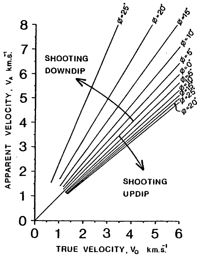
Figure 4.7 Effect of systematic CGP migration along the sea surface for H_o = 2000\text{m} , (a) Relationship of V_A and V_o for various angles of dip, \phi for updip and downdip shooting. (b) Variation of ratio V_A/V_o with angle of dip, \phi for a correct CGP gather and for updip and downdip shooting for the case of CGP migration.
