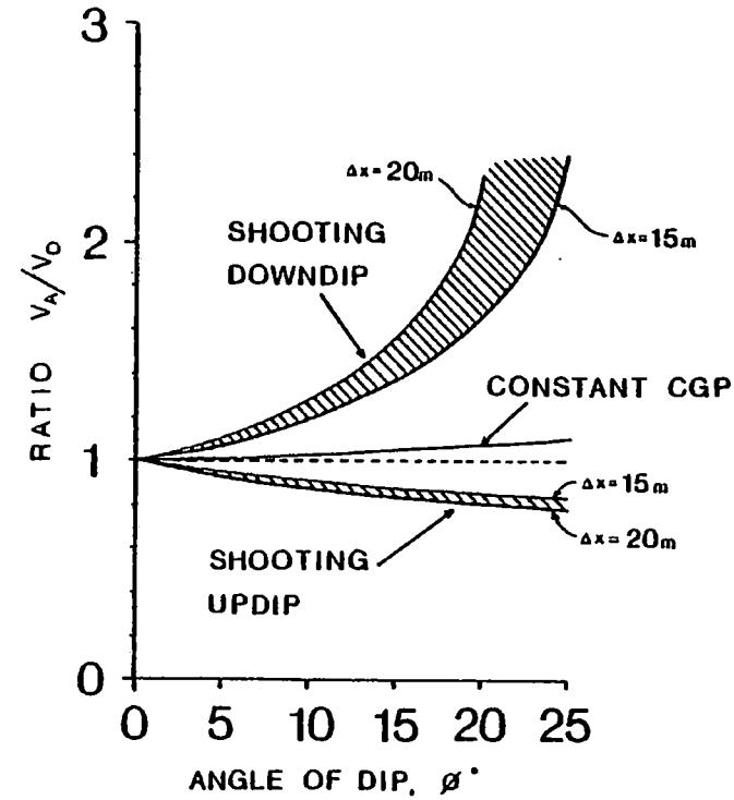
Figure 4.7 Effect of systematic CGP migration along the sea surface for H_o = 2000\text{m} , (a) Relationship of V_A and V_o for various angles of dip, \phi for updip and downdip shooting. (b) Variation of ratio V_A/V_o with angle of dip, \phi for a correct CGP gather and for updip and downdip shooting for the case of CGP migration.
