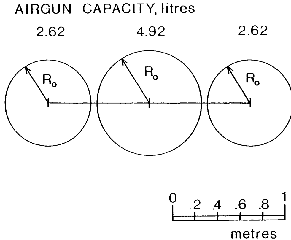
Figure 2.3 Schematic diagram to show the geometry of the 3 airgun bubble pulses 11ms after the shot instant. R_o represents the equilibrium radius of each respective airgun.
