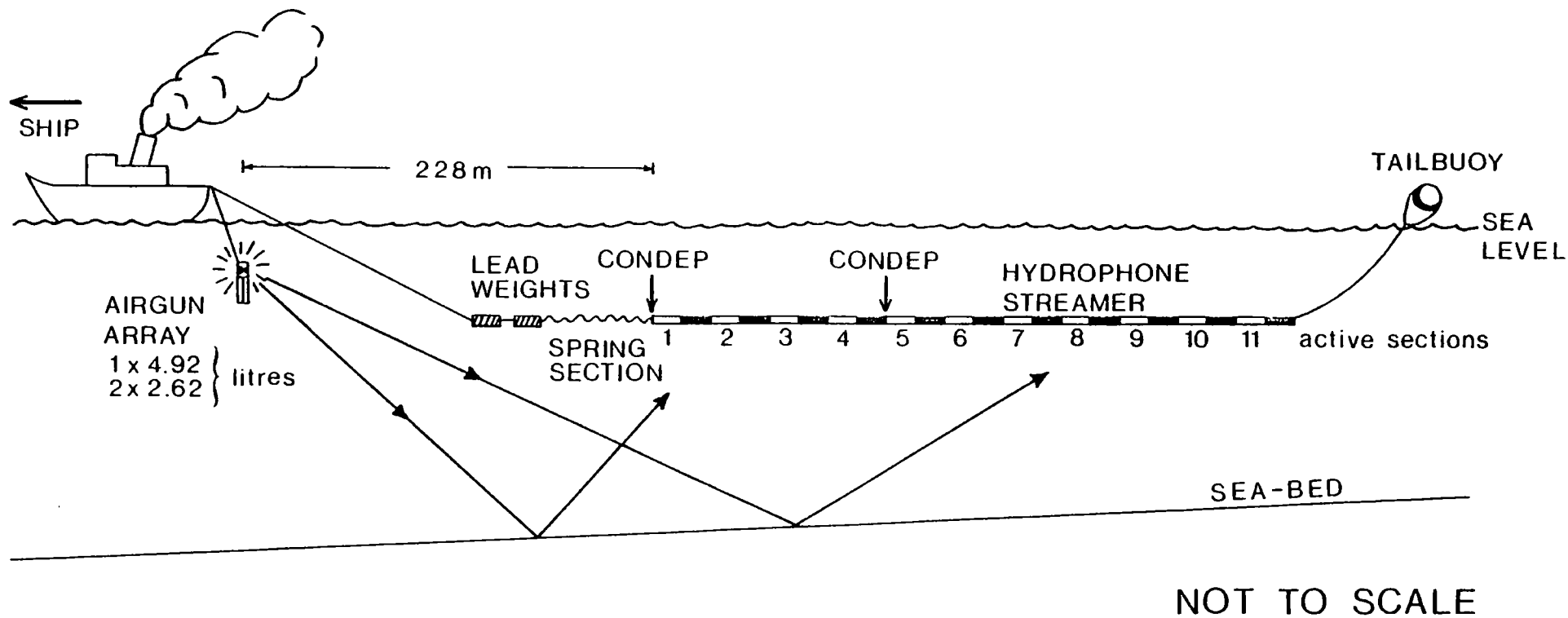
Figure 2.4 Towing arrangement of the hydrophone streamer and airgun array for the acquisition of multi-channel seismic reflection data, East Greenland marine survey, 1977.
