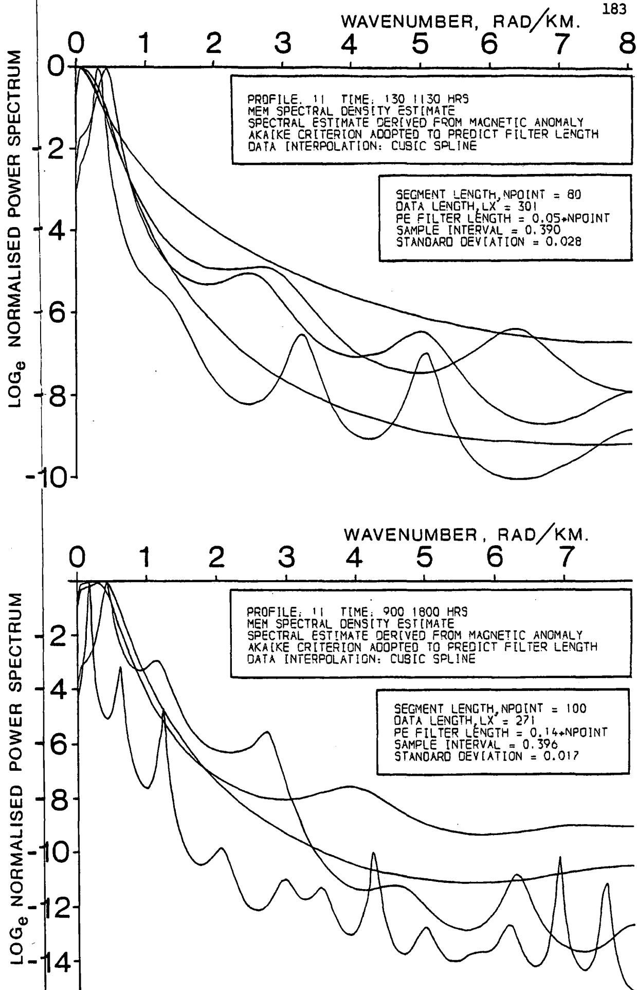
Figure 5.3 Natural logarithm of the MEM spectral density estimate curves for data analysed along profile 11.
