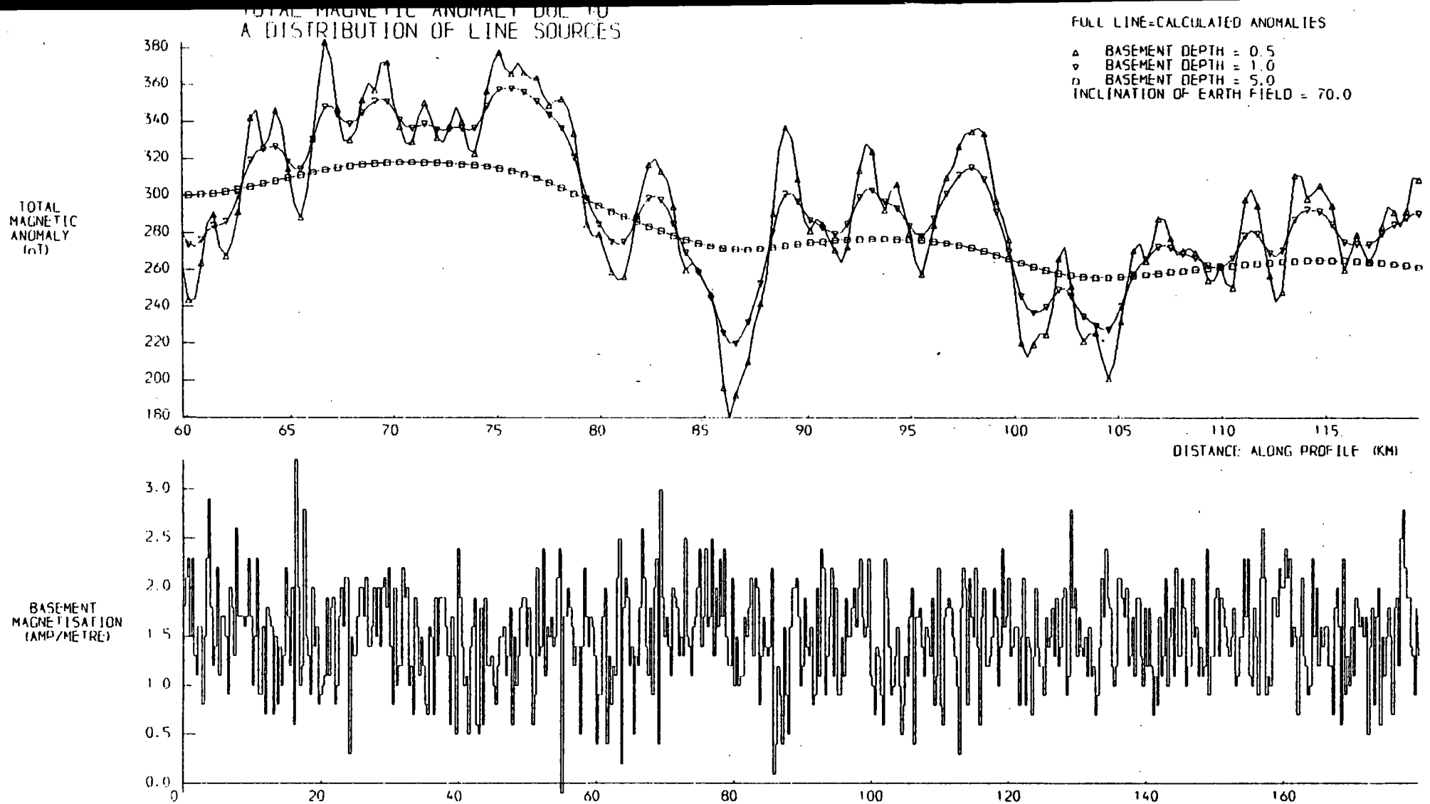
Figure 3.7 Model of randomly magnetised magnetic basement used for MEM spectral depth determination (generated by method of Treitel et al. , 1971).
