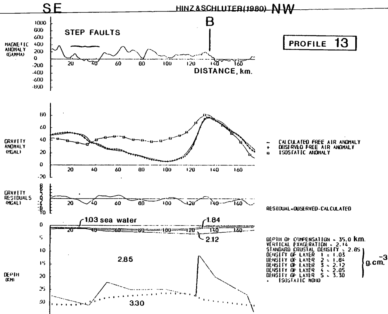
Figure 5.12 Gravity interpretation for profile 13. B represents the proposed ocean-continent boundary taken from Hinz and Schluter (1980).
