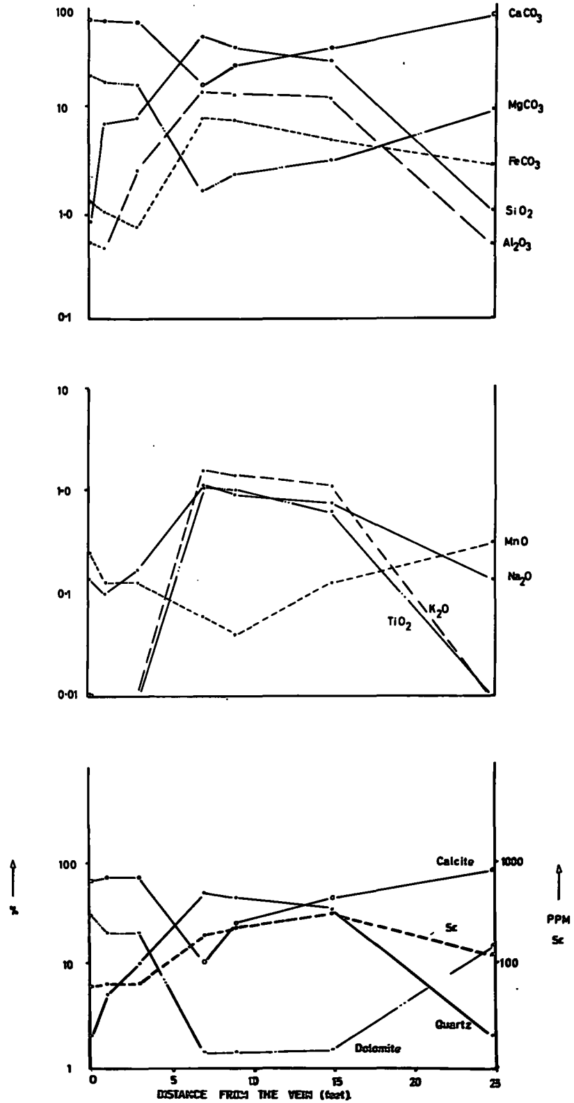
FIG 4-10 MASSON HILL QUARRY.
