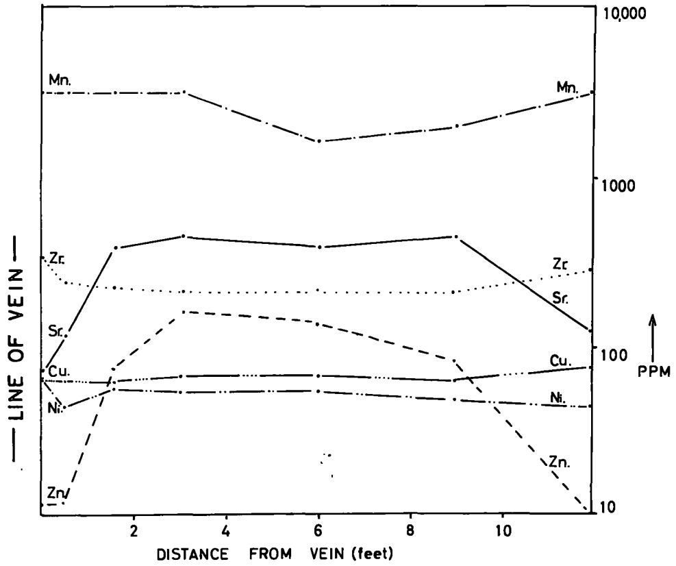
FIG. 6-13 TRACE ELEMENT VARIATIONS — WYNCH BRIDGE.
