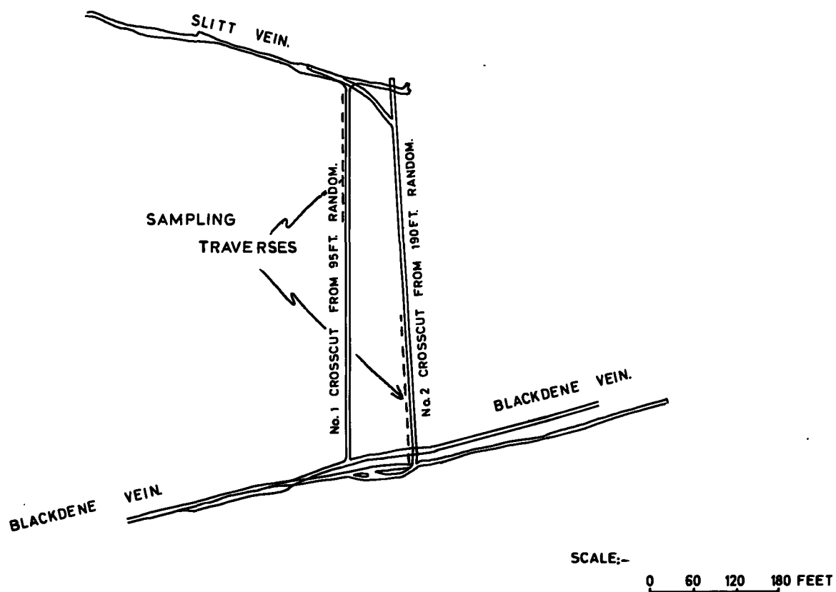
FIG. 2-3. SAMPLING LOCALITIES IN THE ALTERNATING BEDS AND SLATY HAZEL.
