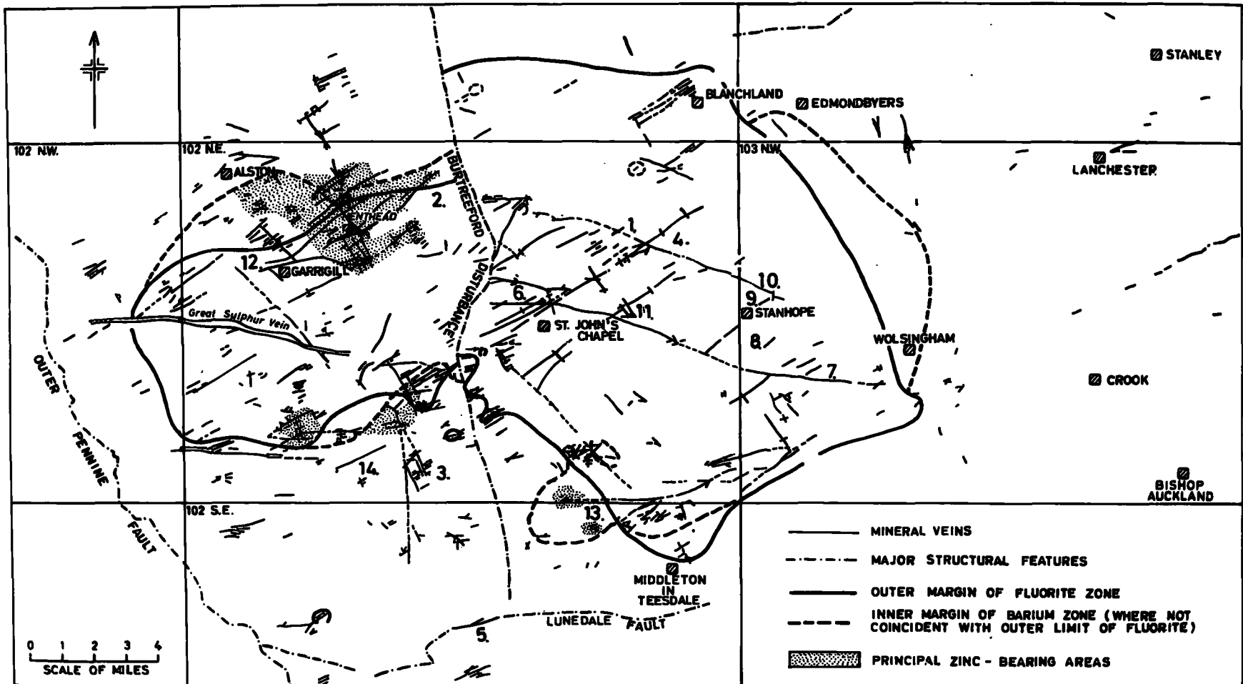
FIG. 2-6. SAMPLING LOCALITIES IN THE NORTHERN PENNINE OREFIELD. (AFTER DUNHAM 1948 PLATE II)
