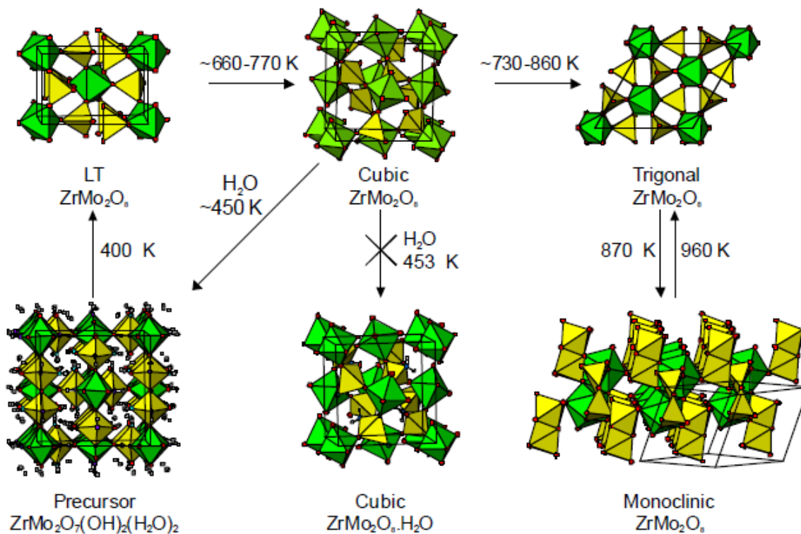
Figure 2.10 Ambient pressure phases of ZrMo_2O_8 . 13
