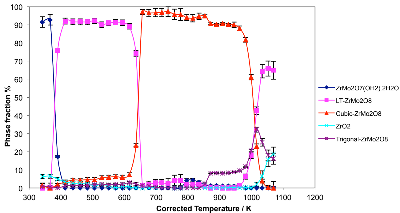
Figure 4.2 Percentage composition as a function of temperature for variable temperature powder X-ray diffraction experiments on perchloric acid derived \text{ZrMo}_2\text{O}_7(\text{OH})_2 \cdot 2\text{H}_2\text{O} (JER 113, experiment code d9_04487).
