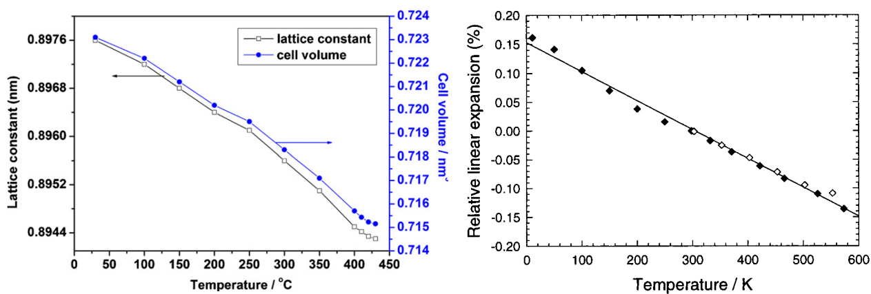
Figure 2.11 Thermal expansion of cubic ZrMo_2O_8 obtained by Lind et al. 24
