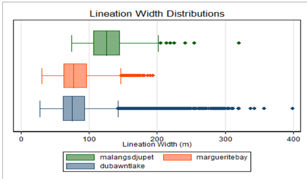
Figure 4.24: Box plots comparing the lination width distributions for the three palaeo-ice stream beds mapped. The boxes enclose the 25 th to the 75 th percentile, with the median represented by the central line, while the whiskers represent the 5 th and 95 th percentiles.
