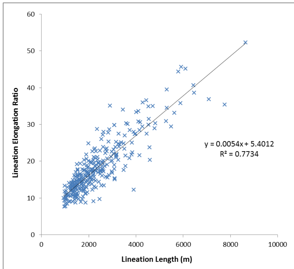
Figure 4.20: Scatter graph for the Malangsdjupet lineation population (n=301), showing the relationships between lineation length and elongation ratio. Again lineation ER is found to be relatively strongly (positively) correlated with lineation length.
