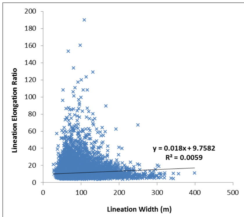
Figure 4.7: Scatter graph for the Dubawnt Lake lineations, showing the relationships between lineation width and elongation ratio. Note that there is apparently no correlation between the two measures.
