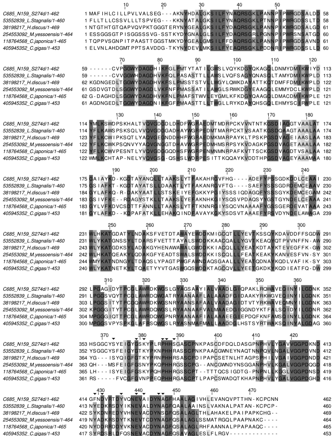
Figure 28 : Alignment of D. reticulatum contig with Molluscan homologues
