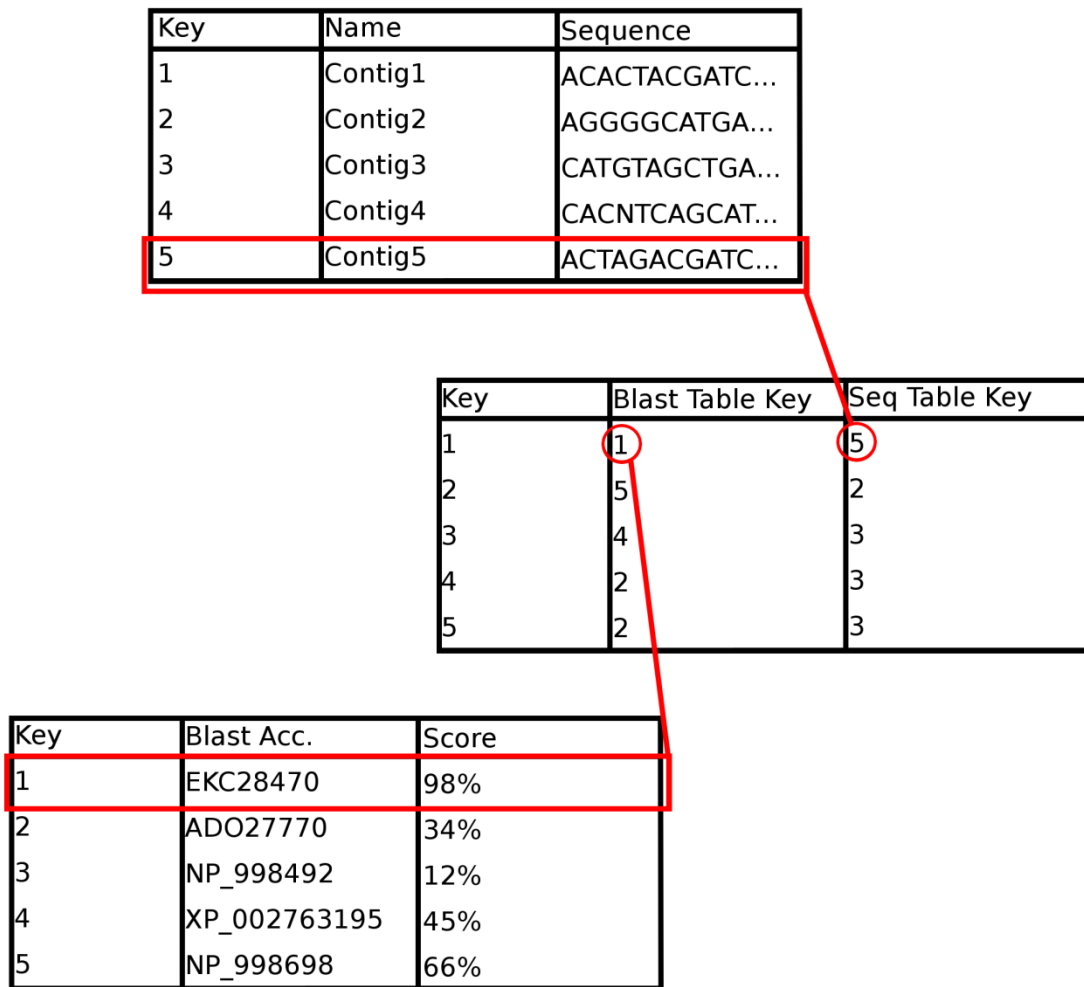
Figure 3 : Simple example of a relational database model
