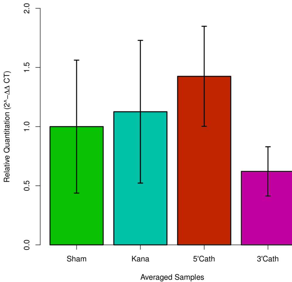
Figure 48 : Average RQ values for RNAi against Cathepsin L
