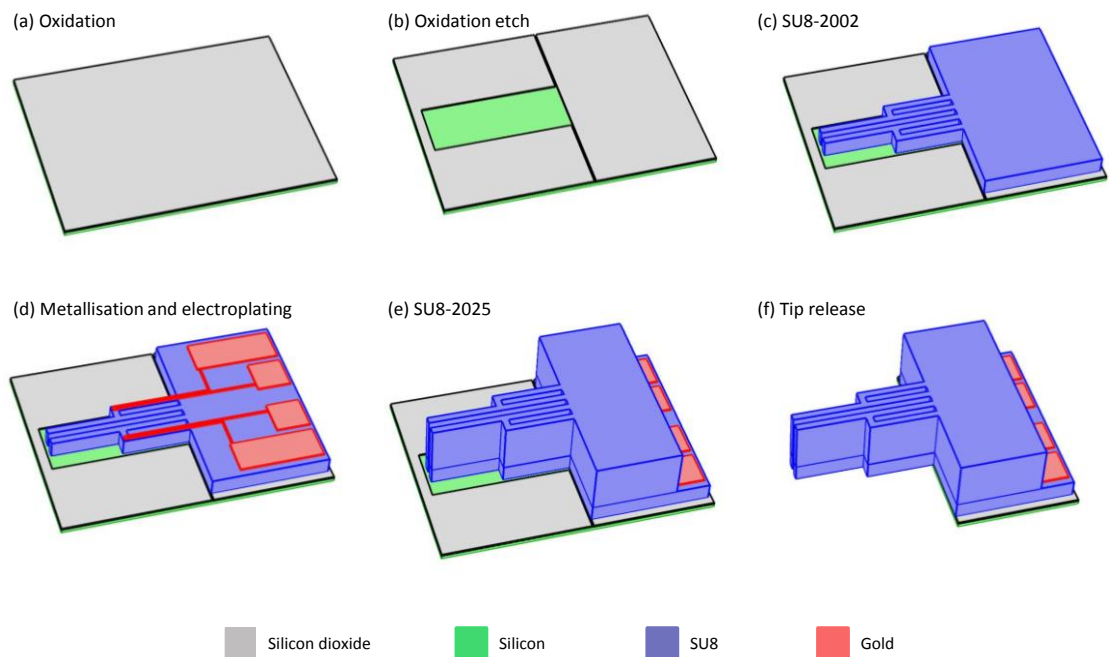
Figure 2.8 – Schematic of the microgripper fabrication (not to scale).
