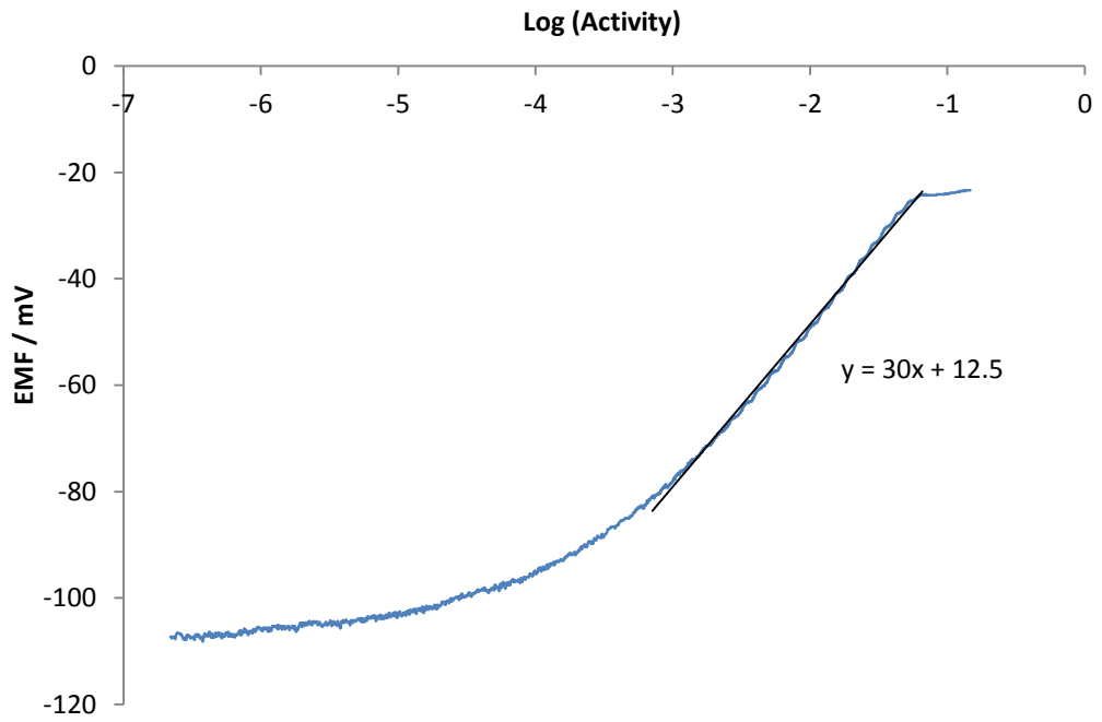
Figure 5.22 – Calibration standard use for the \text{Na}^+ ISE device done in a background of M2 media.
