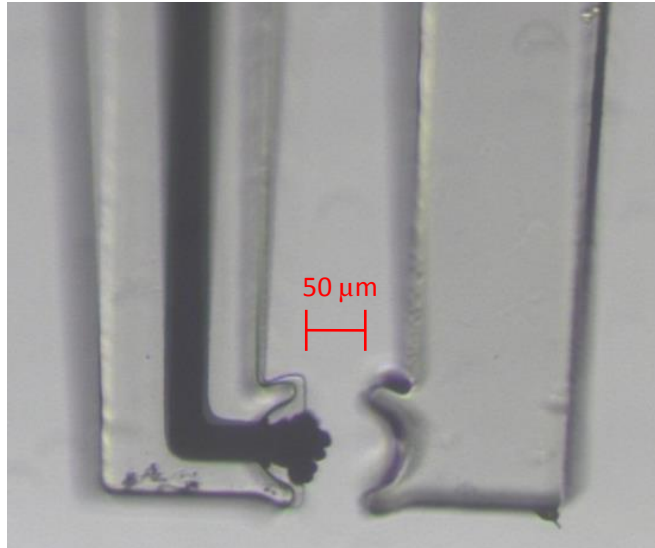
Figure 3.23 – Image of the microgripper tips showing the fibril texture of the PEDOT deposition onto the electrode.
