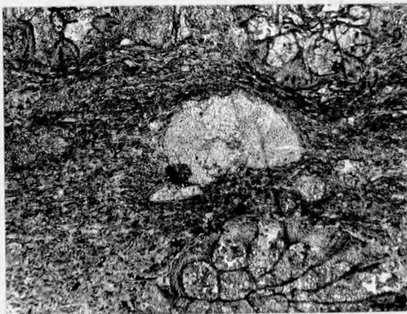
B. Richmond Chert Series, Round Hill, north of Hoove. x 47. Bryozan fragments and part of a crinoid ossicle set in, and distorting the bedding of, a very fine-grained mixture of chemically precipitated carbonate and almost isotropic brown silica.
