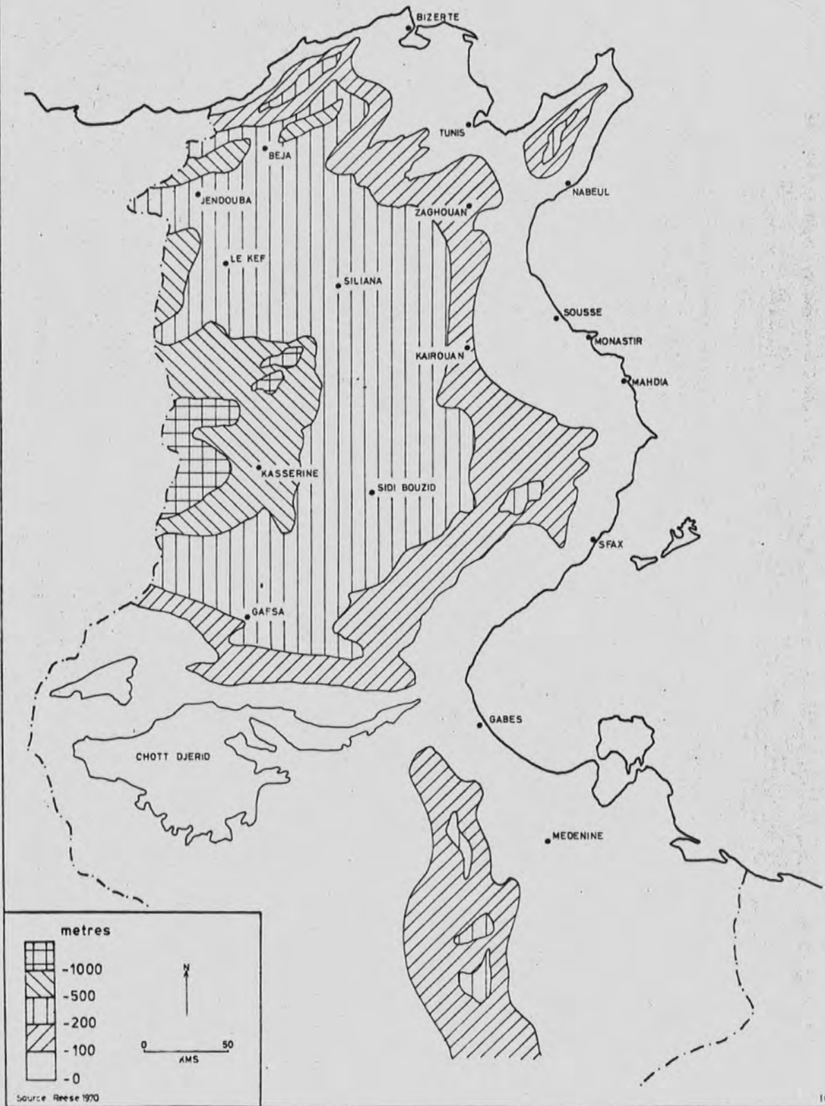
Fig 3.1 GENERALIZED RELIEF
