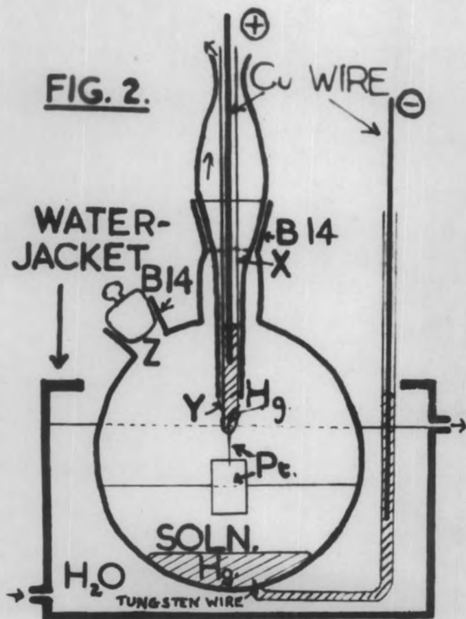
MERCURY-CATHODE ELECTROLYSIS CELL.
