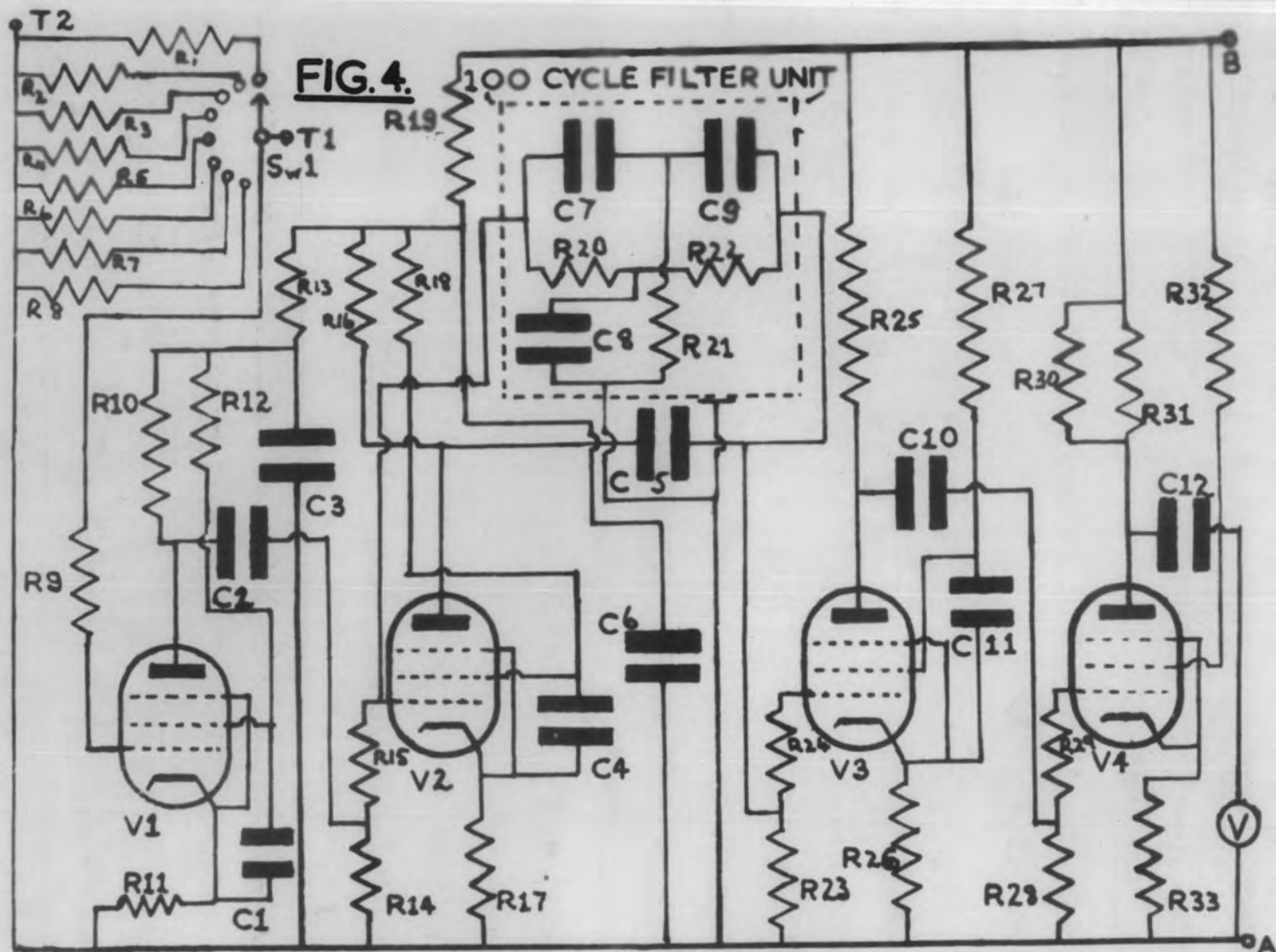
FLUORIMETER AMPLIFIER.
