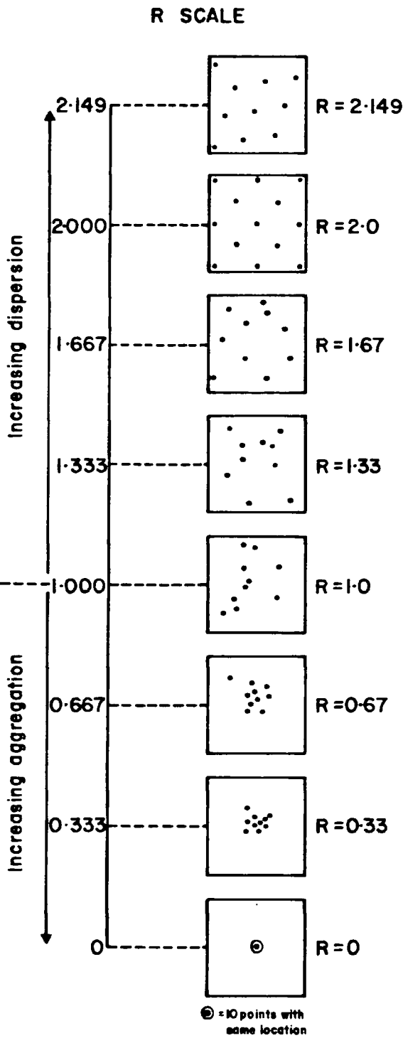
Figure 3.1 NEAREST NEIGHBOUR ANALYSIS
