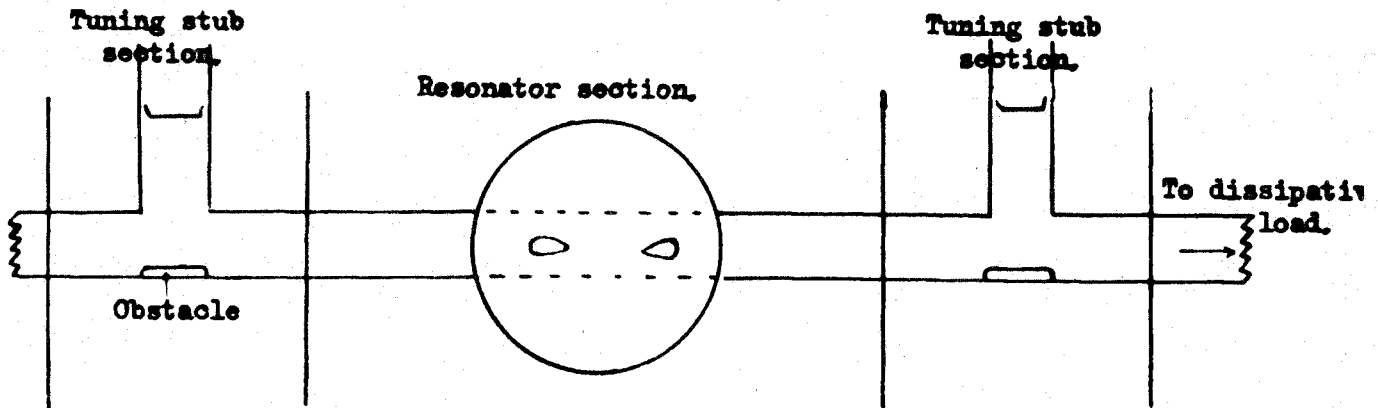
Fig. 31 , Arrangement of U.H.F. apparatus.
