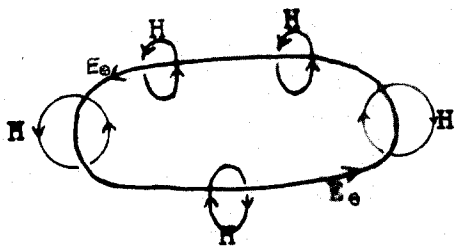
Fig. 6 . Field configuration, H_{01} mode.
