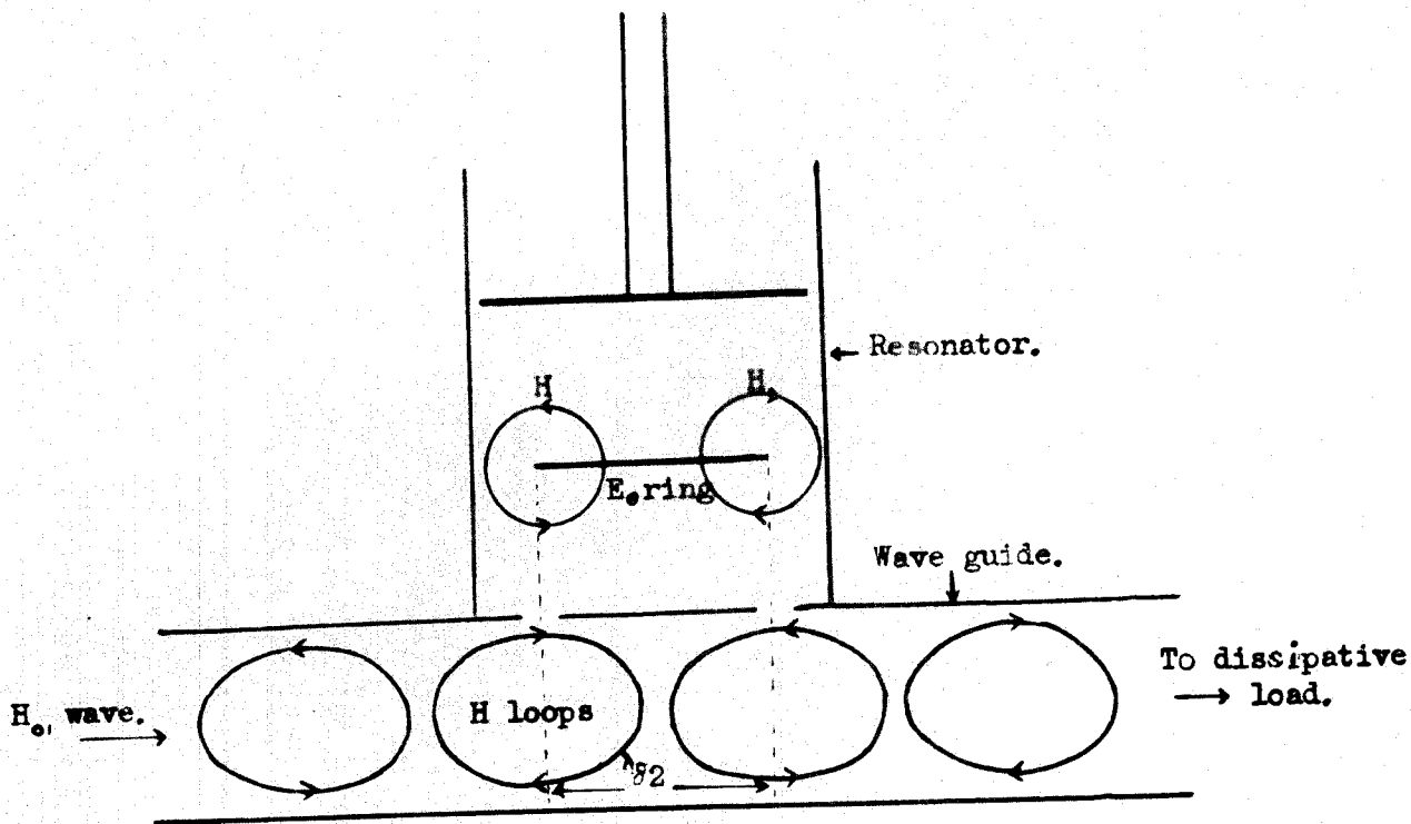
Fig. 8 . Magnetic coupling to resonator.
