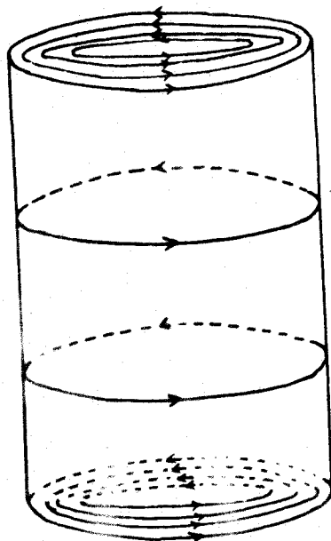
Fig. 7 . Current flow, H_{01} mode.
