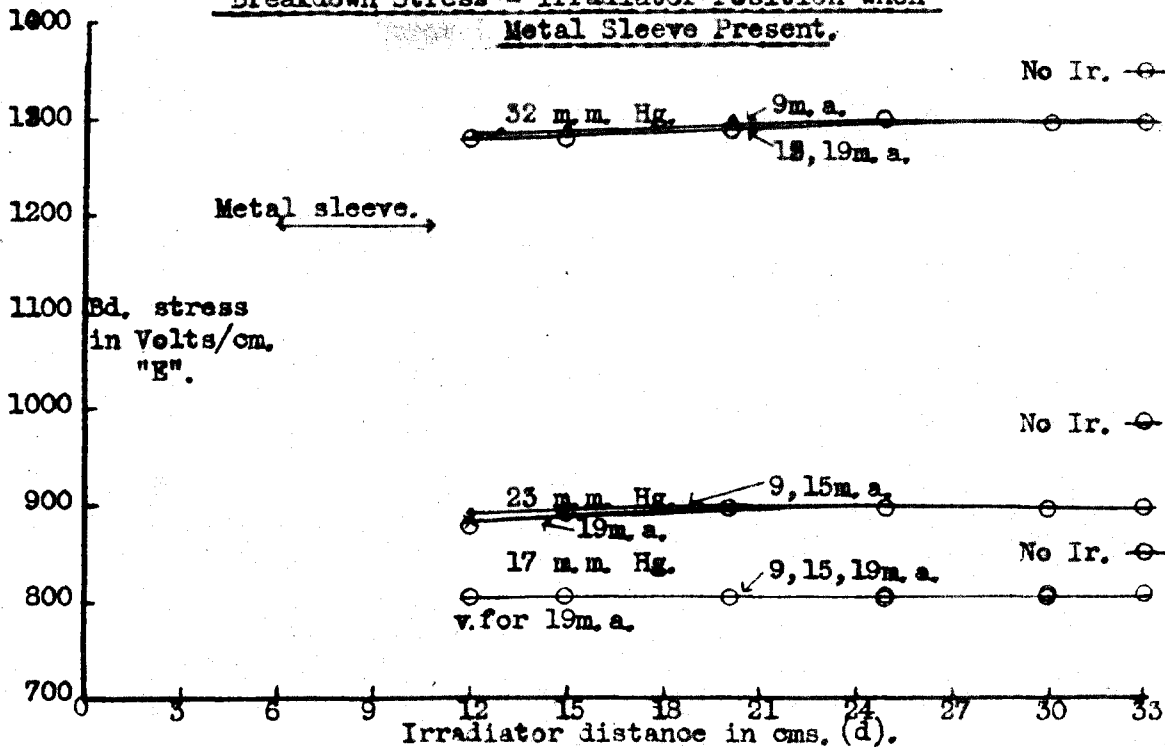
Graph 20 Breakdown Stress - Metal Sleeve Position with Irradiator Fixed.
