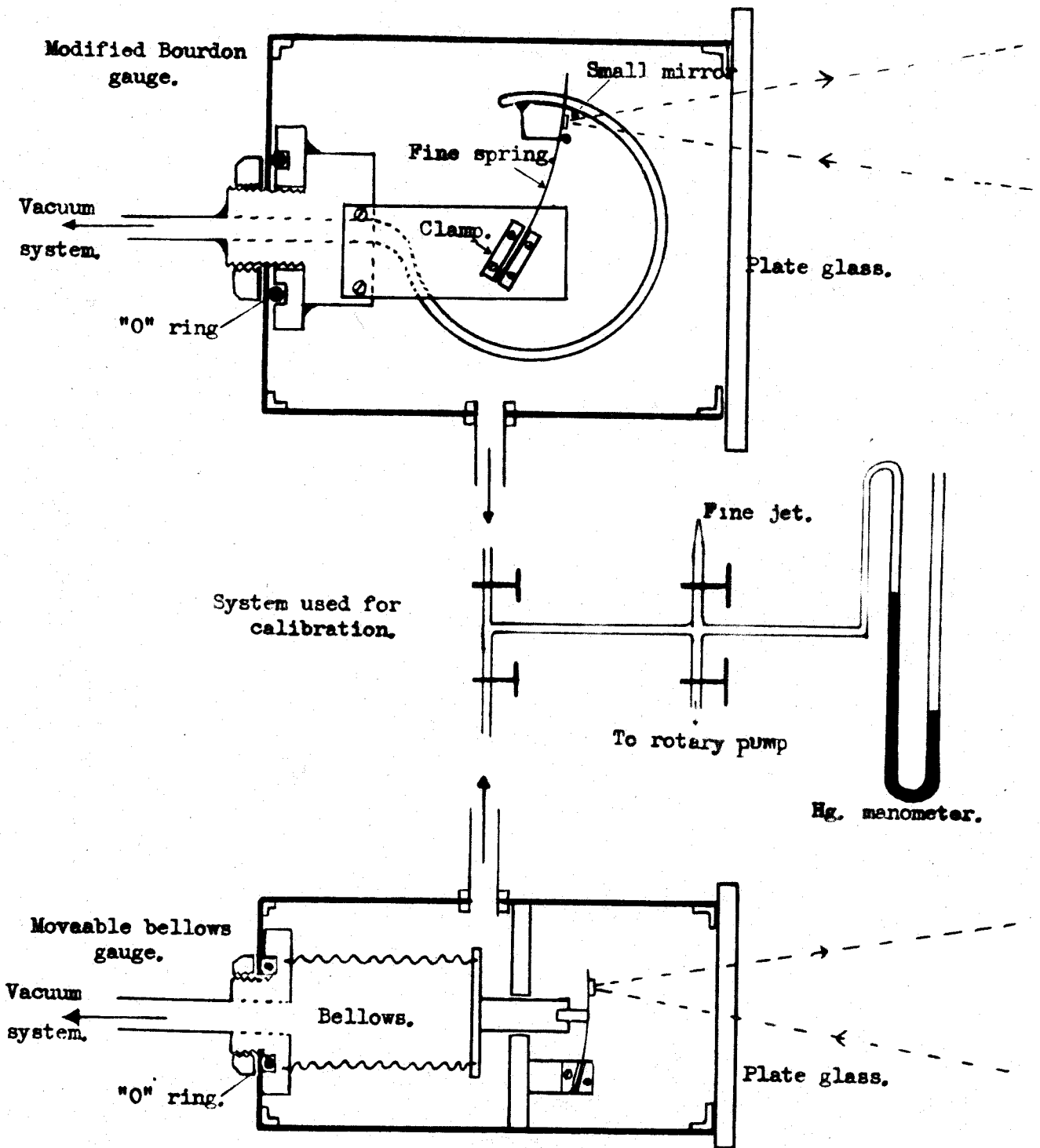
Fig. 42. Pressure gauges.
