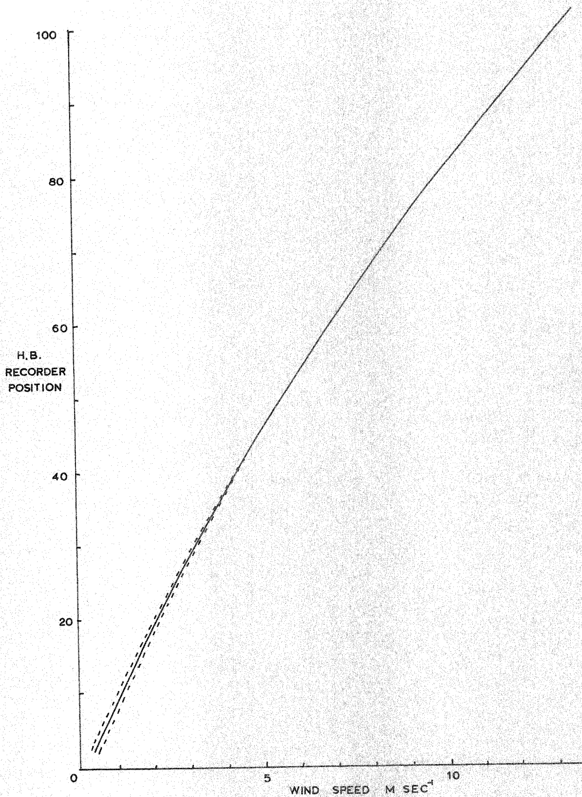
A TYPICAL ANEMOMETER CALIBRATION FIGURE 18.
