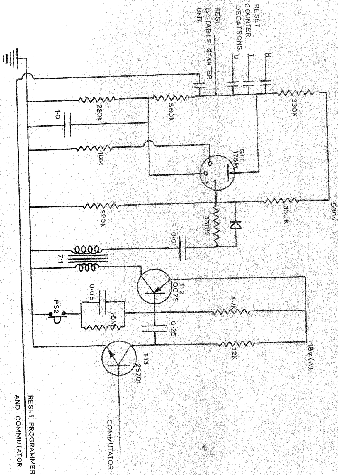
RESET UNIT FIGURE 31.
