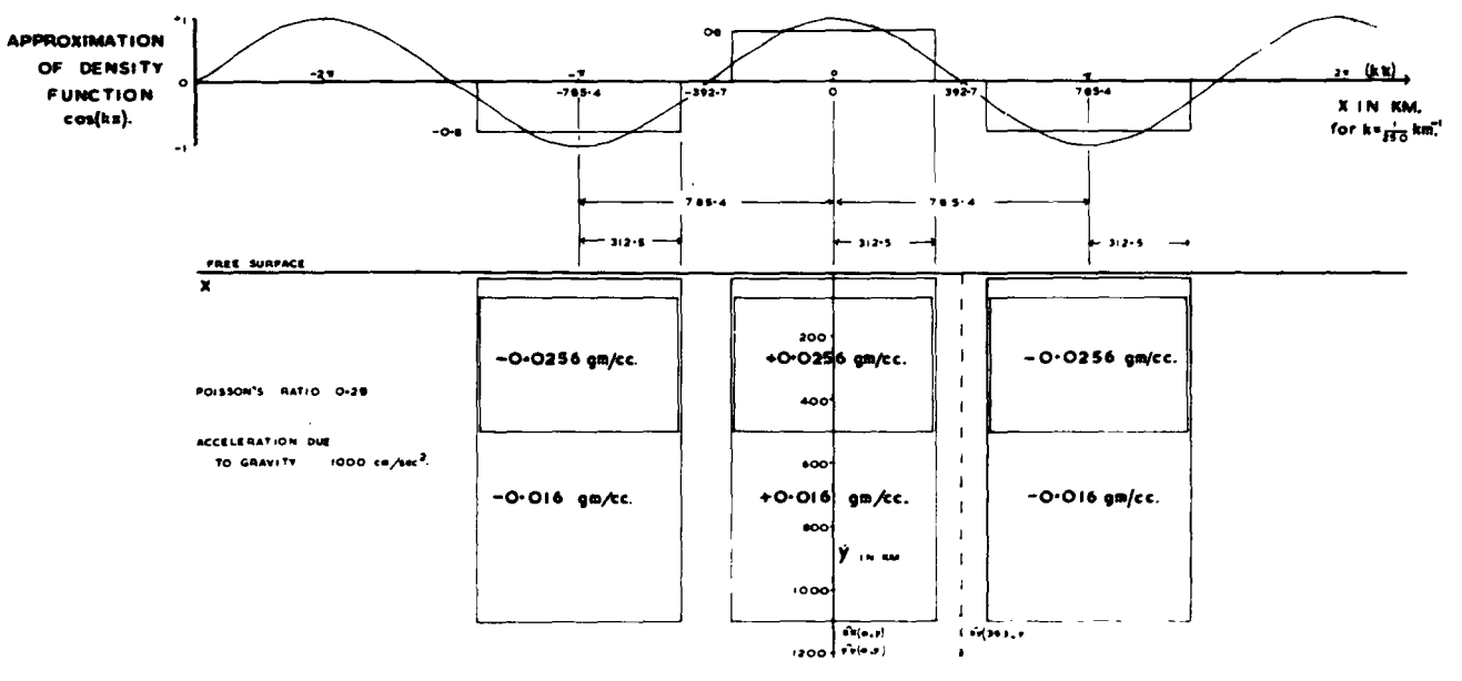
THE SIMULATION OF DURNEY'S NUMERICAL RESULTS FOR k EQUALS \frac{1}{350} \text{ km}^{-1}
