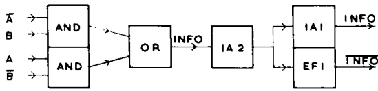
TWO BIT MODULE
