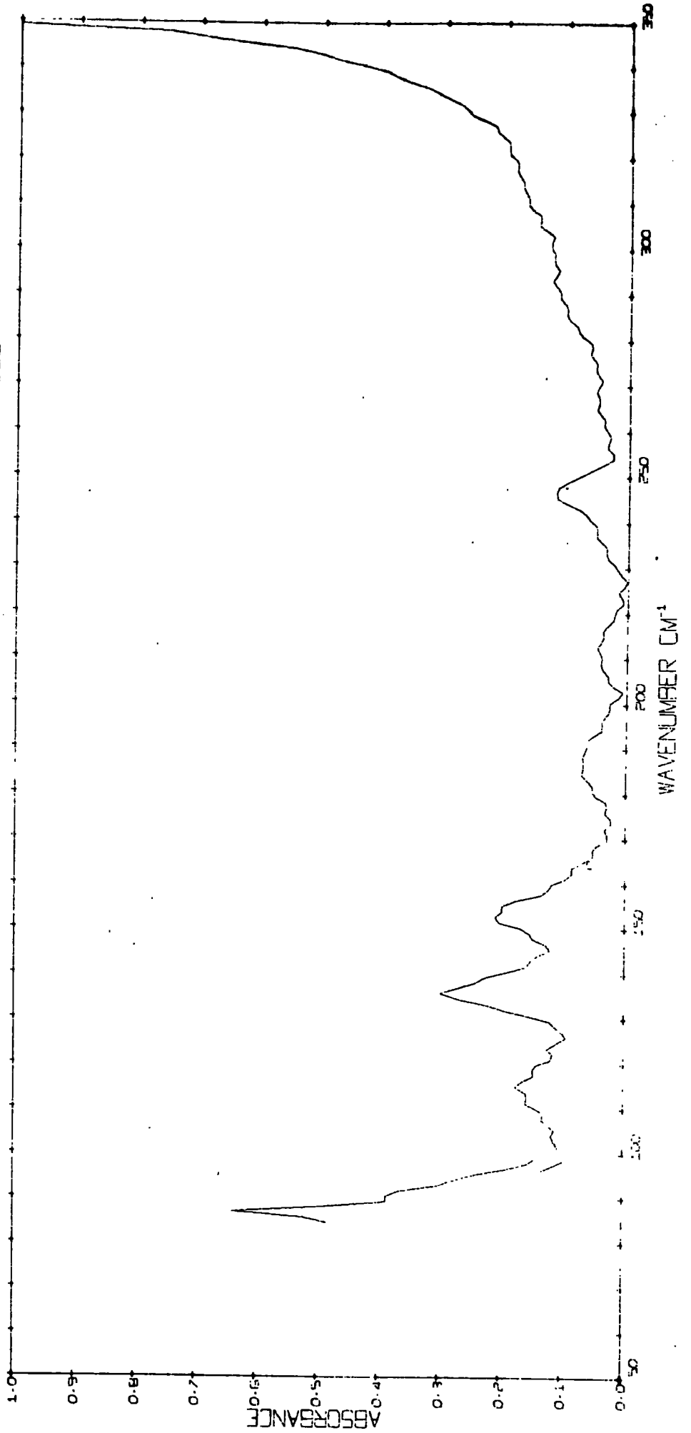
Spectrum Number 8.19
