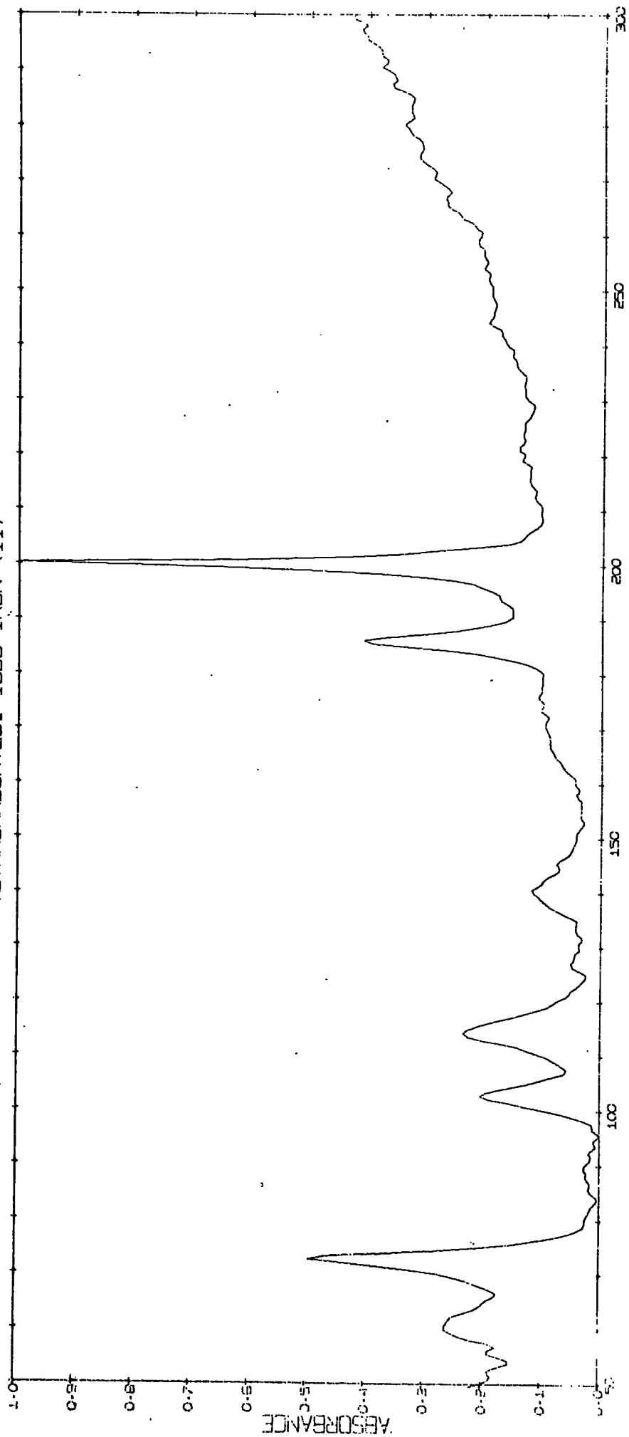
Spectrum 8.9
