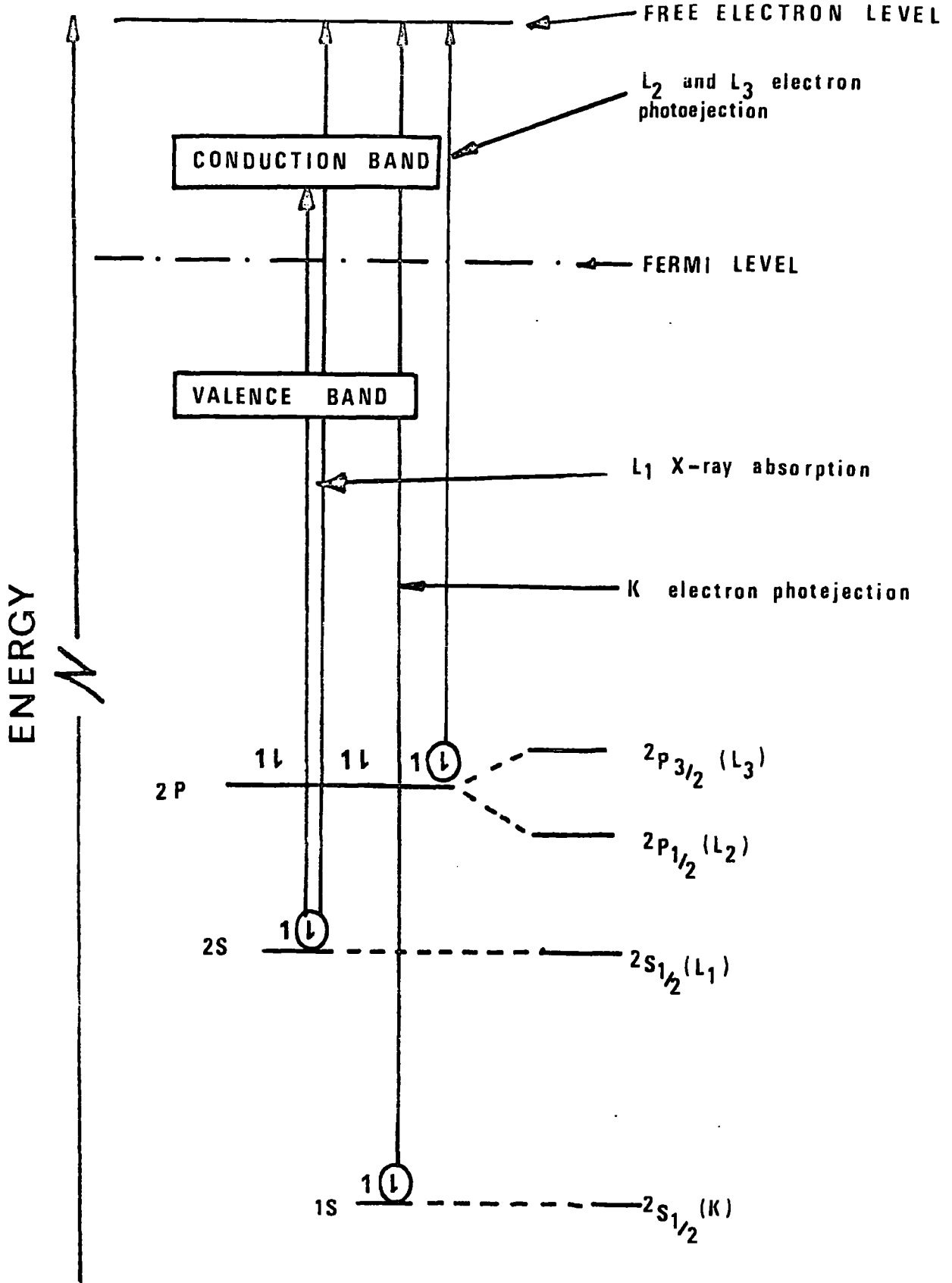
Fig. 7.2 Photo ionisation of an electrical insulator.
