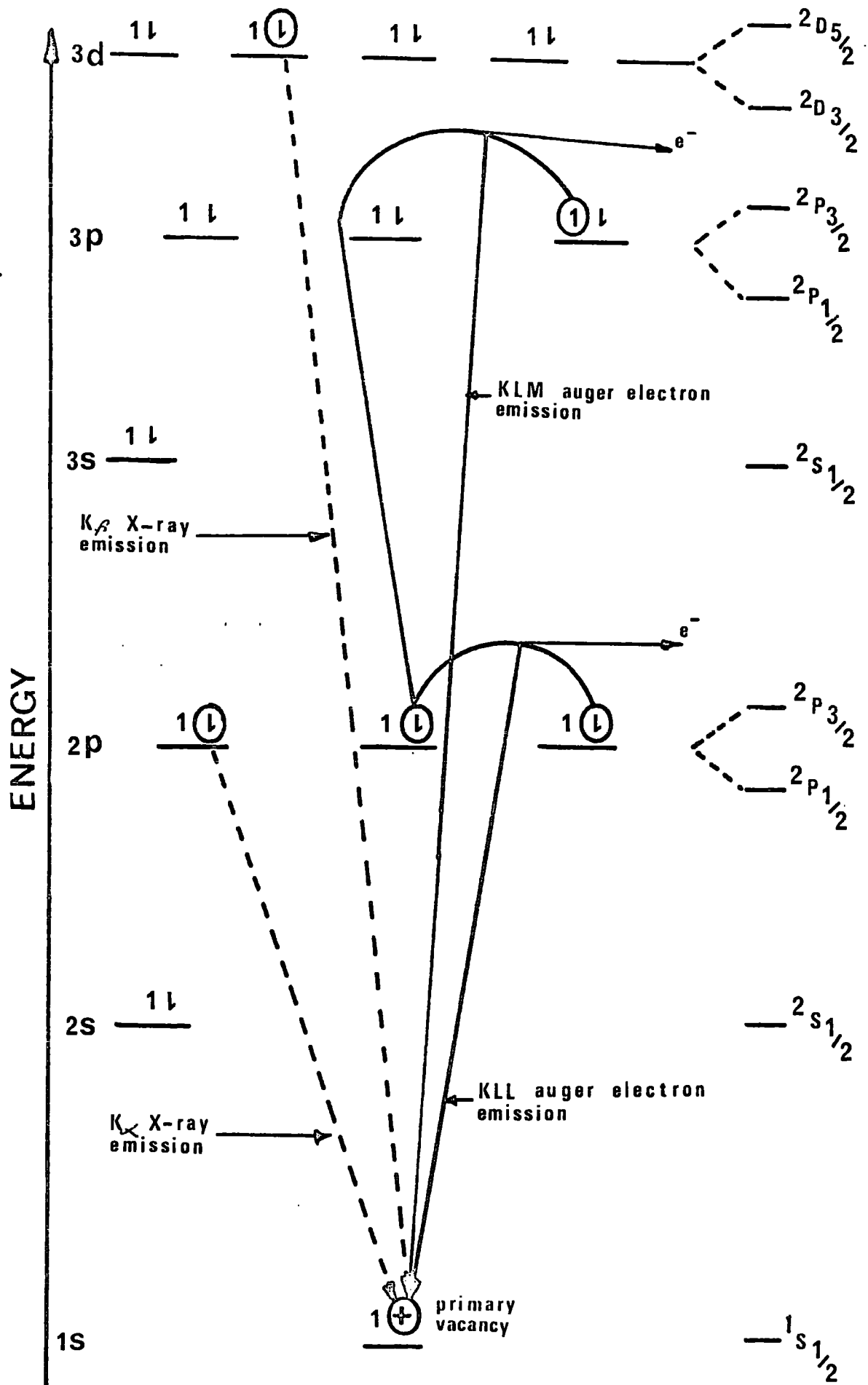
Fig. 7.3 Diagram for electron relaxation.
