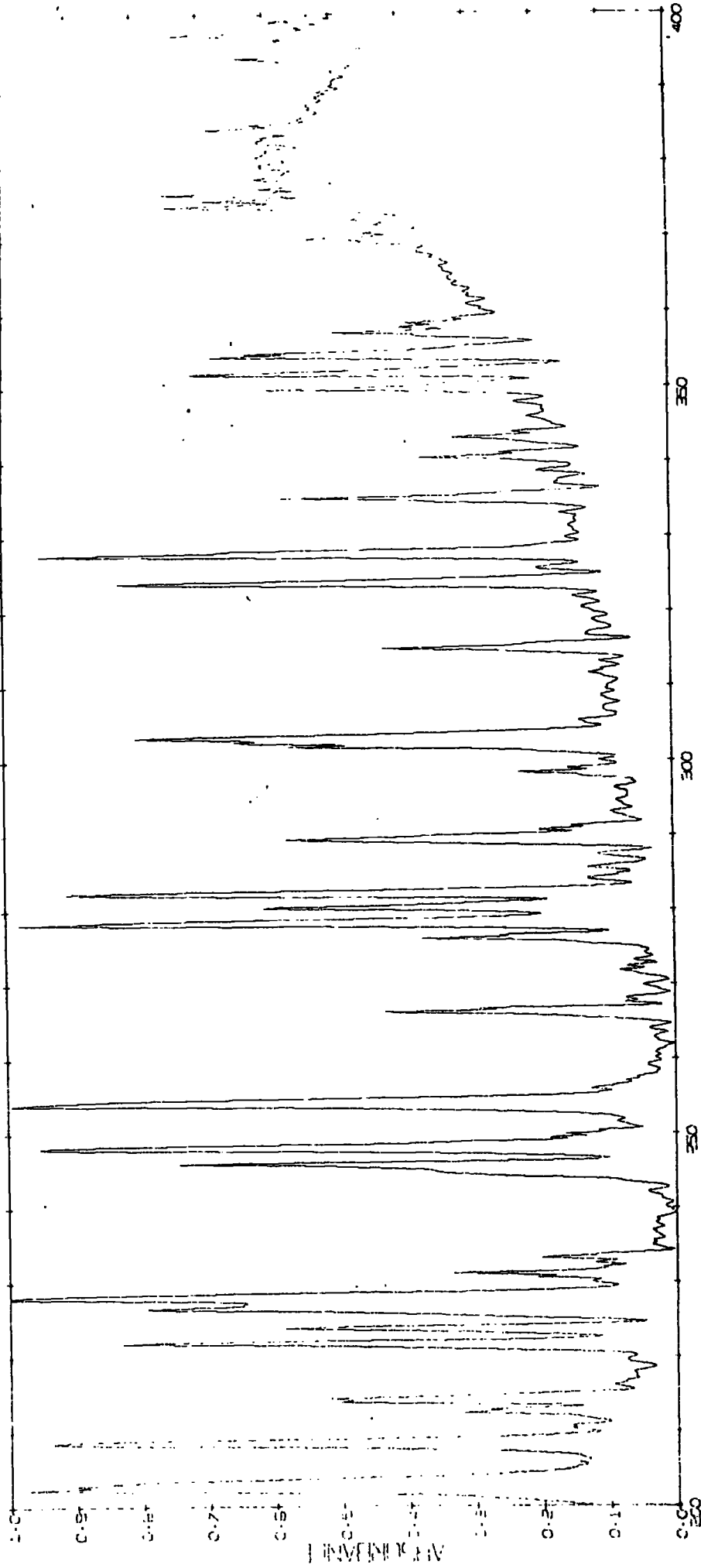
Spectrum 8.6B
