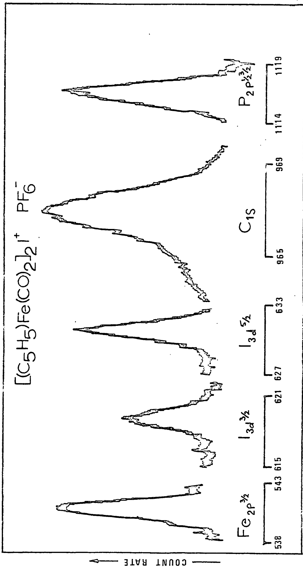
Spectrum number 7.6
