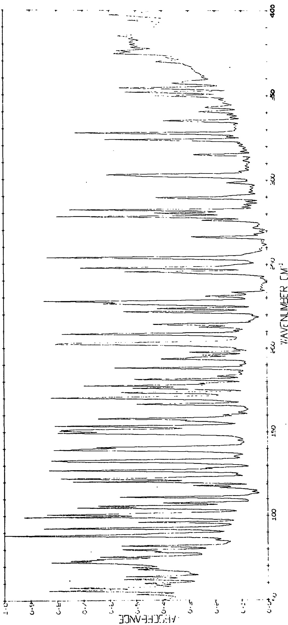
Spectrum 8.5
