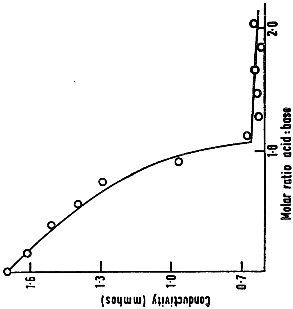
The conductimetric titration of \text{BCl}_3 against [(\pi\text{-C}_5\text{H}_5)\text{Fe}(\text{CO})_2]_2 in liquid hydrogen chloride
