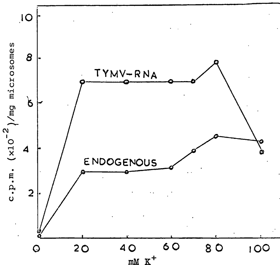
Fig.67. TRANSFER SYSTEM: Effect of K^+ on TYMV-RNA-directed incorporation from ^{14}C AA-V. faba tRNA.
