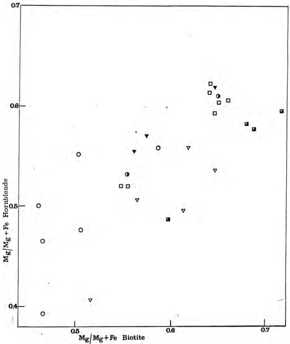
The distribution of magnesium between biotite and hornblende in ○ pyriboleites, ▼ biotite-hornblende-clinopyroxene gneisses, □ amphibolites with magnetite and ilmenite, ▽ amphibolites with ilmenite, ■ amphibolites with magnetite and sphene and ● amphibolites with no oxide phases.
