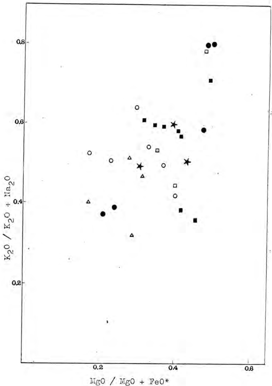
Variation of K_2O to (K_2O + Na_2O) ratio against MgO to (MgO + \text{total Fe as FeO}^*) ratio in intermediate hornblende-bearing rocks of Lervig and Lande gneiss ○, Kvinesdal gneiss △, Fjotland granite □, and Sirdalsvatn Series ■, together with biotite-clinopyroxene gneisses of Fjotland granite ★, and Sirdalsvatn Series ●.
