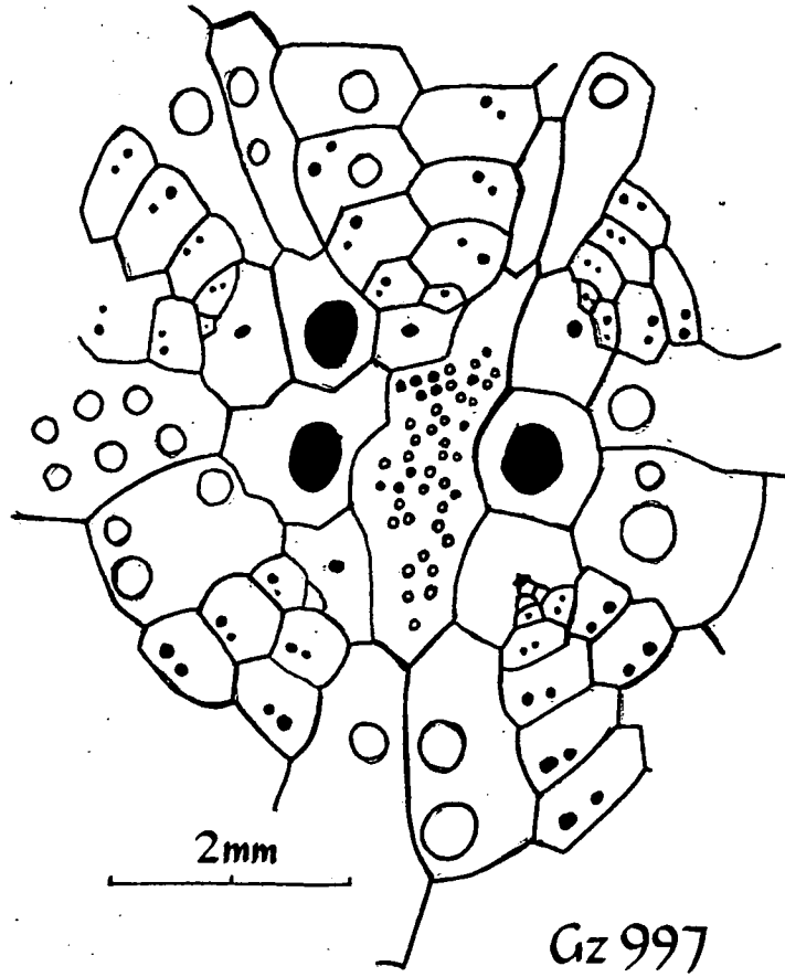
APICAL DISC OF Pericosmus latus
