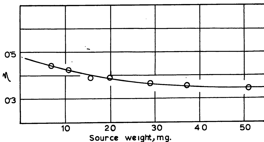
Fig.12. Counting-efficiency curve for ^{99}\text{Mo} as a function of source weight.
