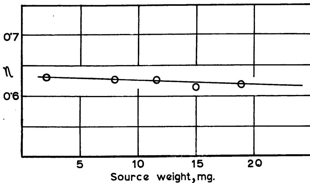
Fig.13. Counting efficiency curve for 46h \text{Sb}^{129} as function of source weight.
