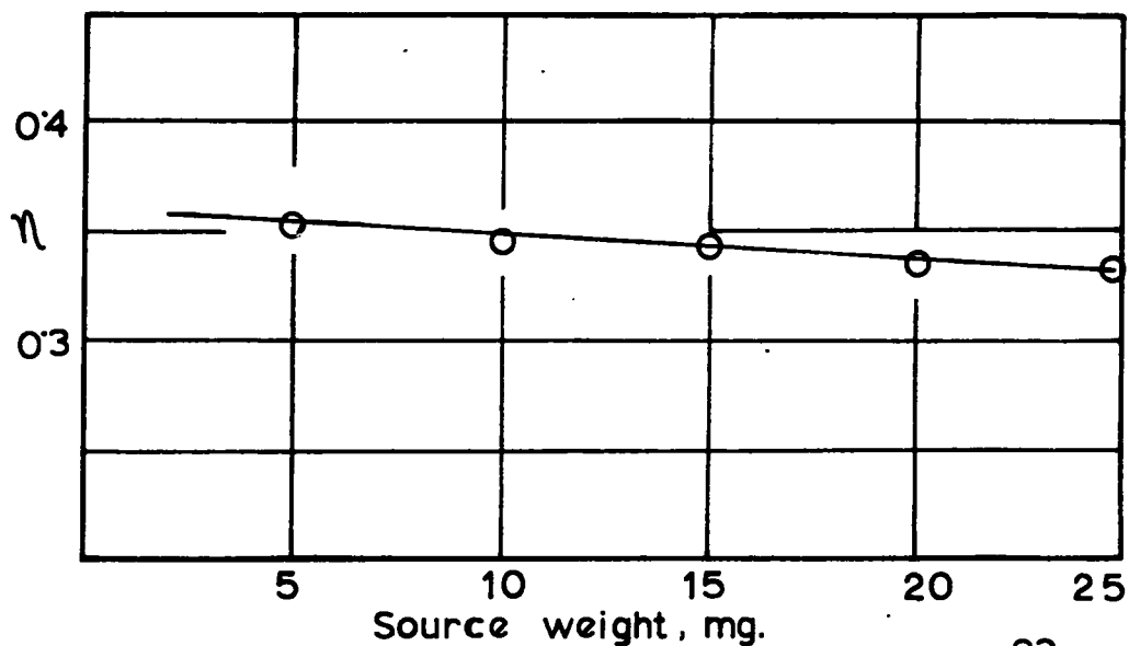
Fig.10. Counting-efficiency curve for ^{83}\text{Br} as function of source weight
