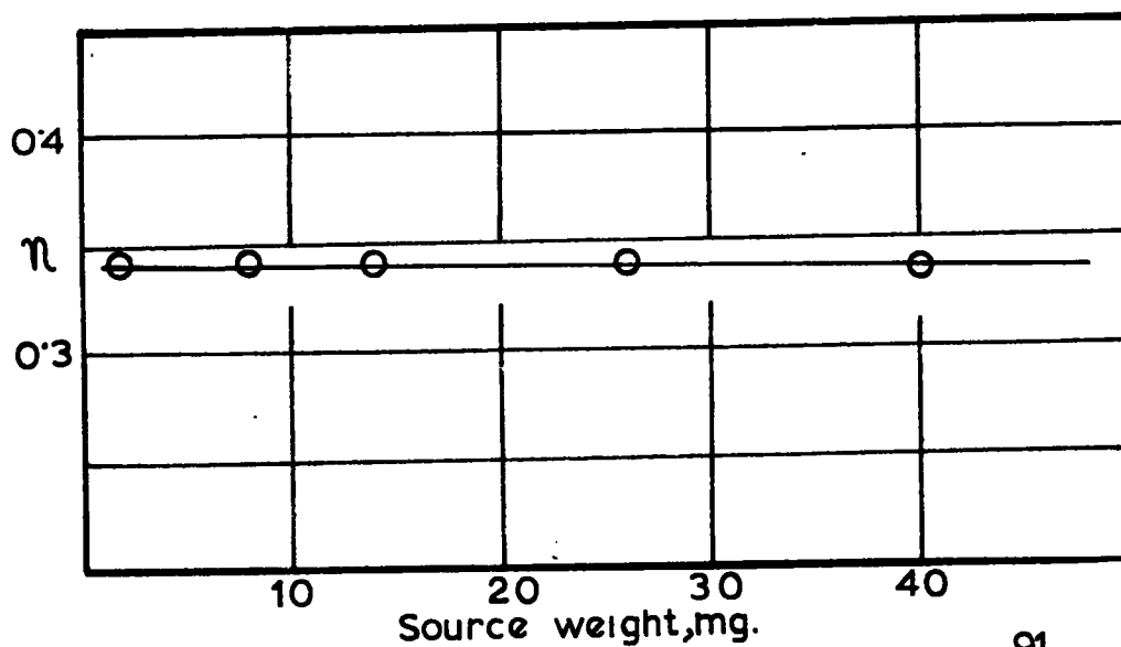
Fig.18. Counting efficiency curve for ^{91}\text{Y} as function of source weight
