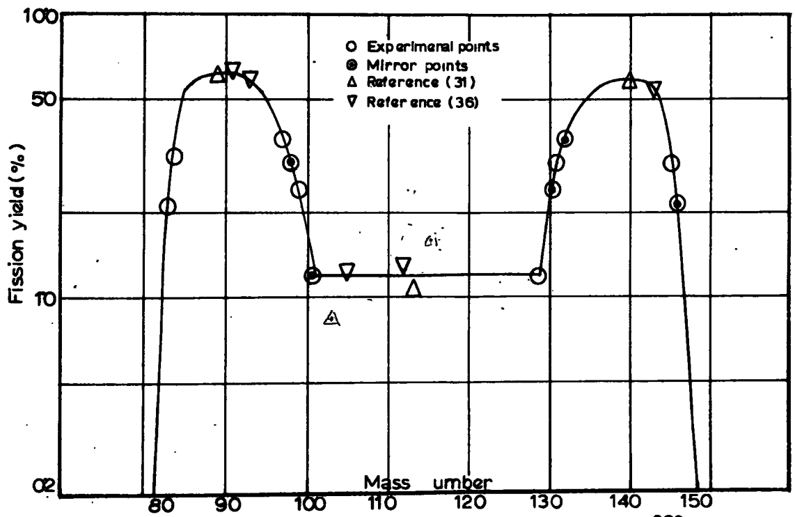
Fig. 24. Mass yield Curve for 14-Mev Neutron Fission of \text{Th}^{232}
