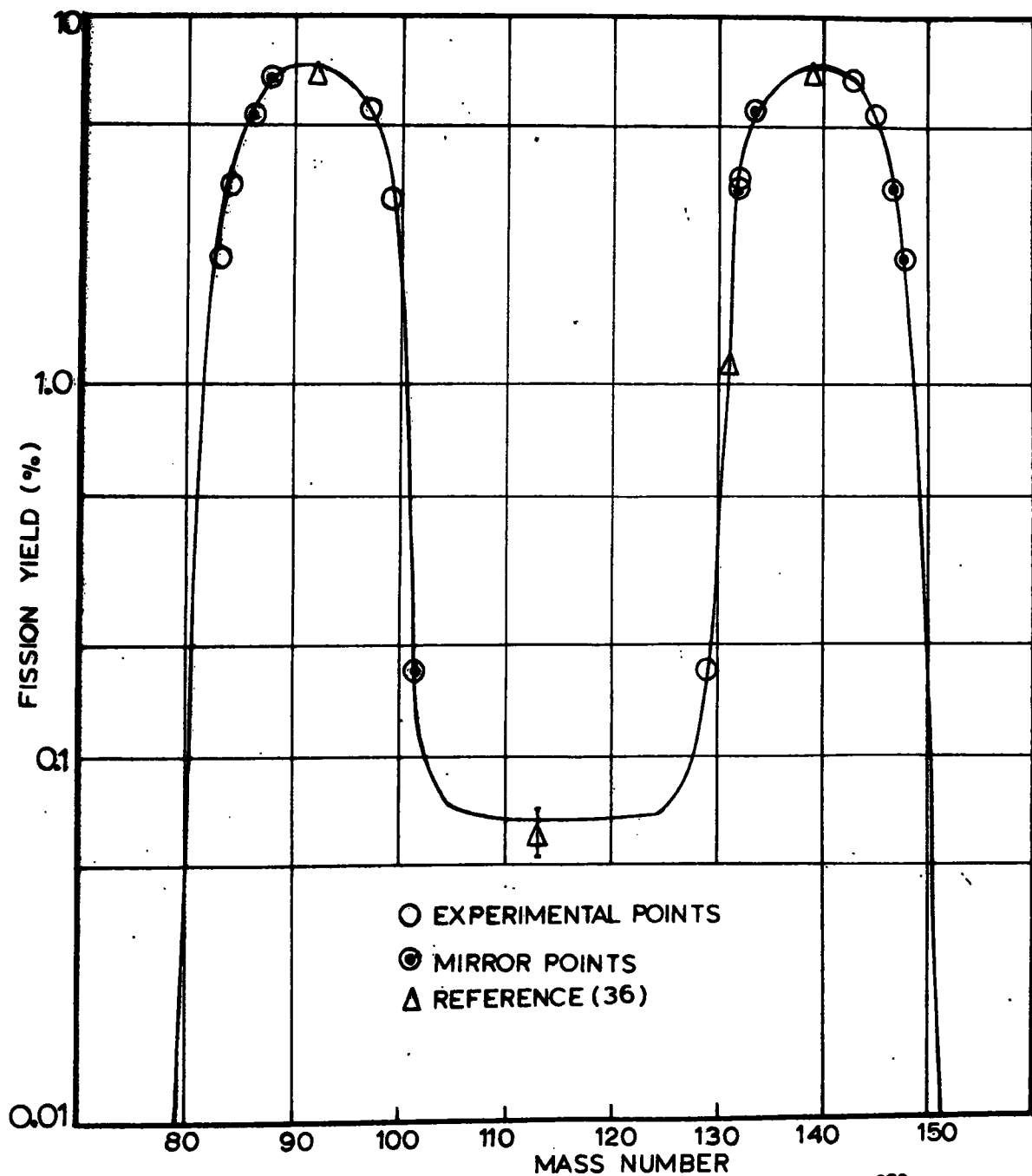
Fig.23. Mass-yield curve for 3-Mev. neutron fission of \text{Th}^{232}
