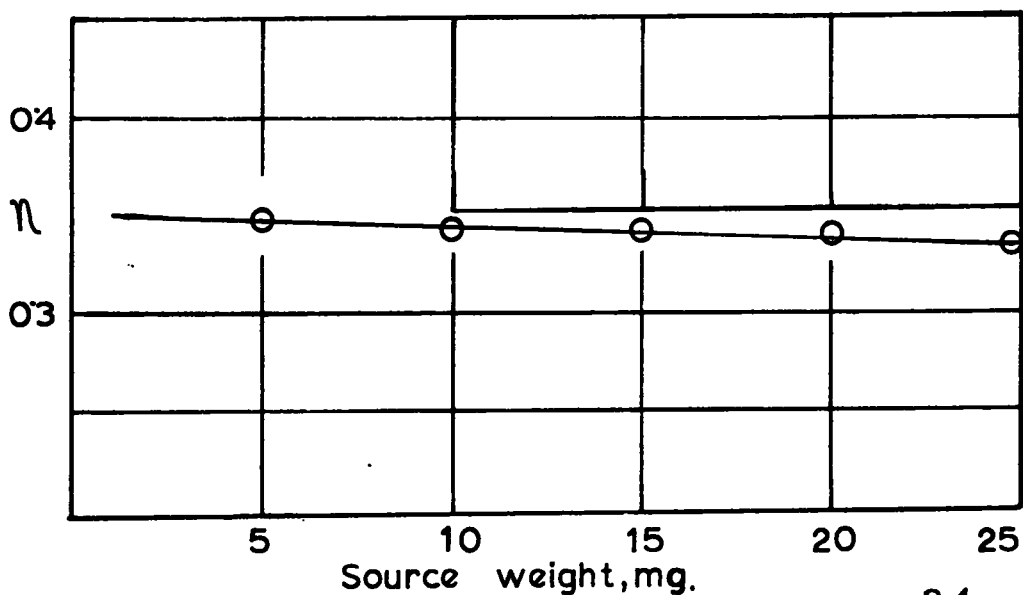
Fig.11. Counting-efficiency curve for ^{84}\text{Br} as function of source weight
