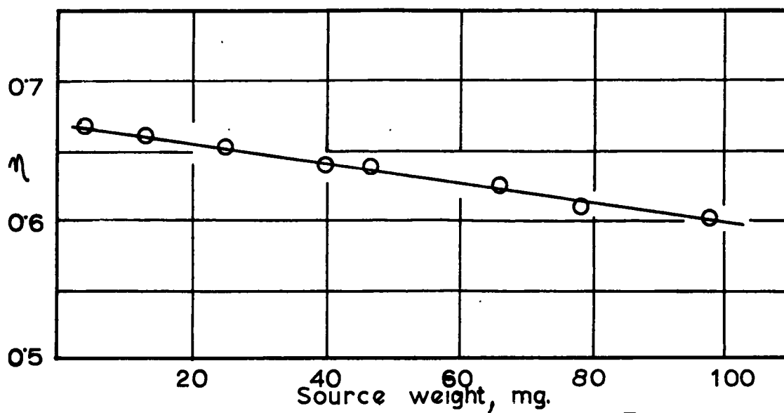
Fig.9. Counting-efficiency curve for ^{97}\text{Zr} as a function of source weight.
