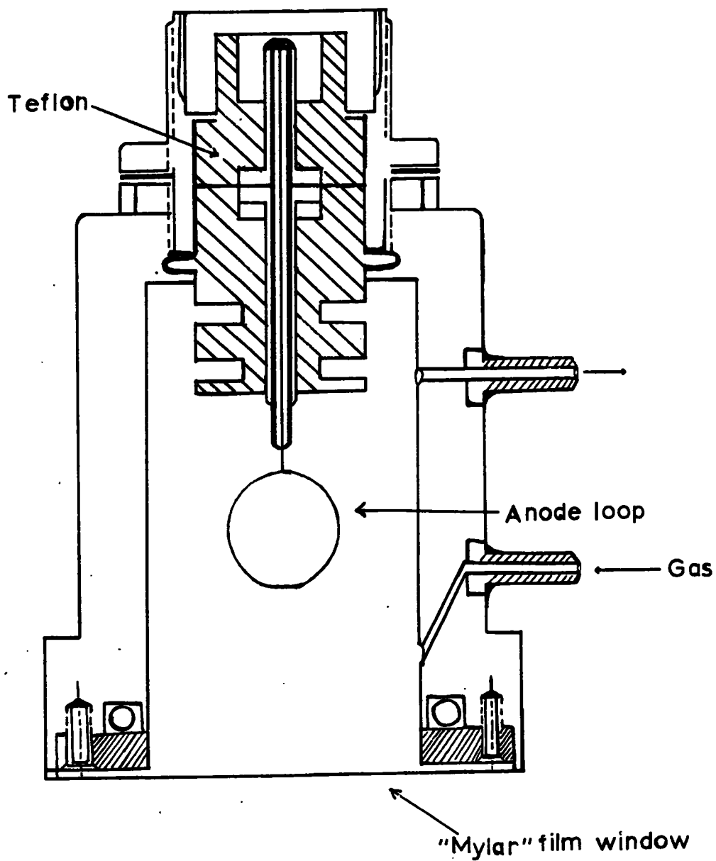
Fig. 4— End-window Gas-flow \beta -proportional Counter
