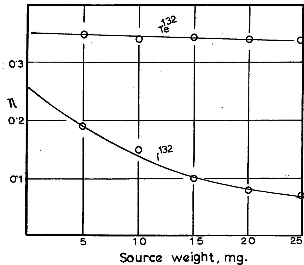
Fig.19. Counting efficiency curves for 77h ^{132}\text{Te} and 2.3h ^{132}\text{I} as function of source weight.
