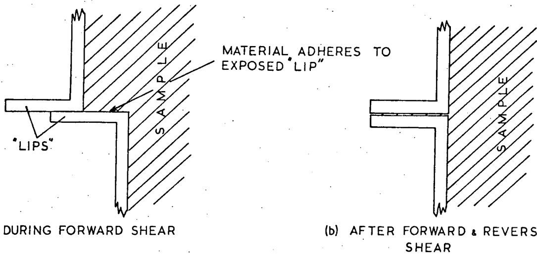
Fig. III. 6. Wedging apart of the shear-box halves by displaced material.
