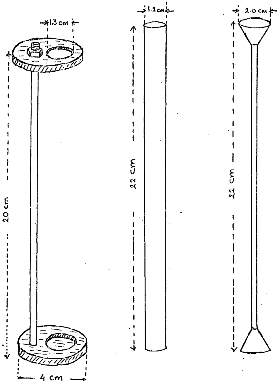
Figure 4.5 The sample holder and the wave guides used in acoustic emission experiments.
