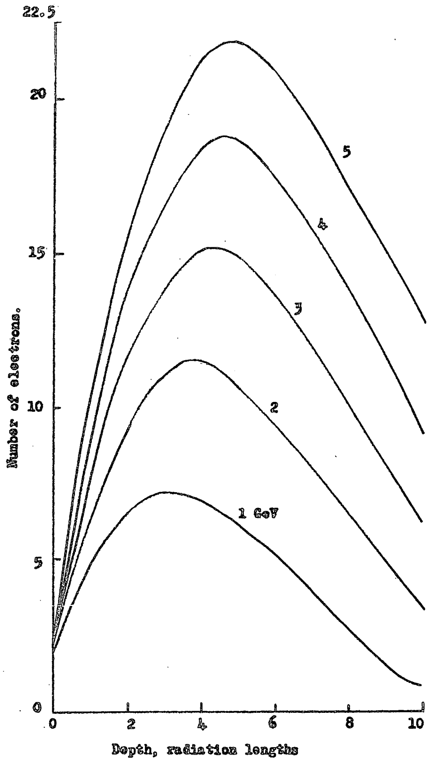
Figure 5.2 Standard shower curves obtained from the experimental curves of Baekenstoss et al. (1963a)
