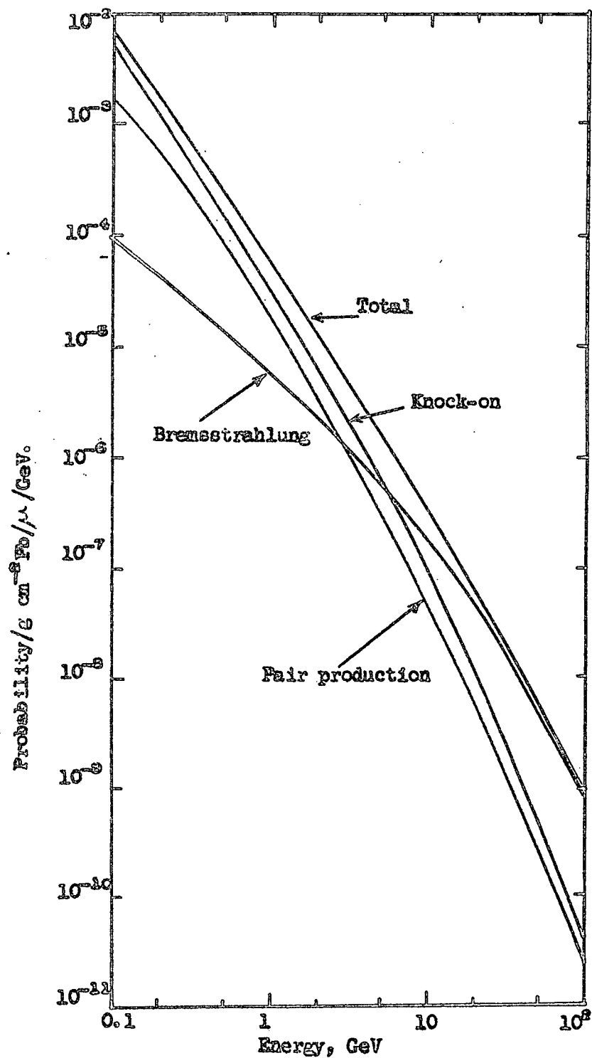
Differential Probabilities for the Electromagnetic Interactions of Muons in Lead at 60m.w.e.
