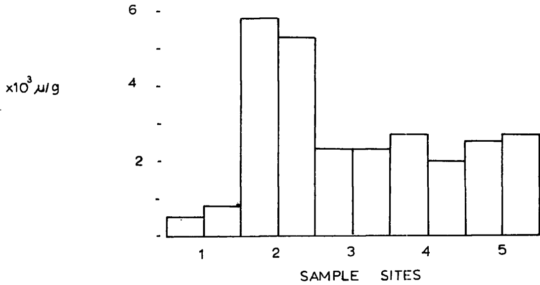
FIGURE 53 LEAD CONCENTRATION IN SKINNINGROVE BECK
