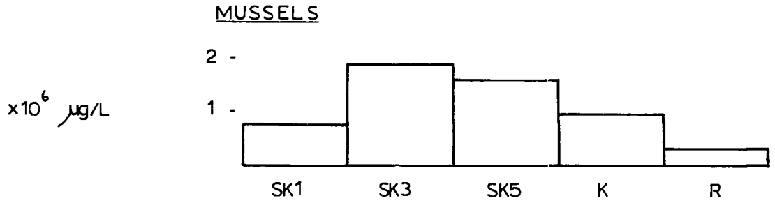
FIGURE 48 . IRON CONCENTRATIONS IN SELECTED MARINE ORGANISMS AT THE SAMPLE SITES.
