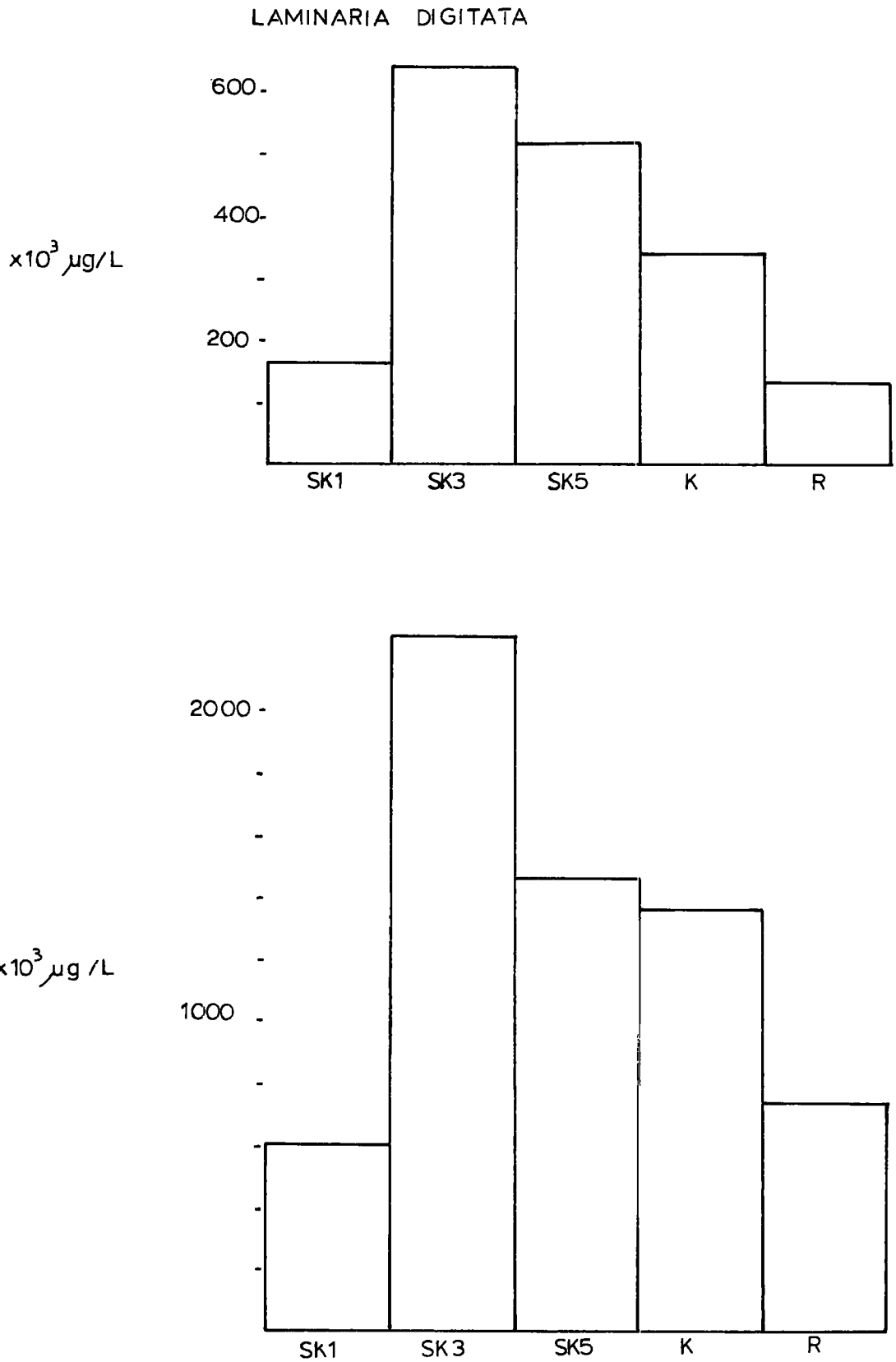
FIGURE 47 . IRON CONCENTRATIONS IN SELECTED SEAWEEDS AT THE SAMPLE SITES.
