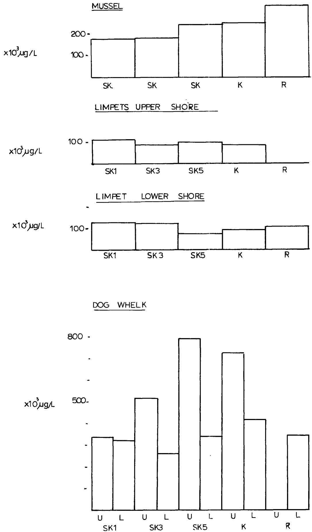
FIGURE 29 . ZINC CONCENTRATIONS IN SELECTED MARINE ORGANISMS AT THE SAMPLE SITES.
