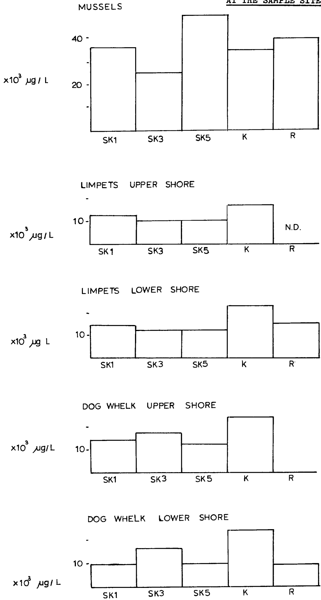
FIGURE 58. LEAD CONCENTRATIONS IN SELECTED MARINE ORGANISMS AT THE SAMPLE SITES.
