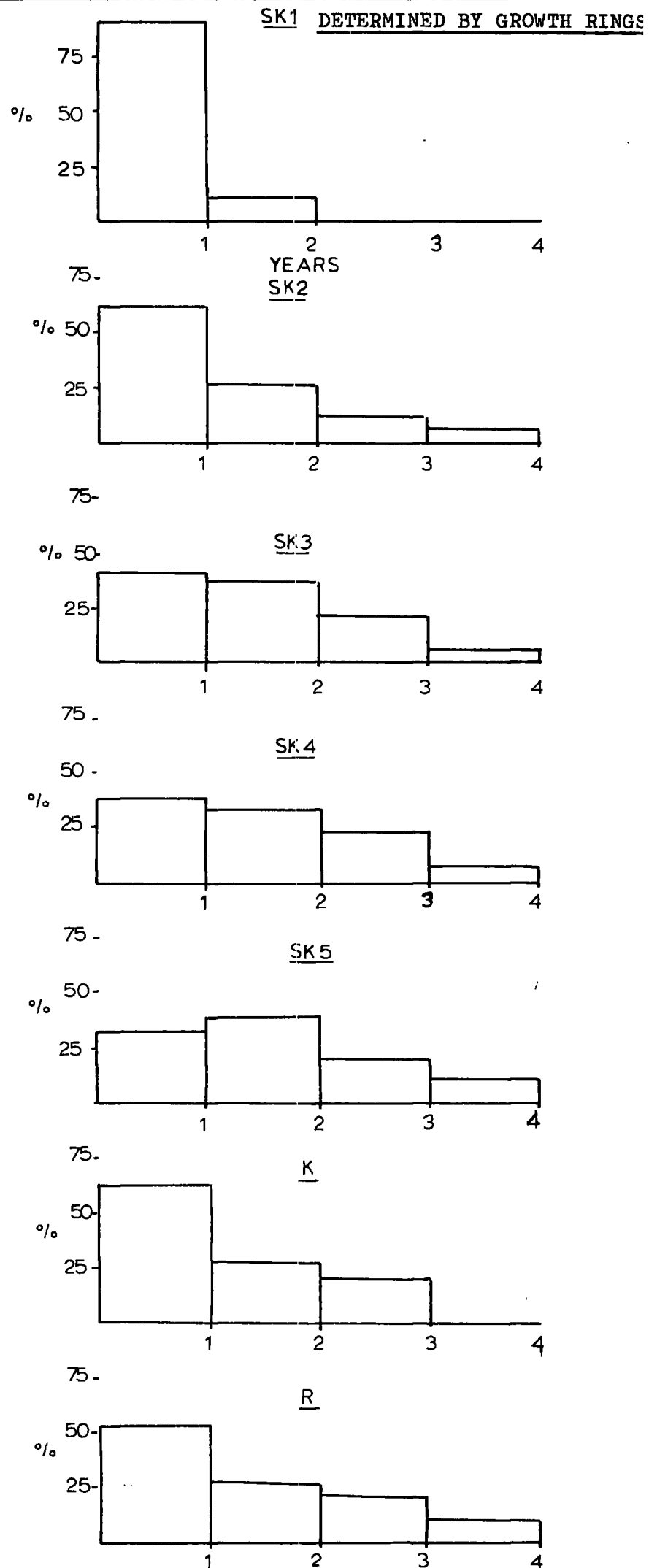
FIGURE 8. AGE STRUCTURE OF LAMINARIA DIGITATA POPULATIONS AS
