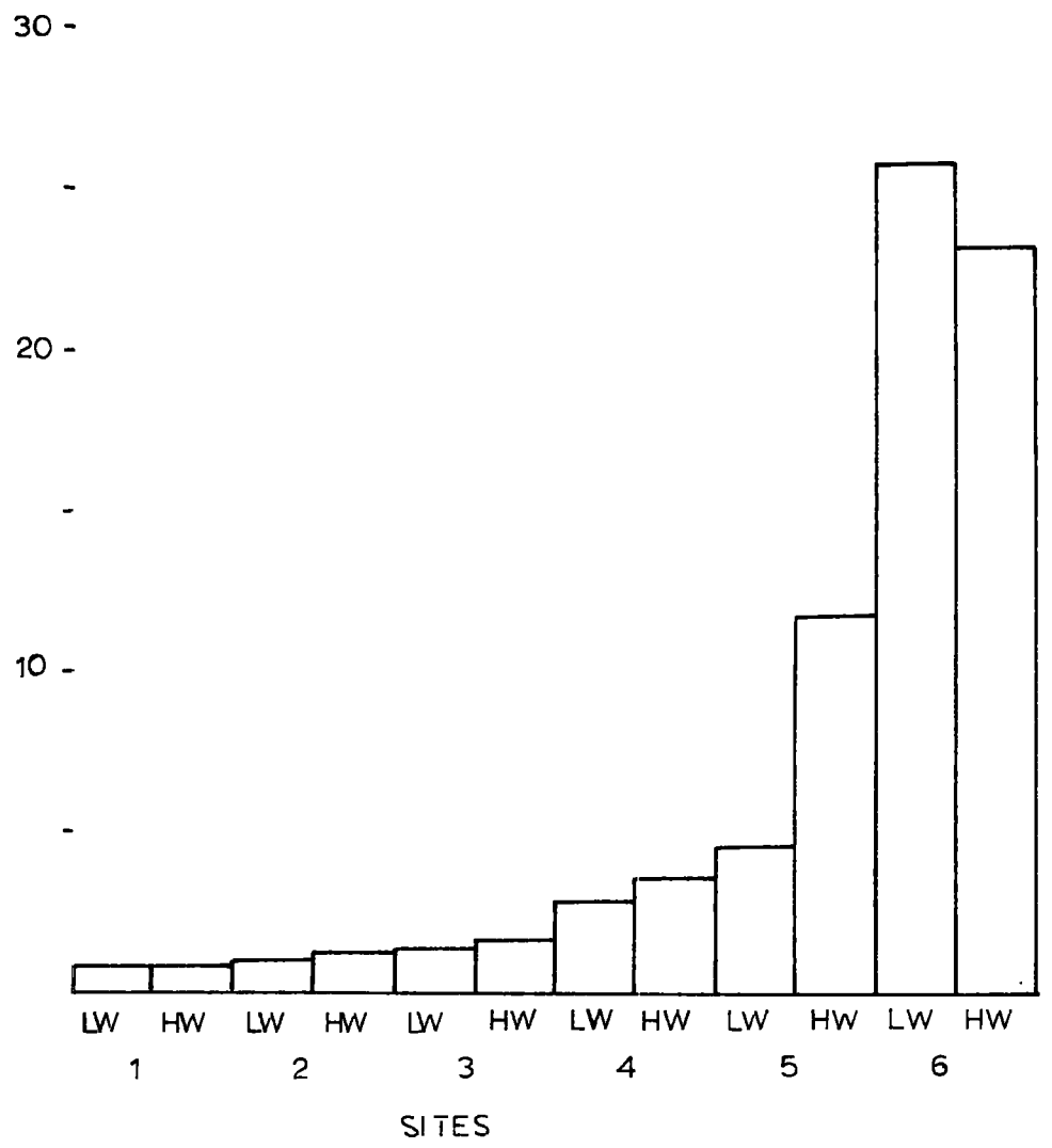
FIGURE 44 . CHLOROSITY VALUES OF WATER SAMPLE FROM SKINNINGROVE BECK.
