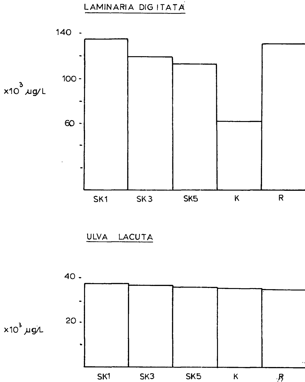
FIGURE 27 . ZINC CONCENTRATIONS IN SELECTED SEaweEDS AT THE SAMPLE SITES.
