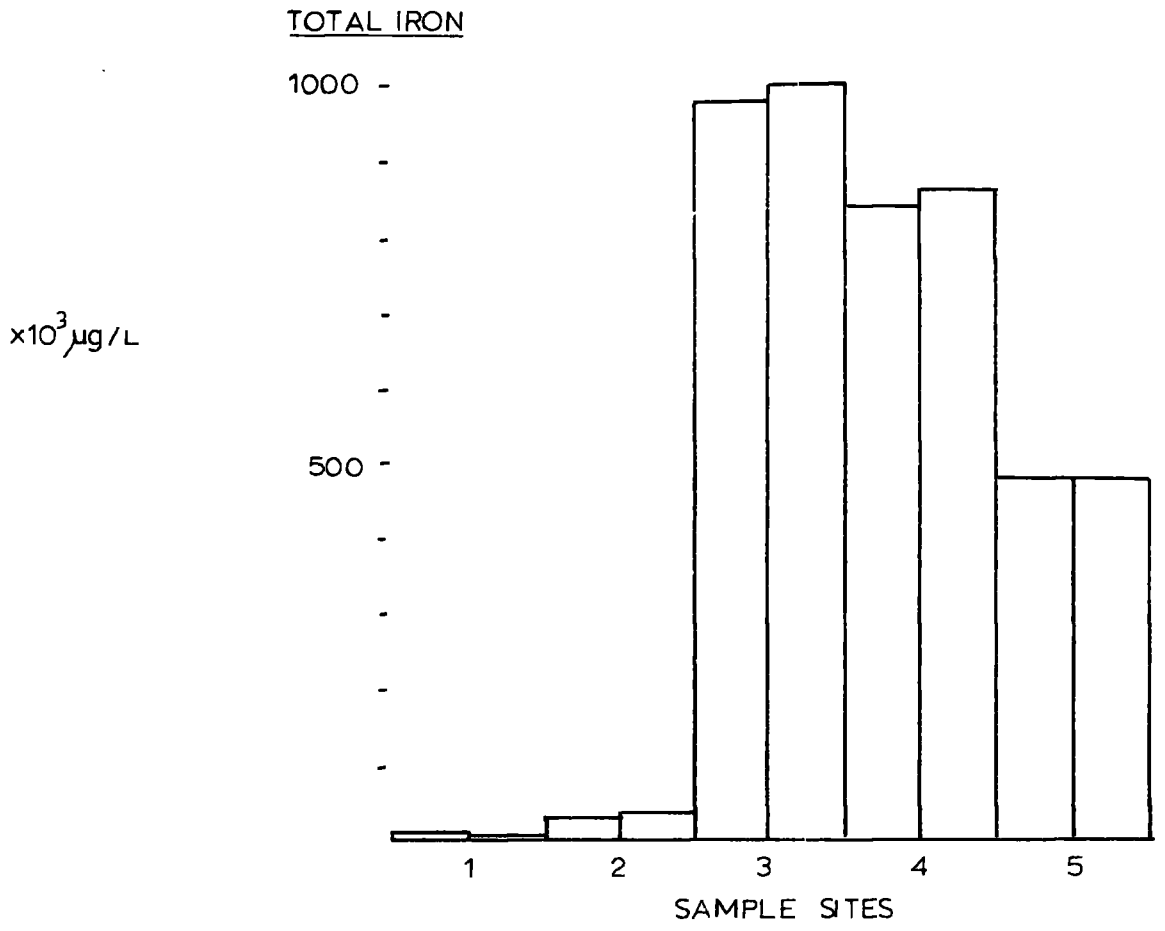
FIGURE 43 . IRON CONCENTRATIONS IN THE WATER FROM SKINNINGROVE BECK.
