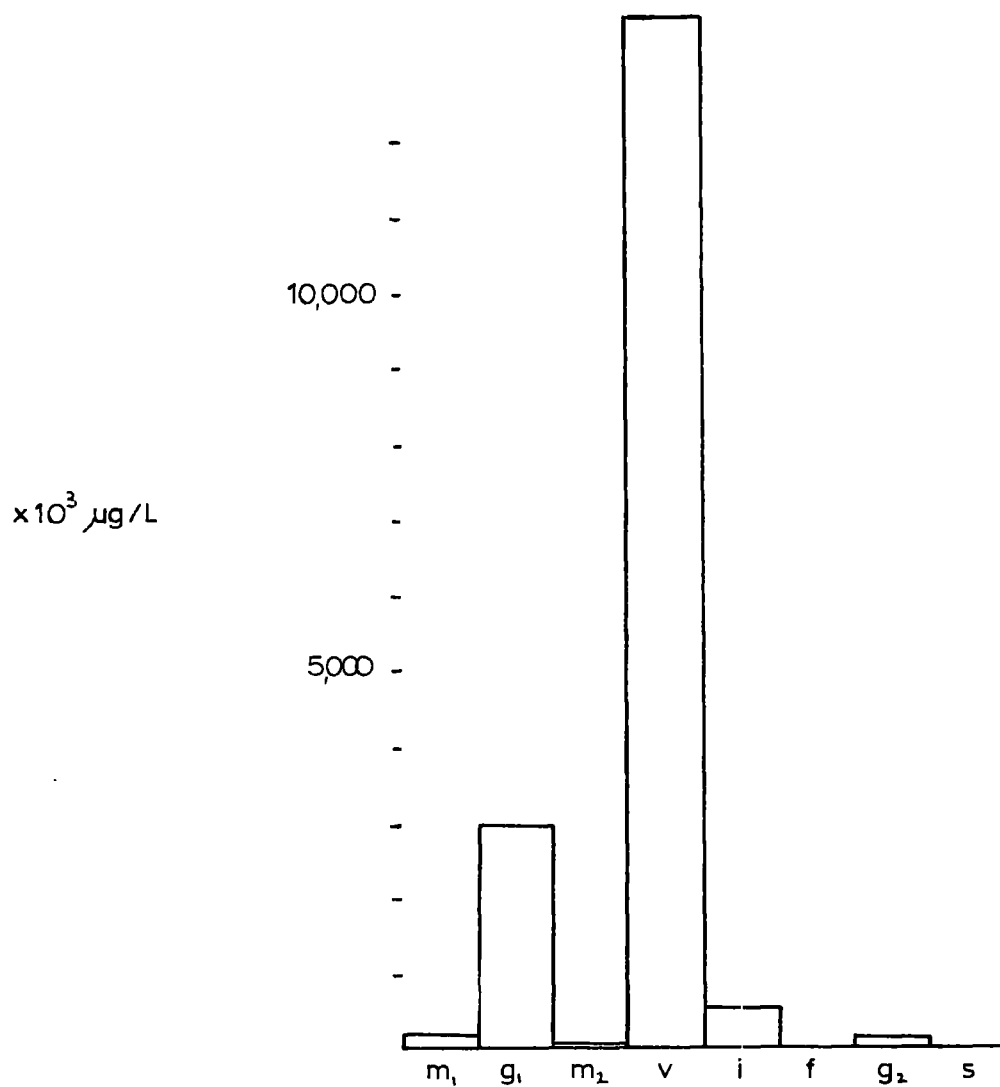
FIGURE 49 . INTERNAL DISTRIBUTION OF IRON IN MUSSELS. ( DATA FROM BROOKS AND RUMSBY 1968 )
