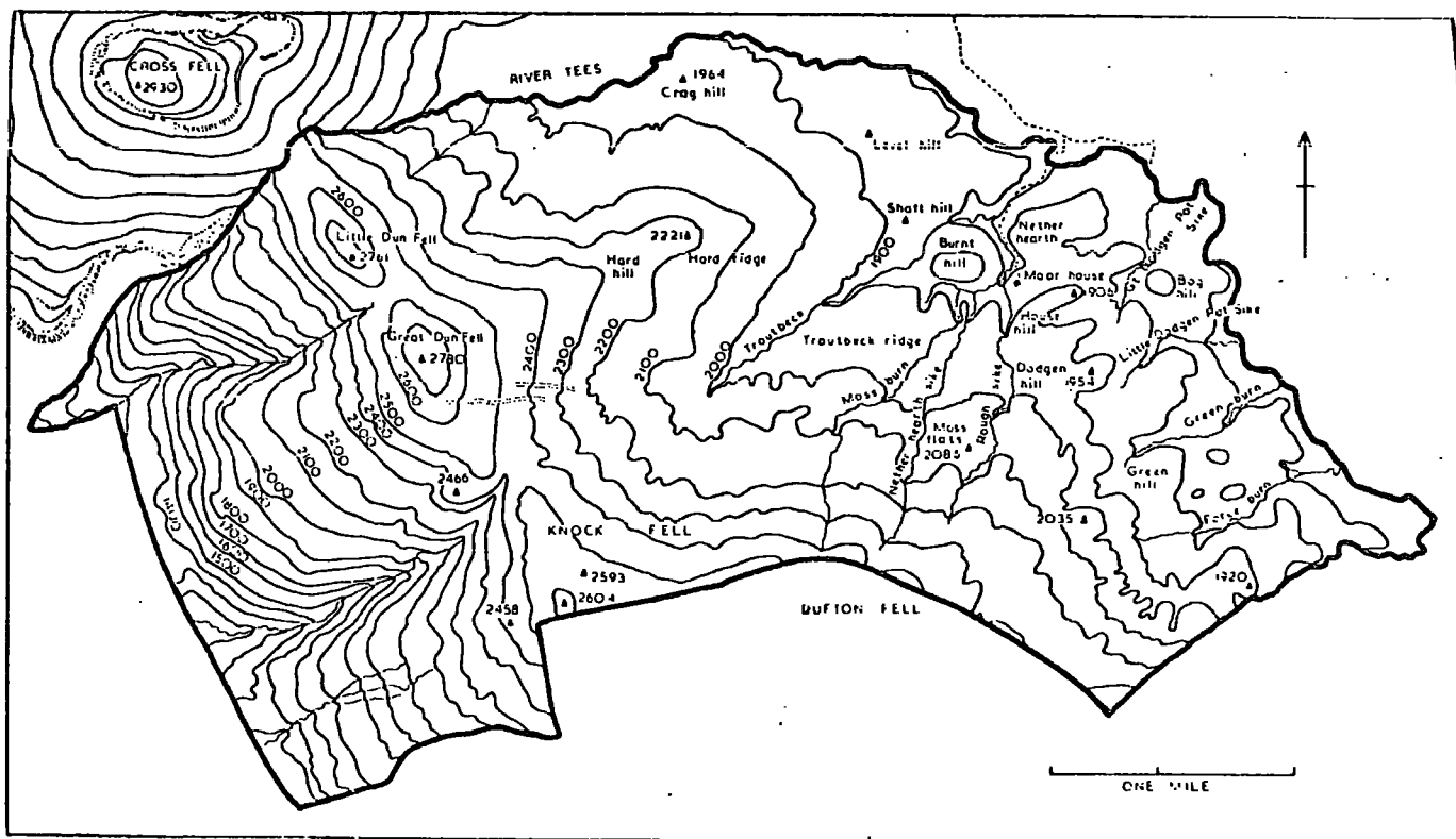
Fig. 1. Map of the Moor House National Nature Reserve showing the major topographical features. (Heights in feet: 1 ft = 0.305 m; 1 mile = 1.6 km approx.) AFTER CRAIG (1961)
