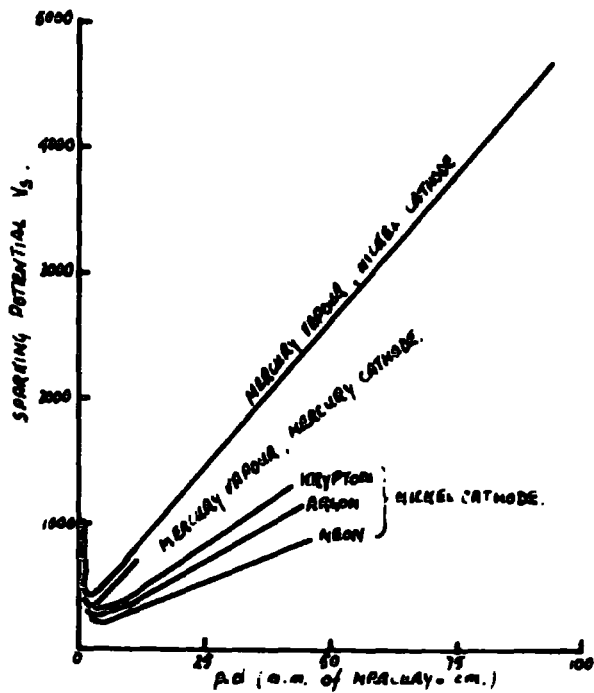
FIG.1.2 PASCHEN CURVES FROM WELSHLYN JONES 1951.
