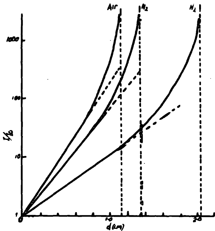
FIG.1.1 TYPICAL LOG I/I_0 , d CURVES FROM WELSHLYN JONES 1951.
