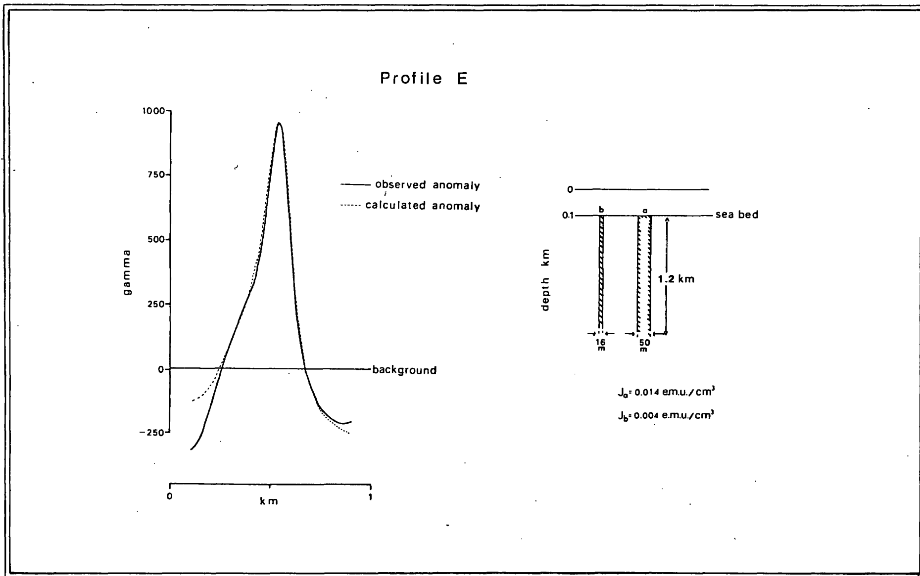
Fig. 10 Interpretation of a Magnetic Feature Associated with the Magnetic High
