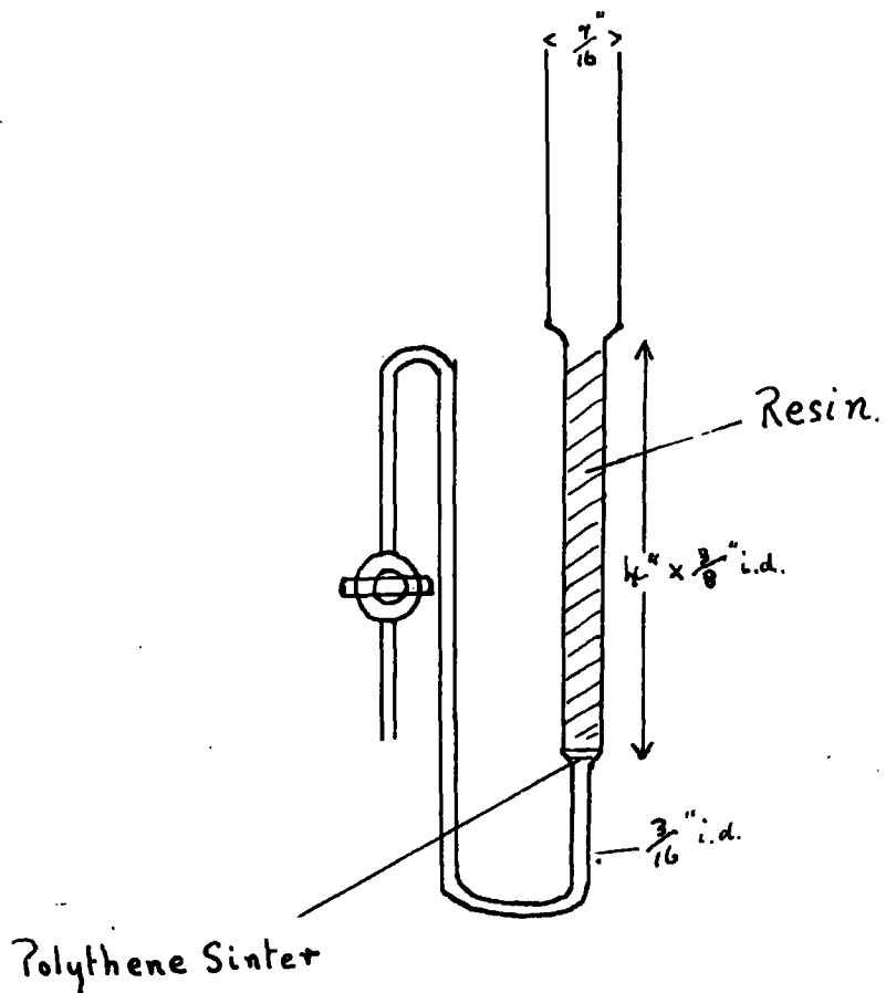
RESIN' EXCHANGE COLUMN.
