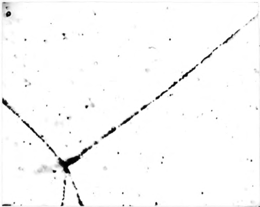
Thorium-X Stat. The long track is due to the alpha-particle from Thorium-C'. (Magnification about 2500 x)
