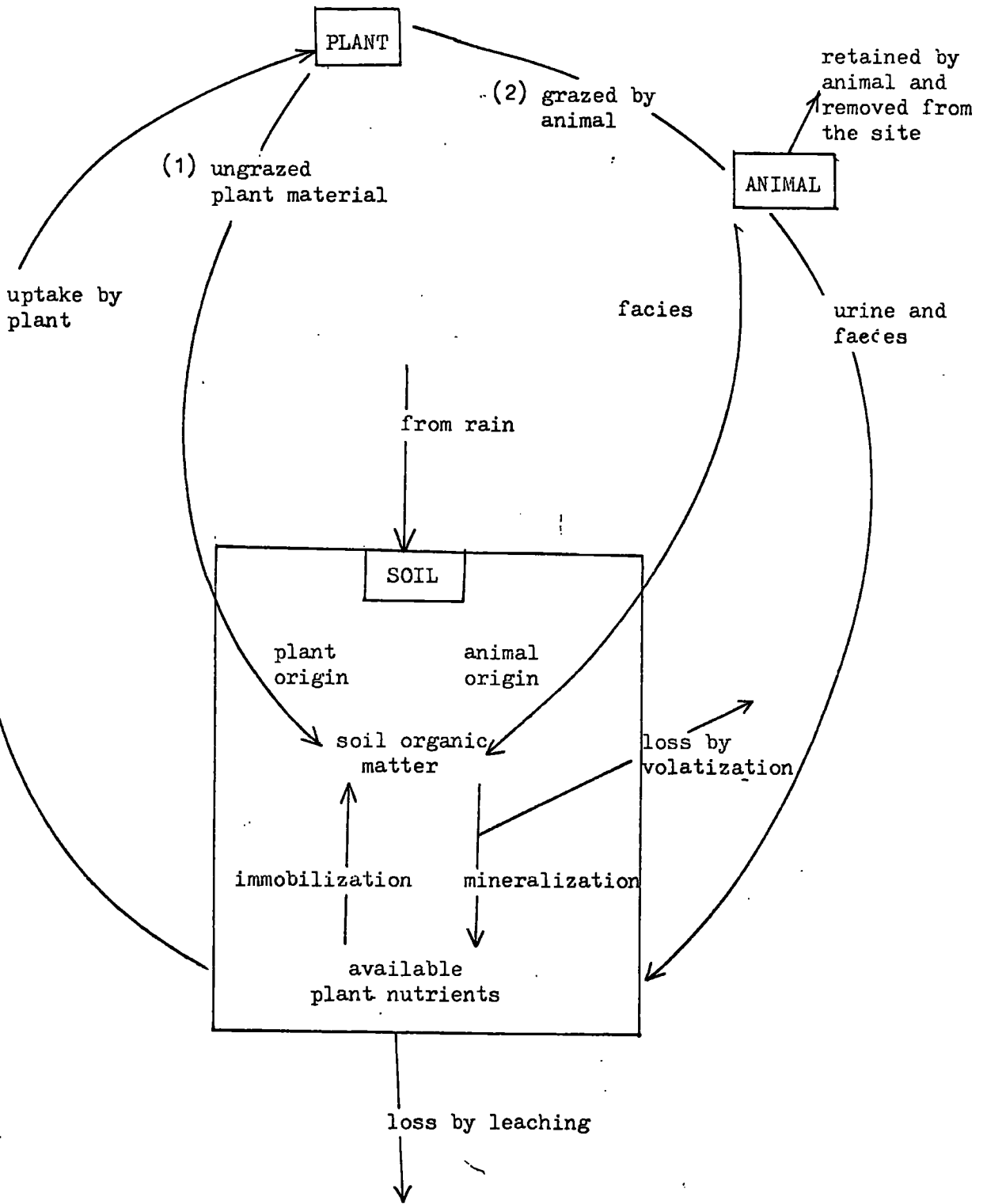
Fig. 46 Nutrient cycle on Waldrige Fell.
