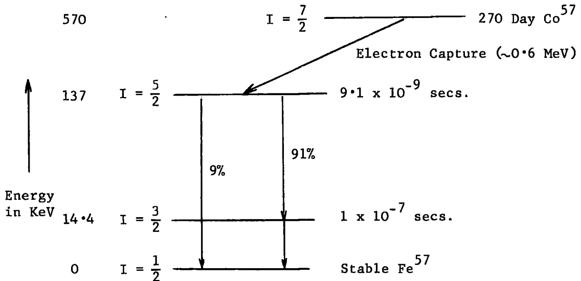
Fig.6-1 Scheme for the Decay of Co^{57} to Fe^{57}
