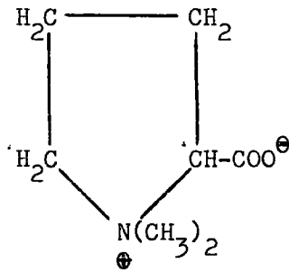
Stachydrine (proline betaine)
