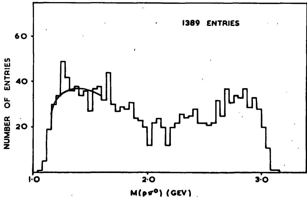
B. M(\rho\pi^0)
