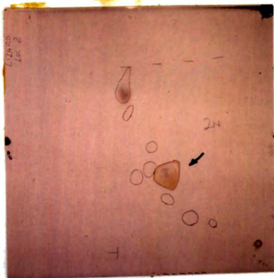
Two dimensional chromatogram of British diploid. The large spot represents compounds 8 and 9 of Fig. 49. →
