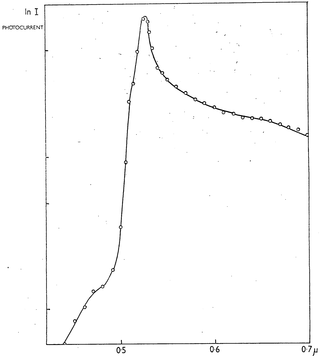
PHOTOCONDUCTIVE SPECTRAL RESPONSE
