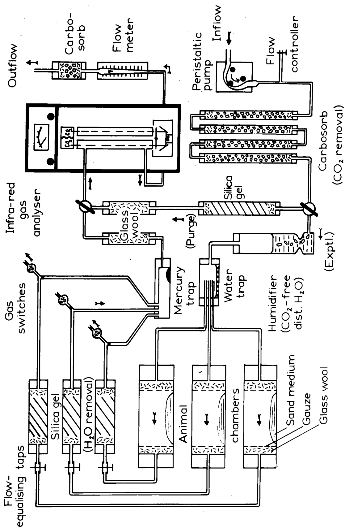
Fig. 29. The infra-red gas analysis apparatus (see text).
