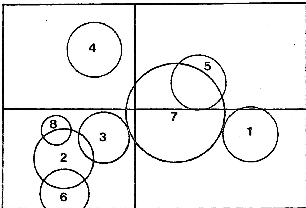
PRINCIPAL COMPONENT 1
