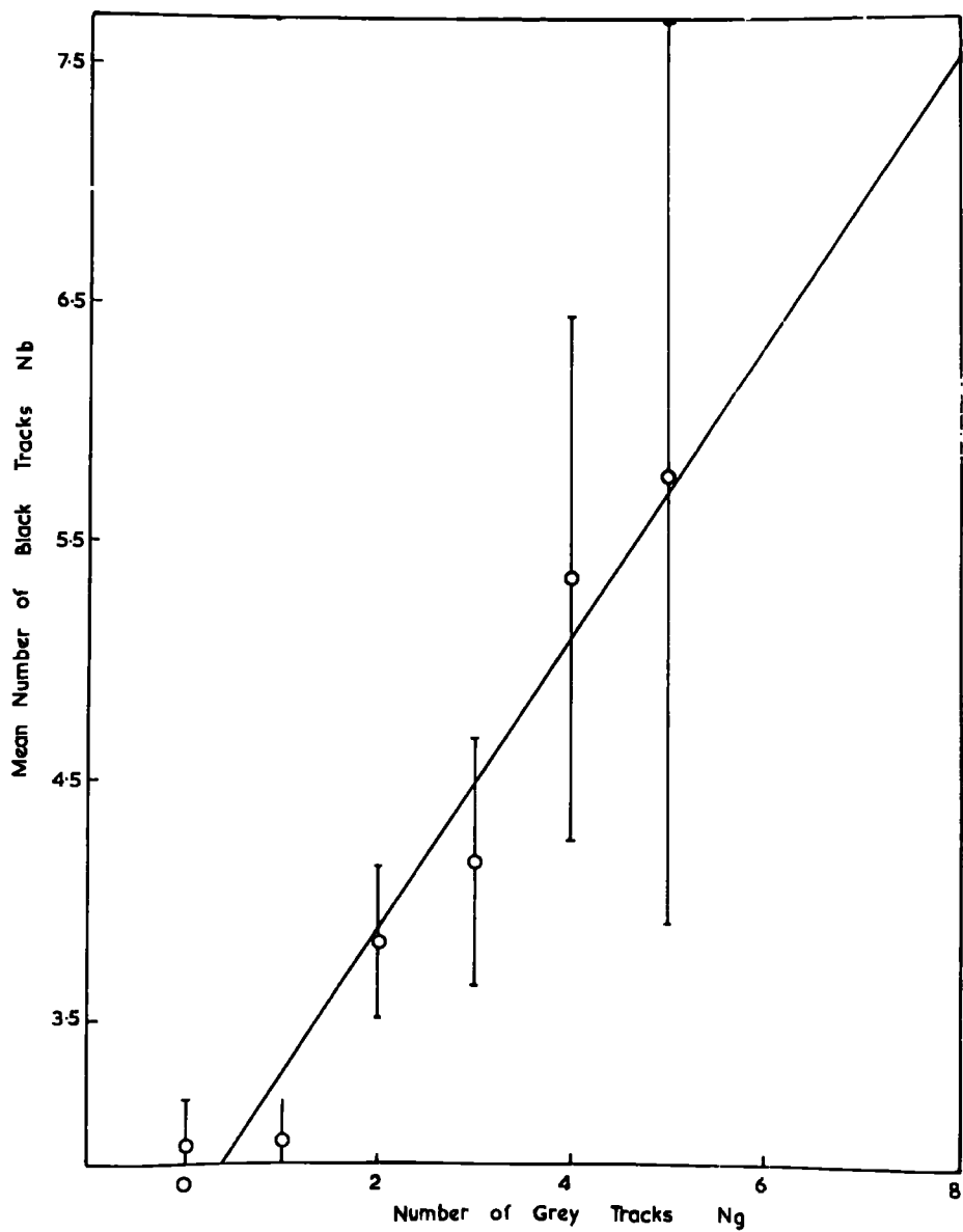
FIG. 12 The variation of mean number of black tracks with number of grey tracks.
