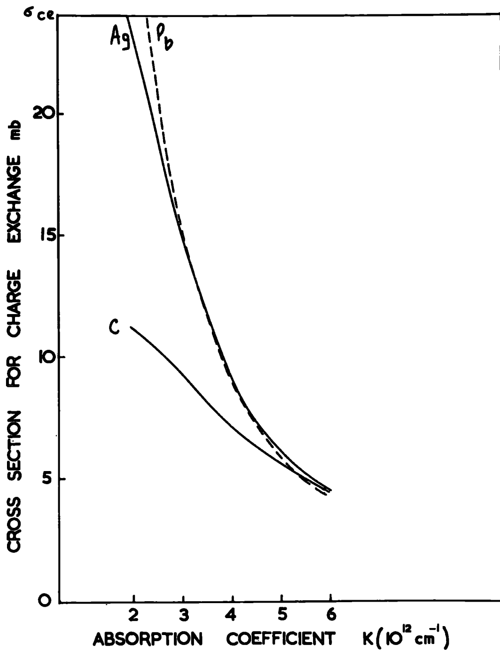
FIG 20 The variation of charge exchange cross-sections with absorption coefficient
