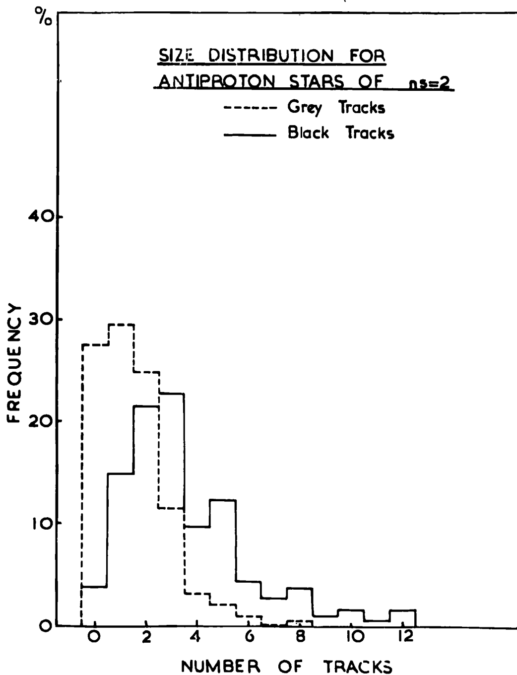
FIG. 15 Size dis n for antiproton stars ns=2
