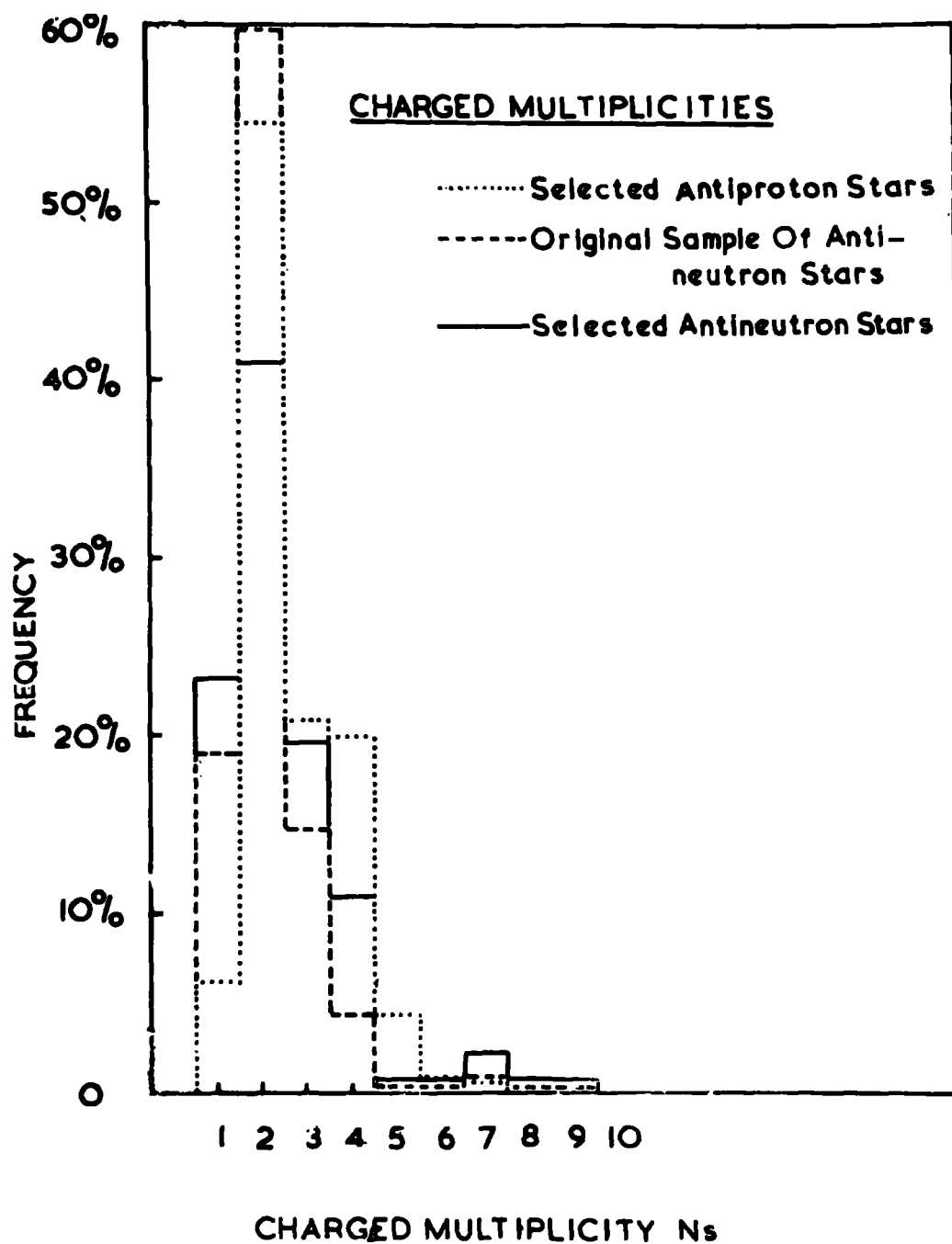
FIG.24 The comparison of charged multiplicities
