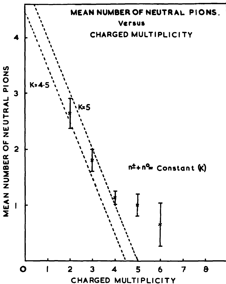
FIG. 5 Mean number of neutral pions accompanying particular charged multiplicities
