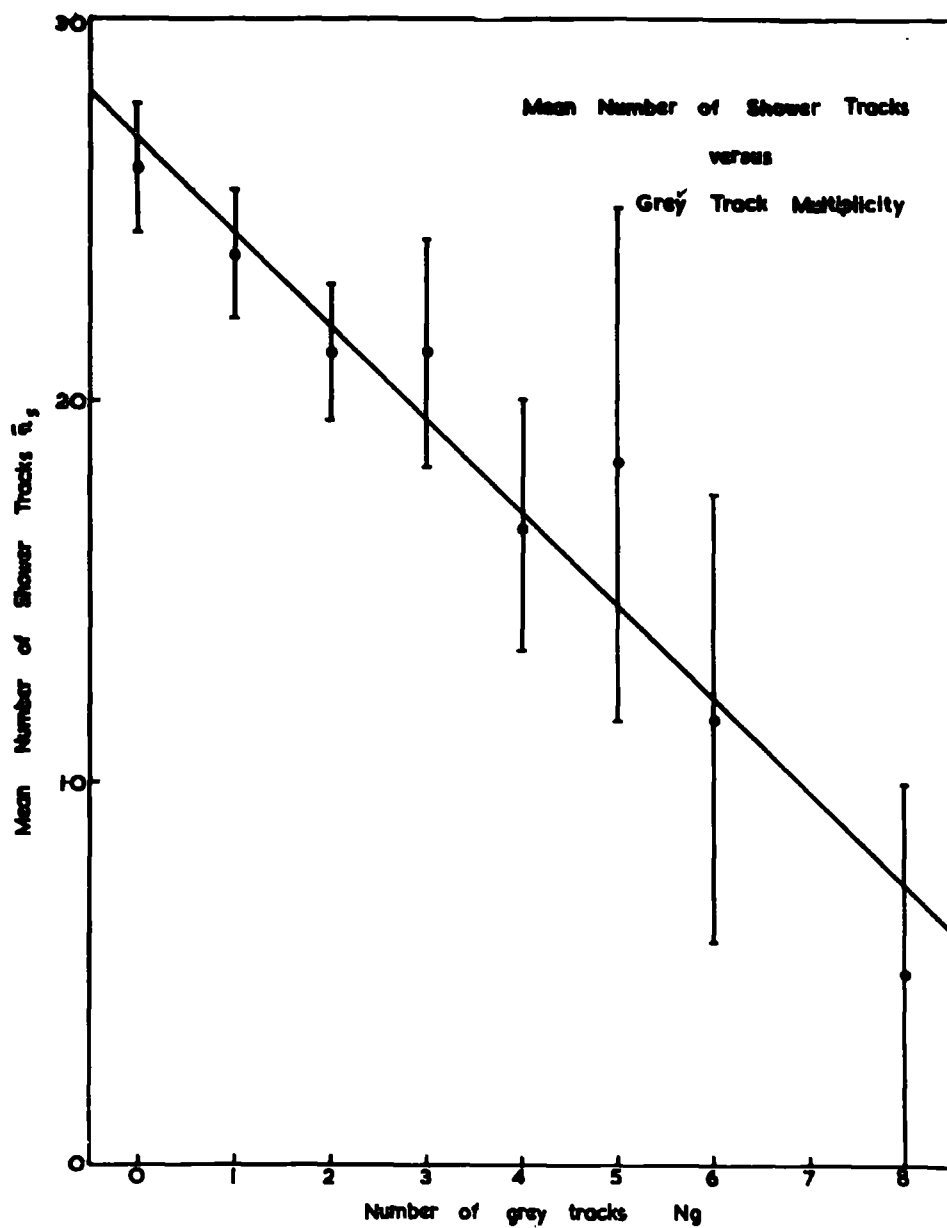
FIG. 13 The variation of the mean number of shower tracks with the grey track multiplicities.
