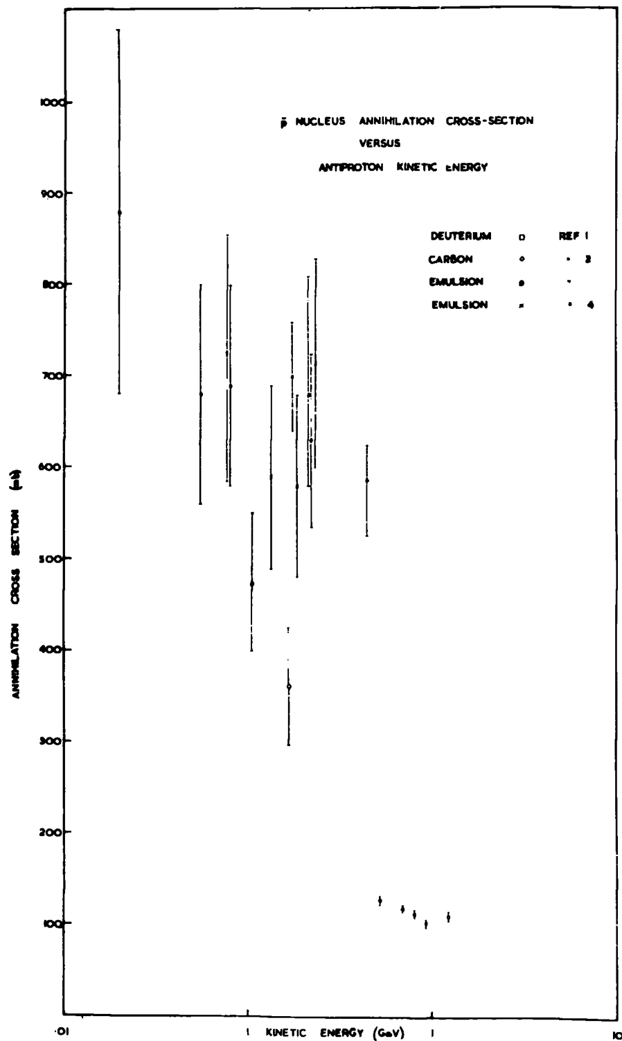
FIG. 2 Annihilation cross sections in complex nuclei
