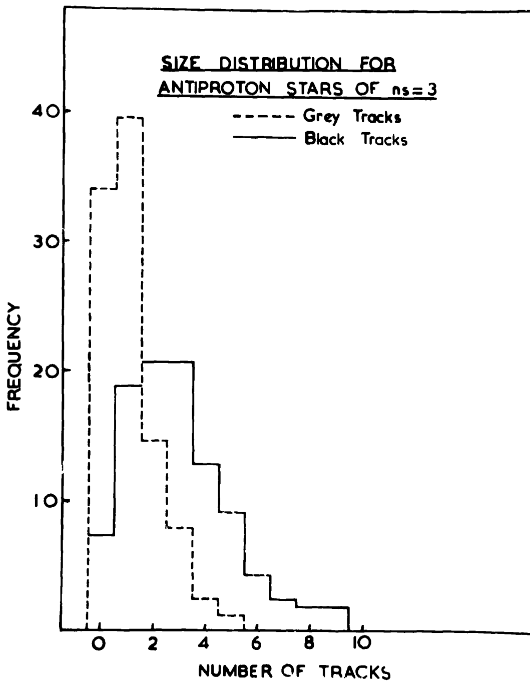
FIG. 16 Size dis n for anti-proton stars n_s=3
