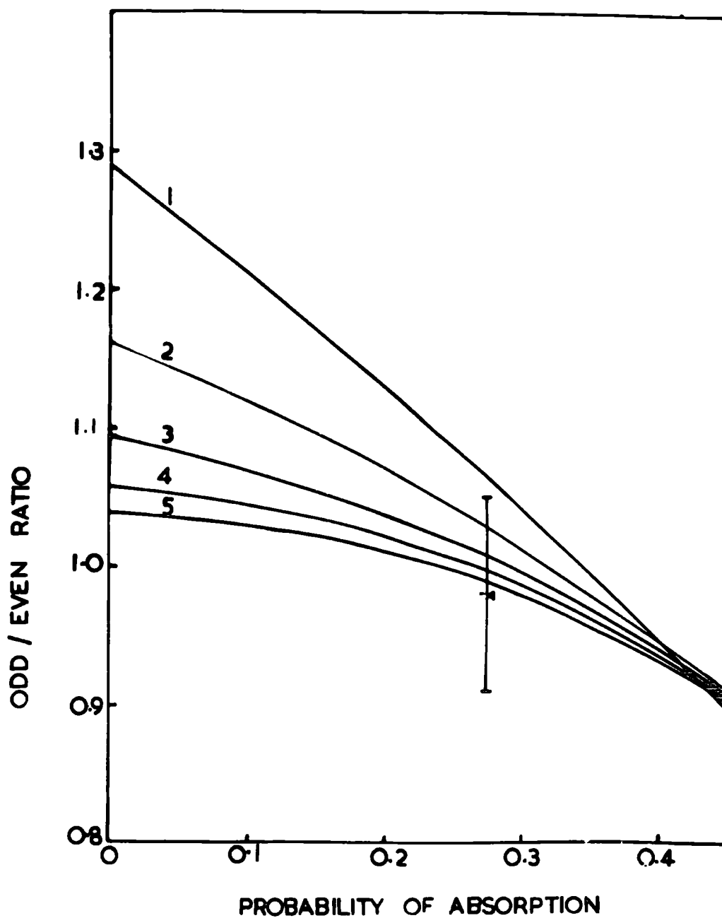
FIG 8 The calculated variation of odd even ratio due to absorption and charge exchange of secondary mesons
