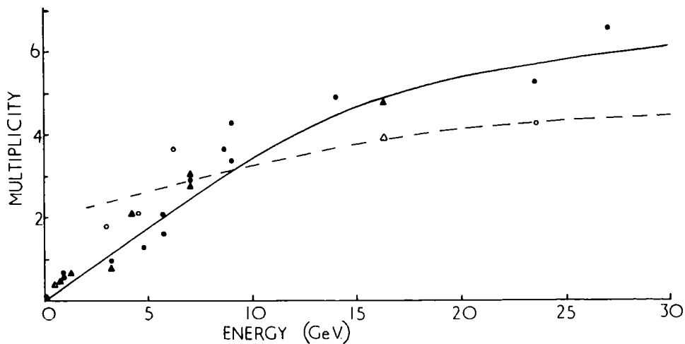
Fig.3. The variation of multiplicity with energy for p-p, \circ ; p-nucleus, \bullet ; \pi -p, \triangle ; and \pi -nucleus, \blacktriangle ; collisions ——— collisions with nuclei - - - collisions with nucleons
