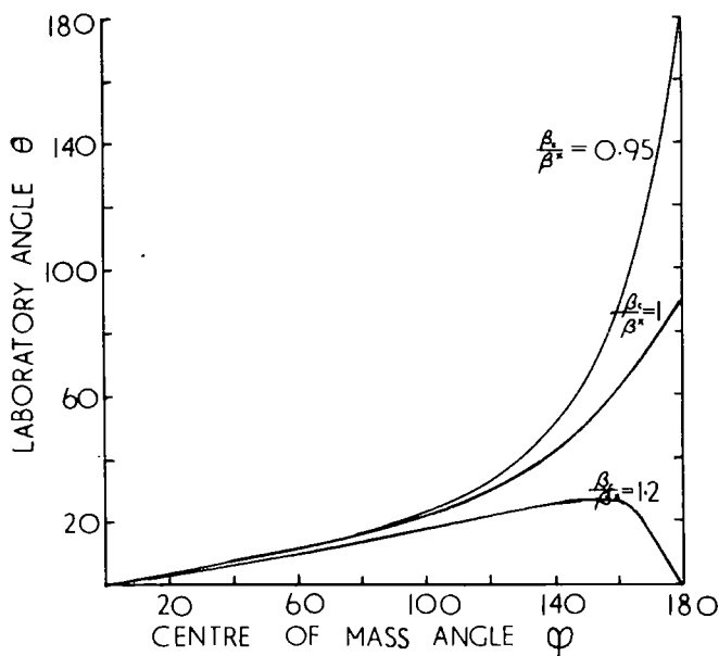
Fig.4. The relation between the of angle of emission in the centre of mass and laboratory systems for secondary particles whose velocities are given by \frac{v}{v^*} = 0.95, 1 and 1.2
