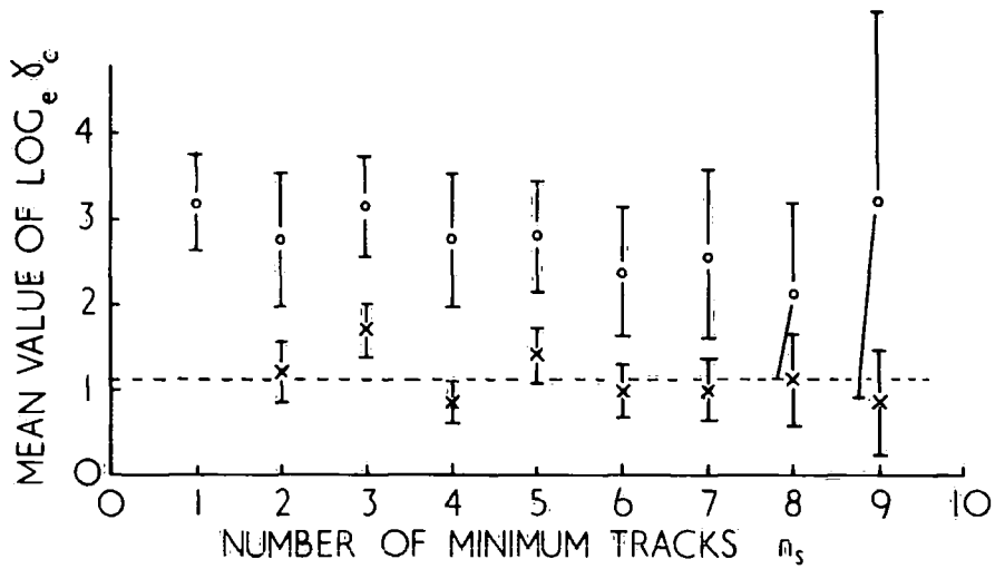
Fig. 24. The relation between the corrected value of \log_e \chi_c and the number of minimum tracks for events produced by 16.3 Gev. \pi^- -mesons with n_q=0 . o \ln \cot \theta for the discarded particle. x corrected \log_e \chi_c
