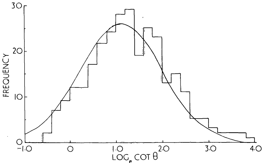
Fig. 25. The distribution of \log_e \cot \theta for events produced by 16.3 Gev. \pi^- -mesons with n_q=0 and excluding the continuing primary.
