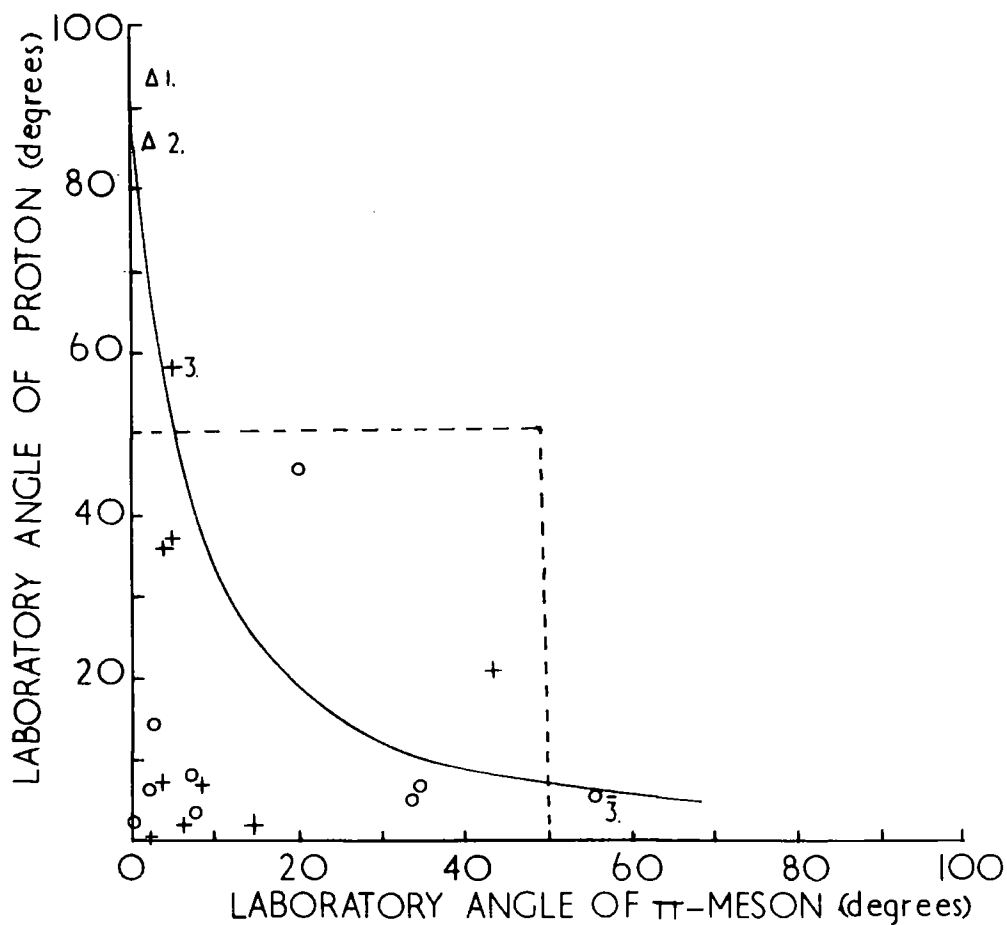
Fig.6. The comparison of the observed and calculated angles of emission for possible \pi^- -p elastic scatterings at 16.3 Gev.
