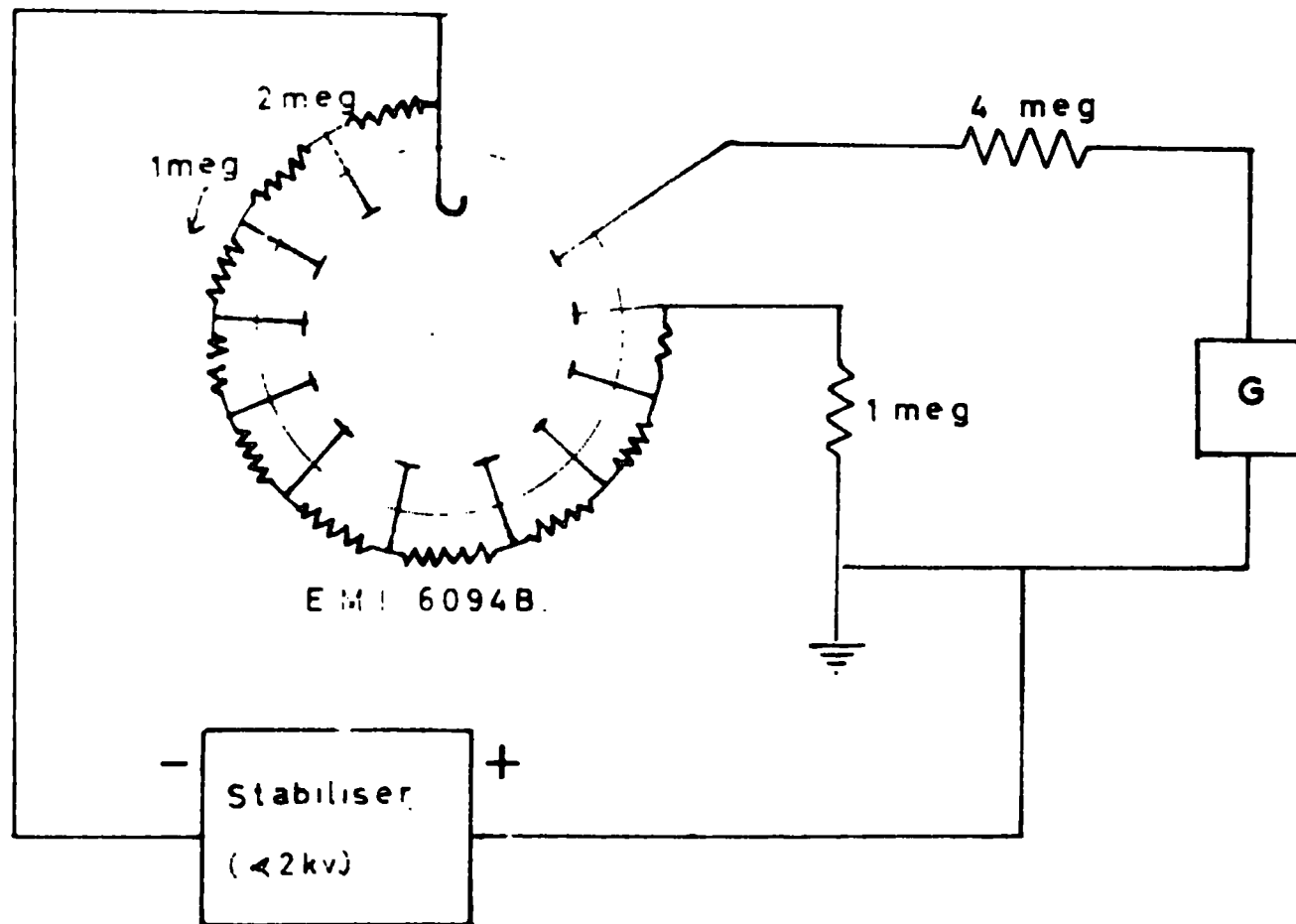
FIG 1 CIRCUIT DIAGRAM FOR REFLECTIVITY MEASUREMENTS.
