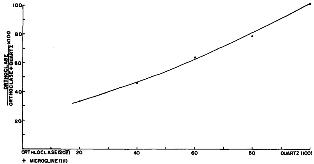
DIAGRAM 7 RELATIVE INTENSITY OF X-RAY DIFFRACTION PEAKS
