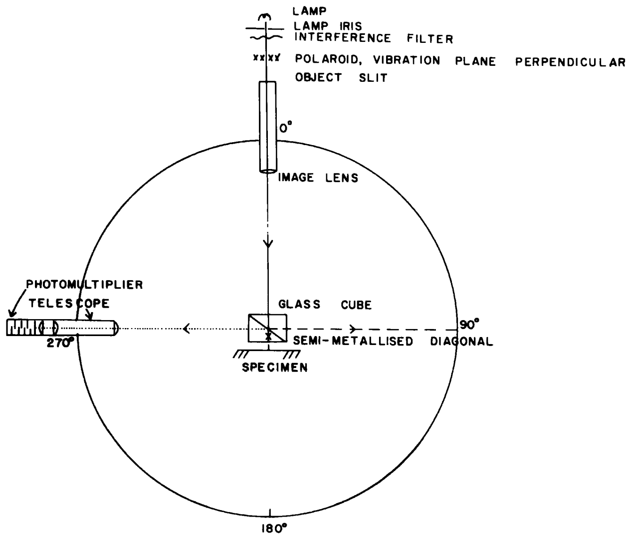
DIGRAM 4 PLAN VIEW WITH SPECIMEN IN PLACE
