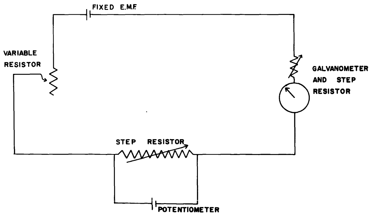
FIGURE 3 LINEARITY OF THE 1/100 th AND 1/1000 th SCALES
