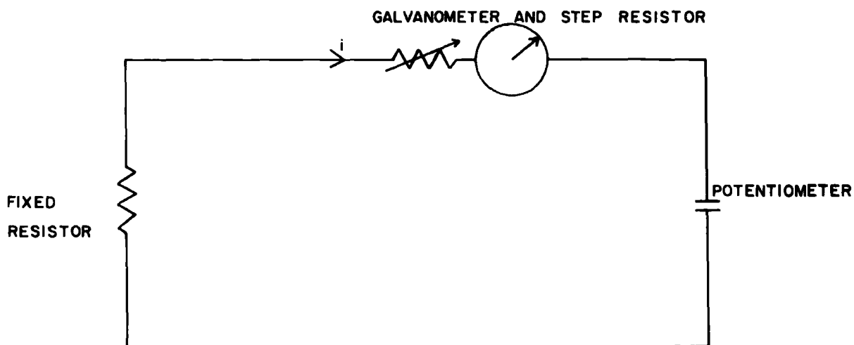
FIGURE 2 FOR DETERMINING THE LINEARITY OF GALVANOMETER ON THE 1, 1/10 , AND 1/100 th SCALES
