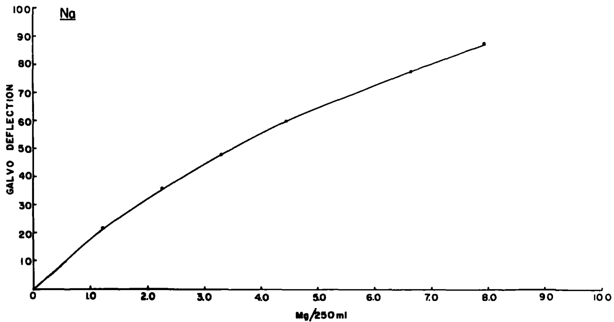
DIAGRAM 2 FLAME PHOTOMETER CALIBRATION FOR Na AND K
