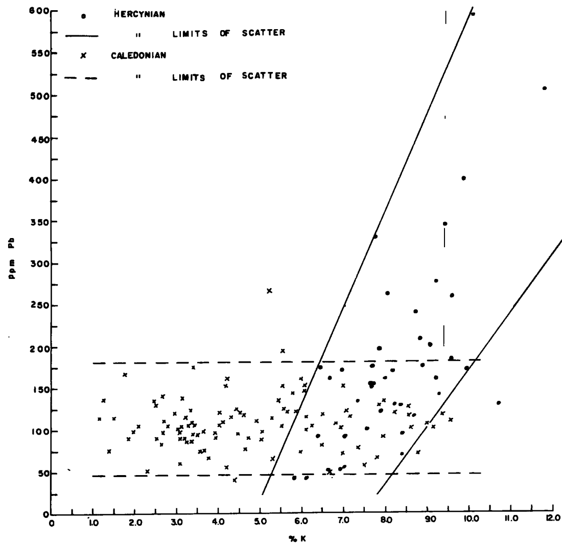
DIAGRAM 16 PLOTS OF Pb vs K IN FELDSPAR
