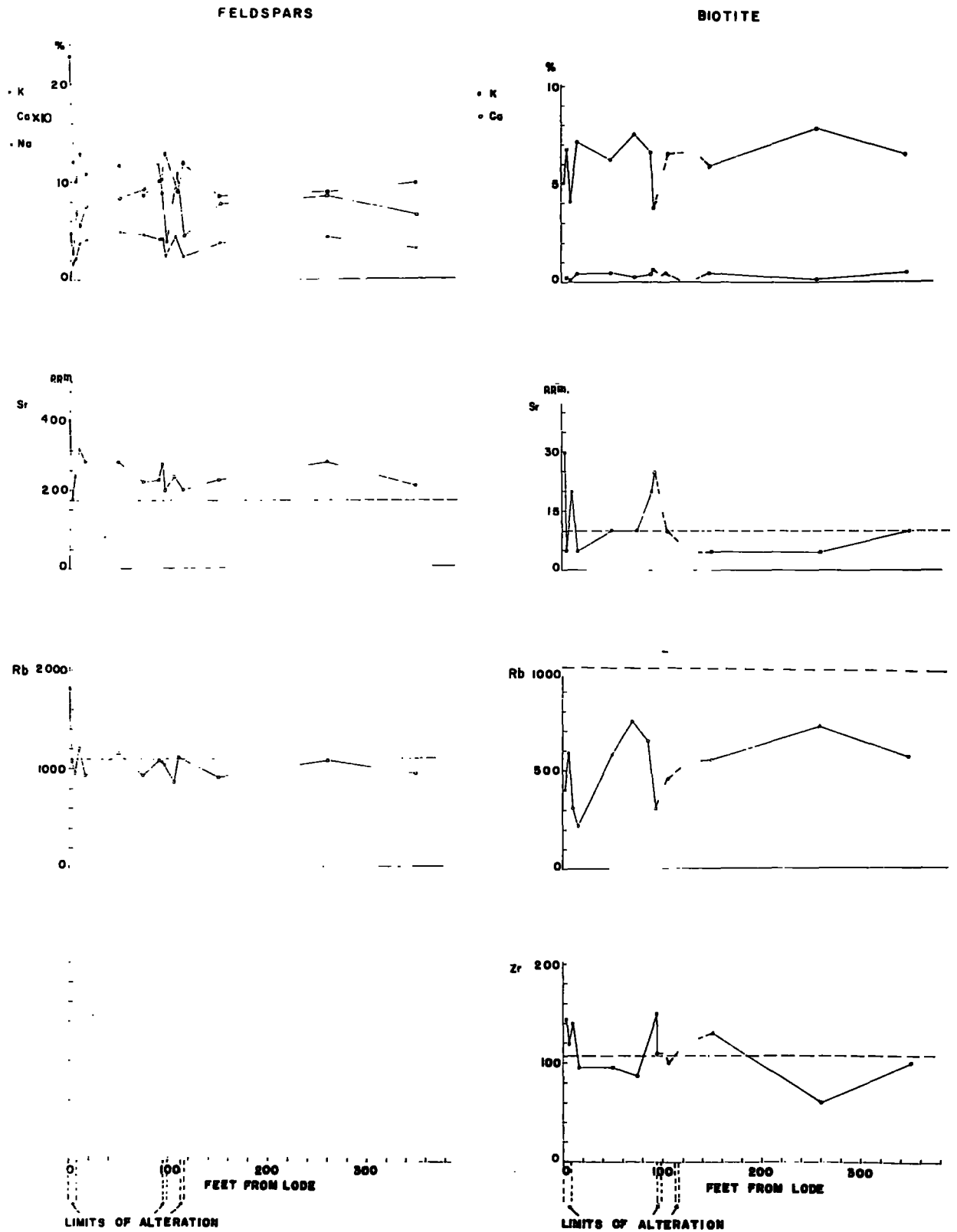
DIAGRAM 29 WALL ROCK ALTERATION, GEEVOR MINE
