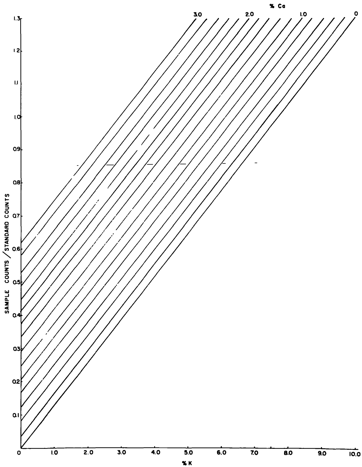
DIAGRAM 3 STANDARD CURVES FOR K IN BIOTITE BY X-RAY FLUORESCENCE
