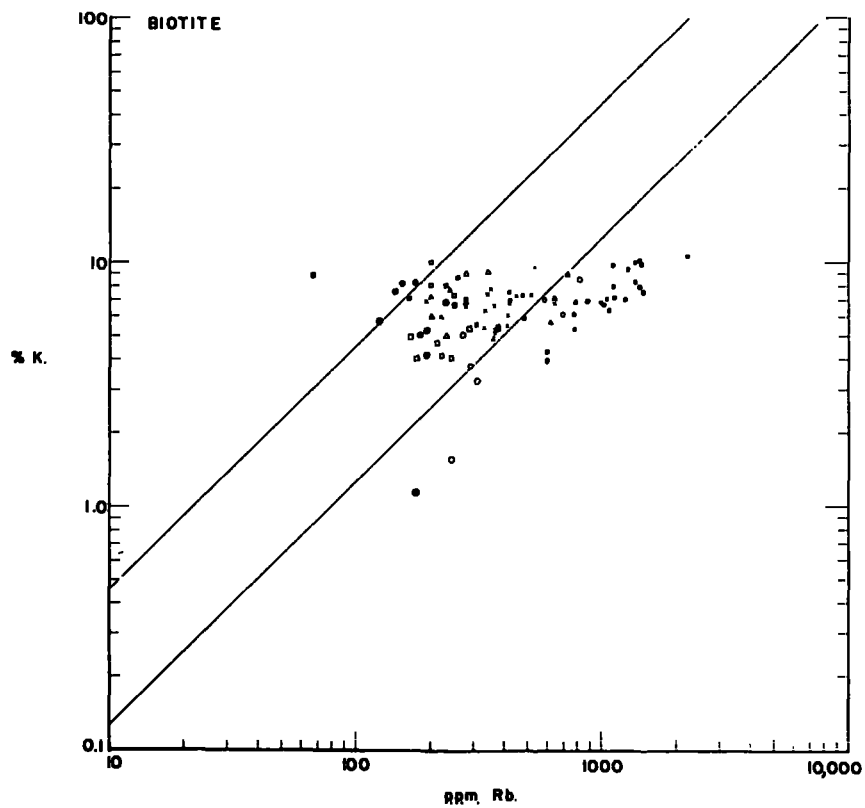
DIAGRAM II PLOTS OF K vs Rb IN FELDSPAR AND BIOTITE
