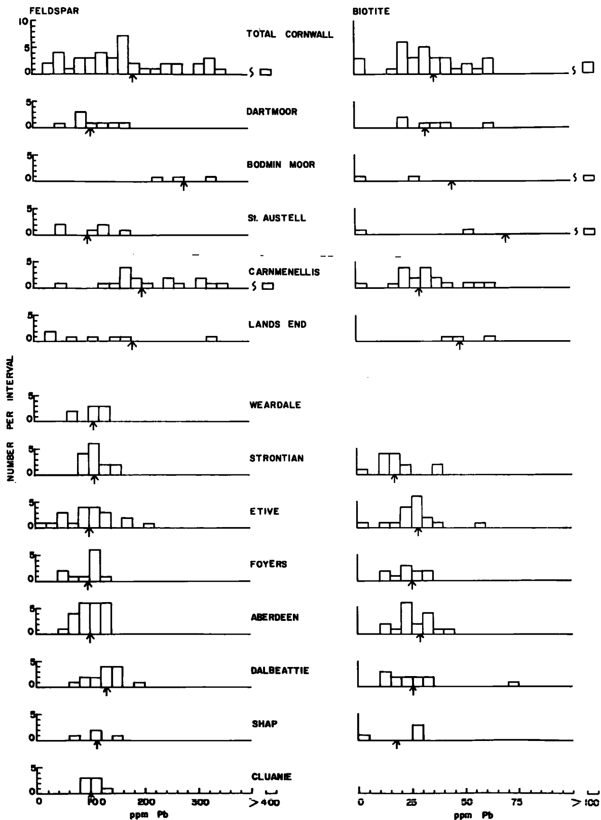
DIAGRAM 15 Pb ANALYSES
