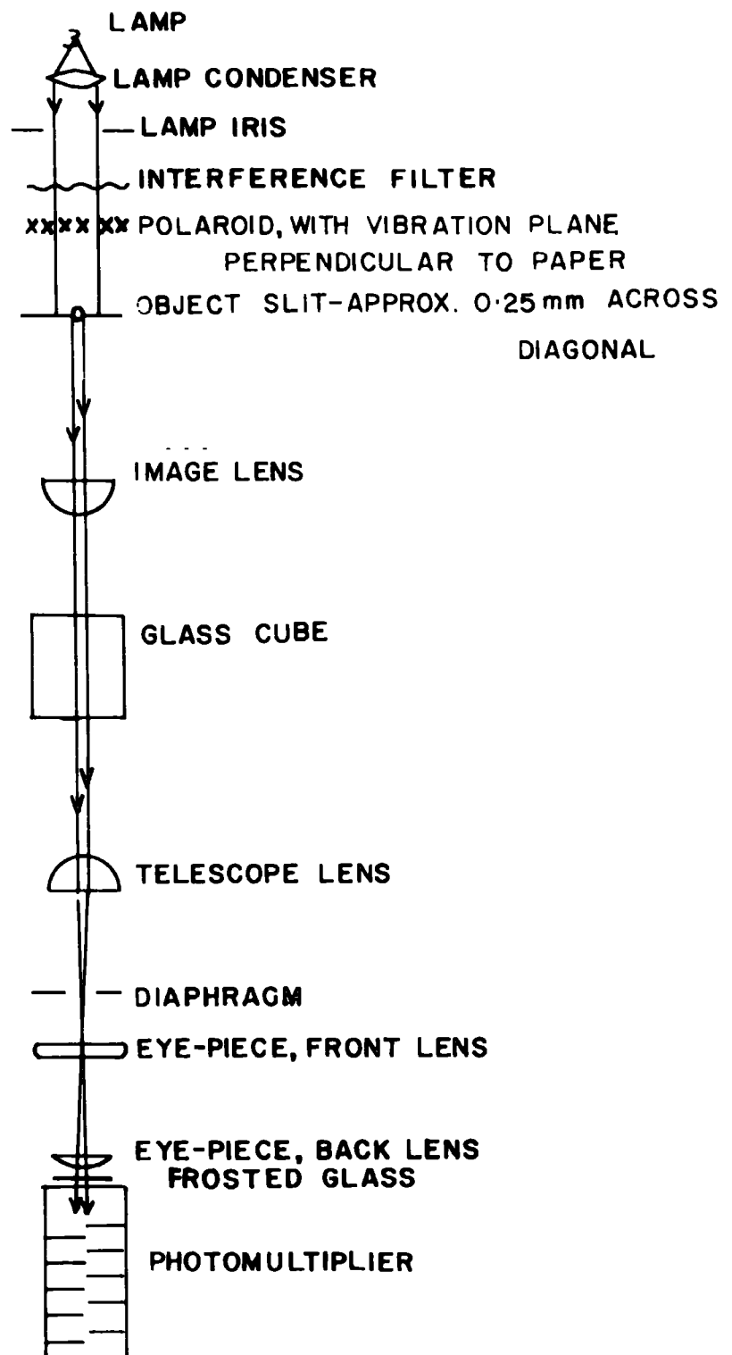
DIAGRAM 3 RAY DIAGRAM APPARATUS FROM CROSS-SECTIONAL VIEW
