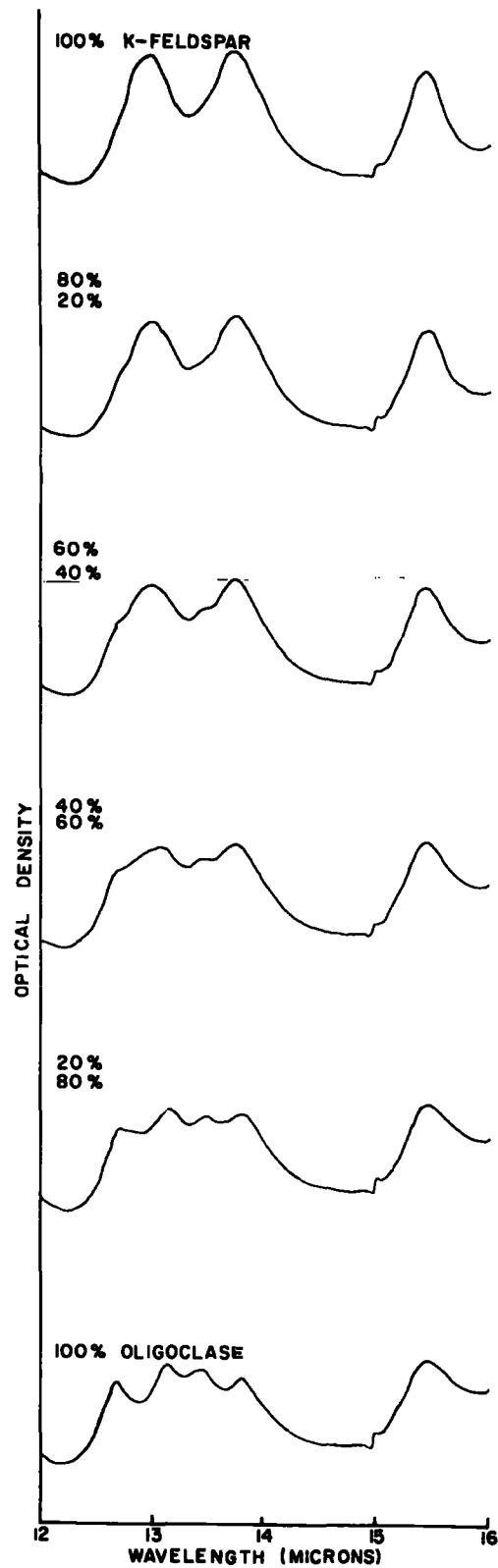
DIAGRAM 5 INFRARED CURVES FOR CHANGES IN K-FELDSPAR-OLIGO- CLASE CONCENTRATION
