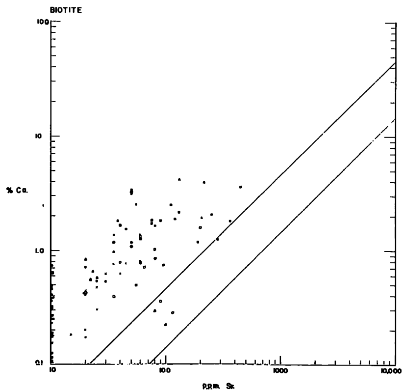
DIAGRAM 14 PLOTS OF Co vs Sr IN FELDSPAR AND BIOTITE
