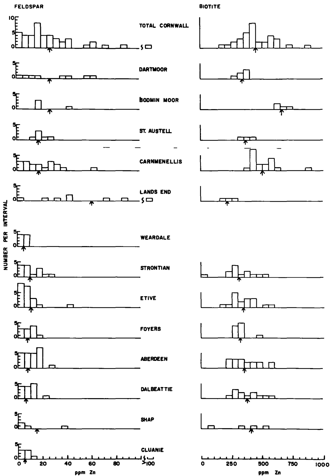
DIAGRAM 18 Zn ANALYSES
