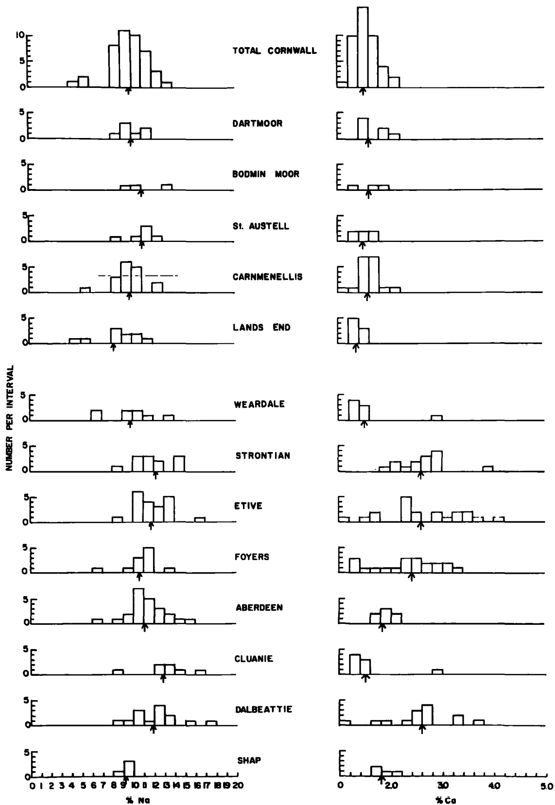
DIAGRAM 8 Na AND Ca ANALYSES IN FELDSPAR
