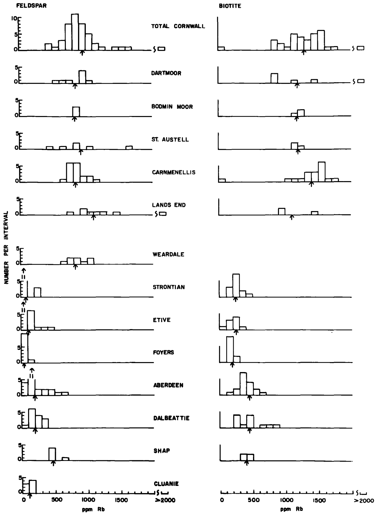
DIAGRAM 10 Rb ANALYSES
