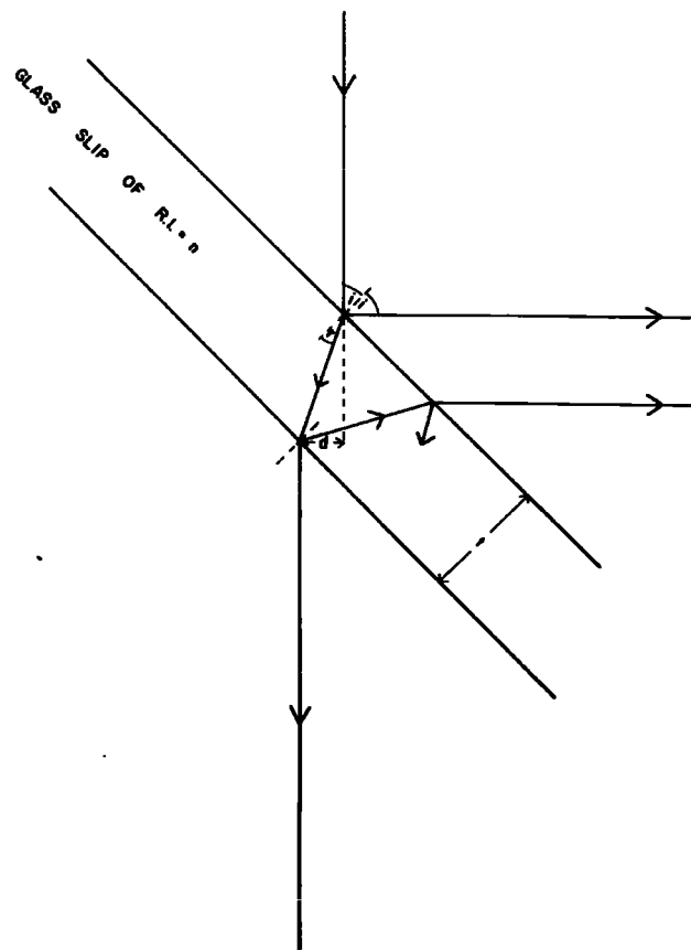
DIAGRAM 2 DISPLACEMENT OF A LIGHT BEAM AFTER PASSING THROUGH A GLASS SLIP
