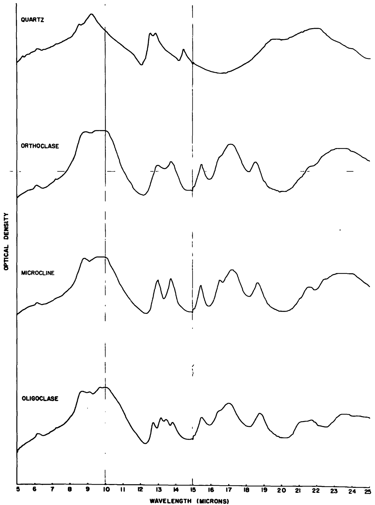
DIAGRAM 4 INFRA-RED CURVES FOR PURE MINERALS
