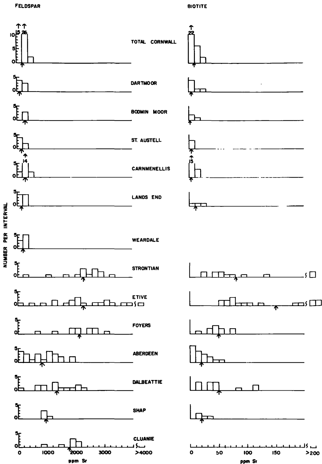
DIAGRAM 13 Sr ANALYSES
