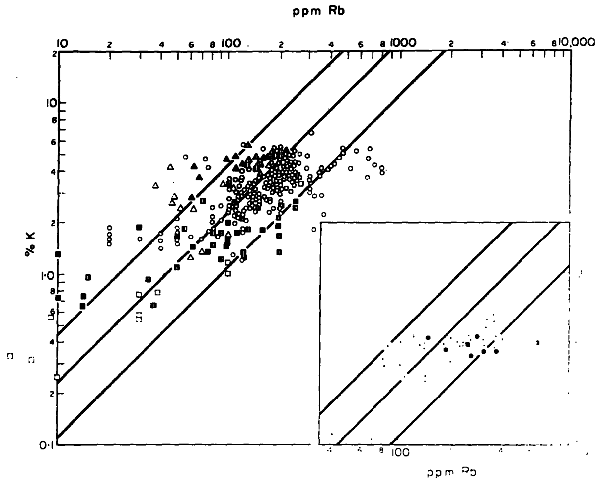
DIAGRAM. [2] Plots of Rb vs. K in plutonic rocks. (AFTER HEIER AND ADAMS)
