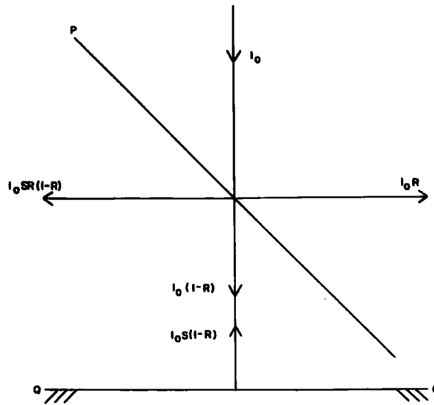
DIAGRAM 1 RAY DIAGRAM
