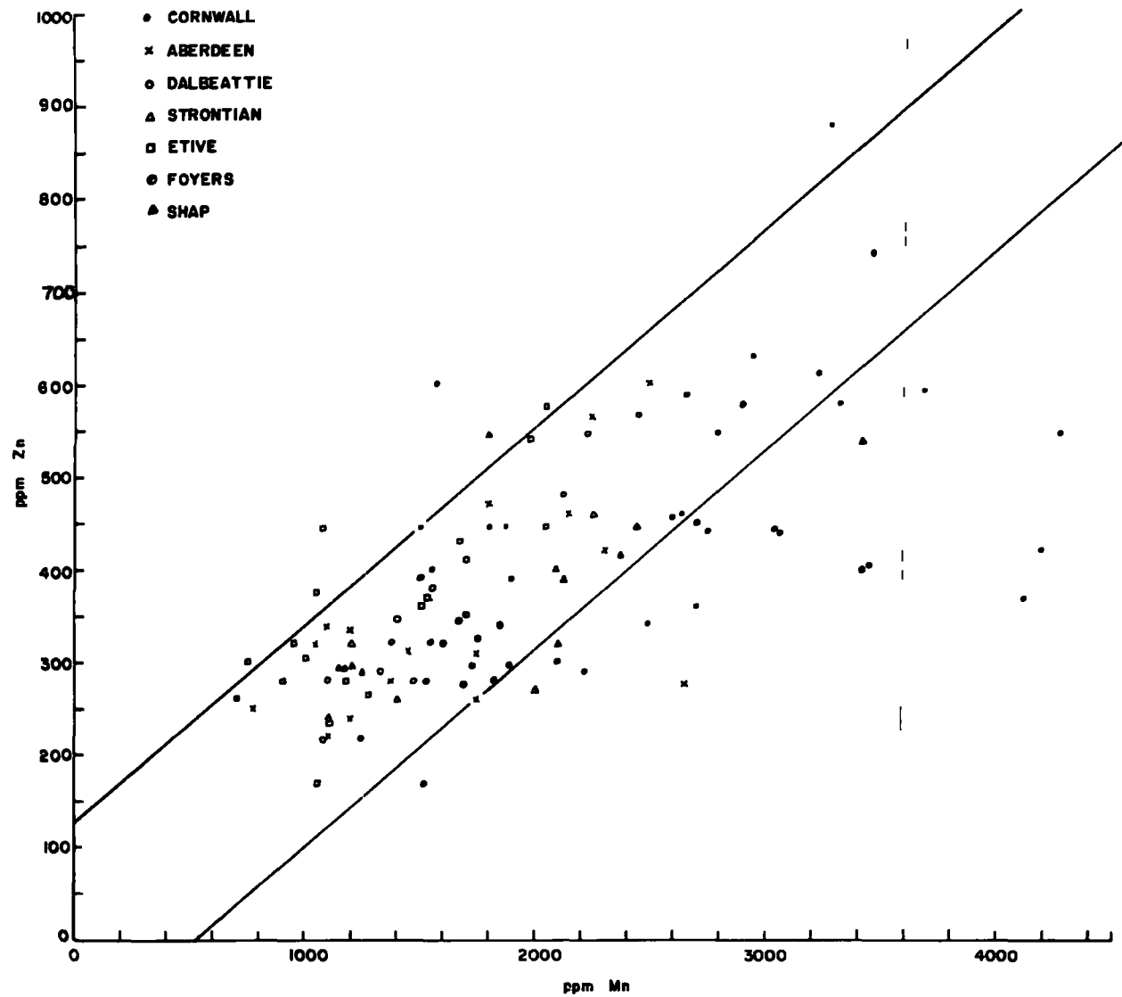
DIAGRAM 20 PLOTS OF Zn vs Mn IN BIOTITE
