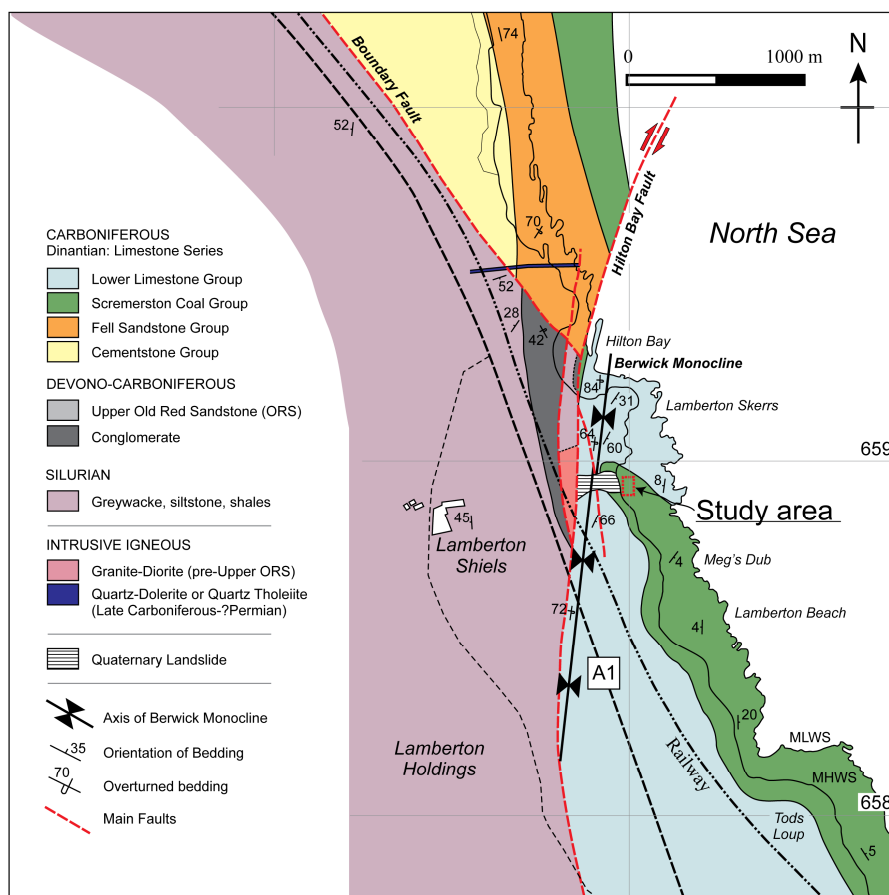
Fig. A15. Location map for the study area at Lamberton.
