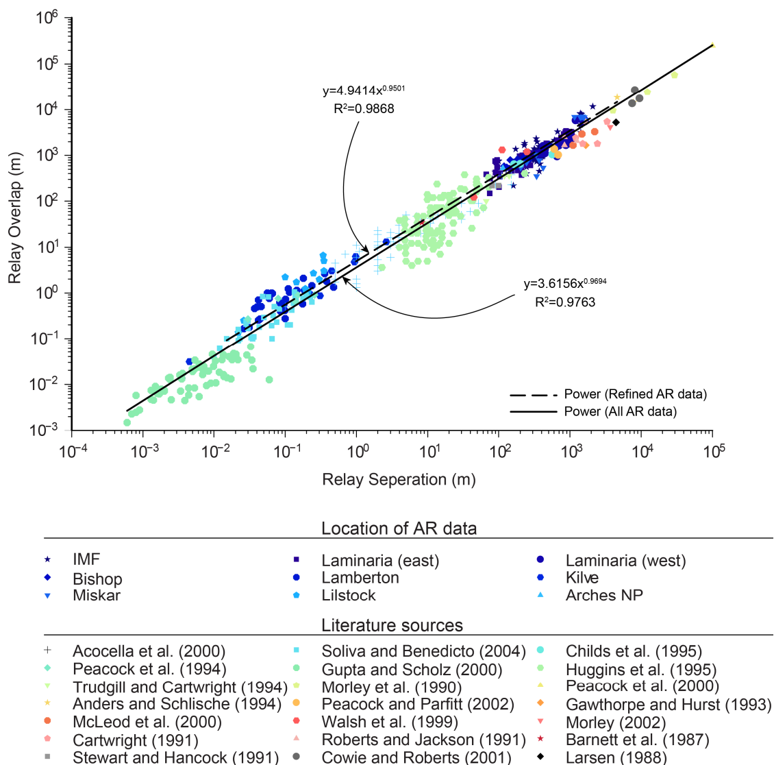
Fig. 5.20. A log-log plot of overlap versus separation for all AR measurements, coloured for their data source. For comparison, the power-law trend line for all the AR data is plotted alongside the trend line for the refined dataset (Fig. 5.21).
