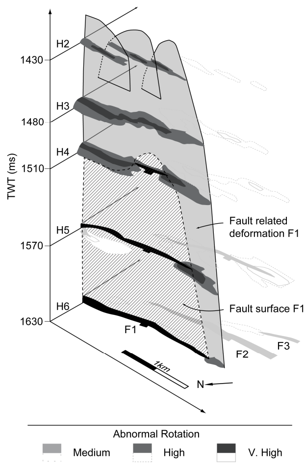
Fig. 3.10. A composite 3D view showing the distribution of the high and very high levels of abnormal rotation in the volume surrounding the mapped F1 fault segment. The cross-hatched area represents the mapped F1 fault surface. A variable thickness zone of fault-related deformation encircles fault F1, grey area.
