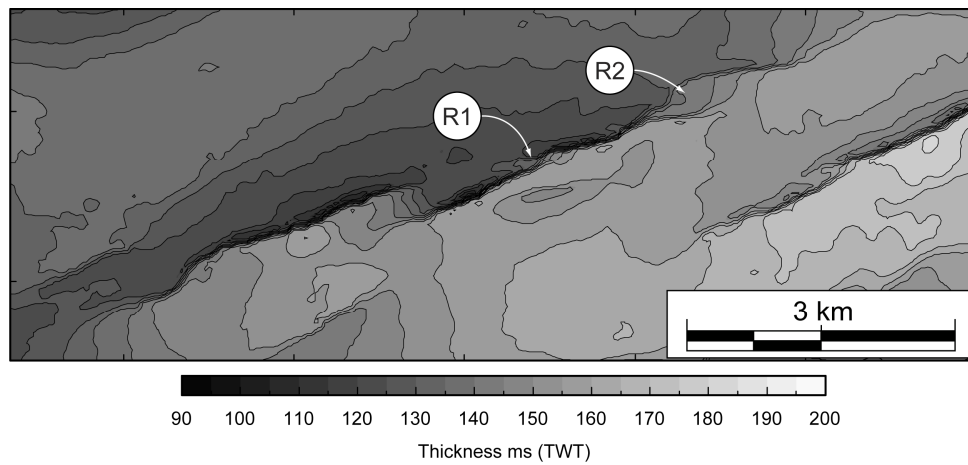
Fig. 4.5. An isochron map for the growth packages from horizon H4 to horizon H2, which are intersected by the studied faults. Horizon H4 is the base of the syn-sedimentary sequence (Fig. 4.4). The changes in accommodation space delimit the location of active faulting at the time of deposition. Relay ramps R1 and R2 are labelled. All fault segments on the NE-SW trending fault-array are active during the same time.
