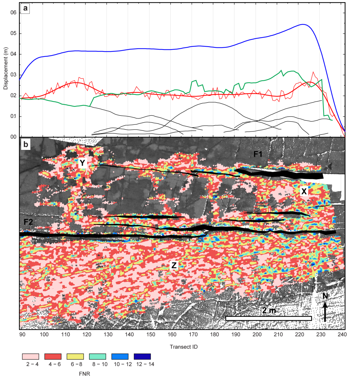
Fig. 2.13. (a) Displacement distance plot for the Lilstock relay ramp ( Fig. 2.12 ). Black lines are throw profiles for the individual fault polygons in (b). The thin red line is the vertical displacement calculated from areas of FNR (b: pinks to blue). The green line is the aggregate displacement for all the fault polygons. The thick red line is a smoothed version of the thin red line, which removes the low level noise relating to erosion features and vegetation on the wave-cut-platform. (b) Map view of coloured laser scan data and overlying FNR maps. Faults F1 and F2 are parallel with near constant separation along-strike. Internal faulting forms en-echelon patterns between F2 and F1 and also trend parallel to the main bounding faults and vein orientations within the ramp. The mottled FNR map results from small (1-5 mm) undulations in the bedding surface due to the preferential erosion of veins and fractures. (X) The ramp has more rotations towards the mutual hanging wall in the east than the west. (Y) A zone of high FNR exist along-strike of the bounding fault F1. (Z) A ~2 m wide zone of high FNR stretches along the length of the relay ramp in the mutual footwall.
