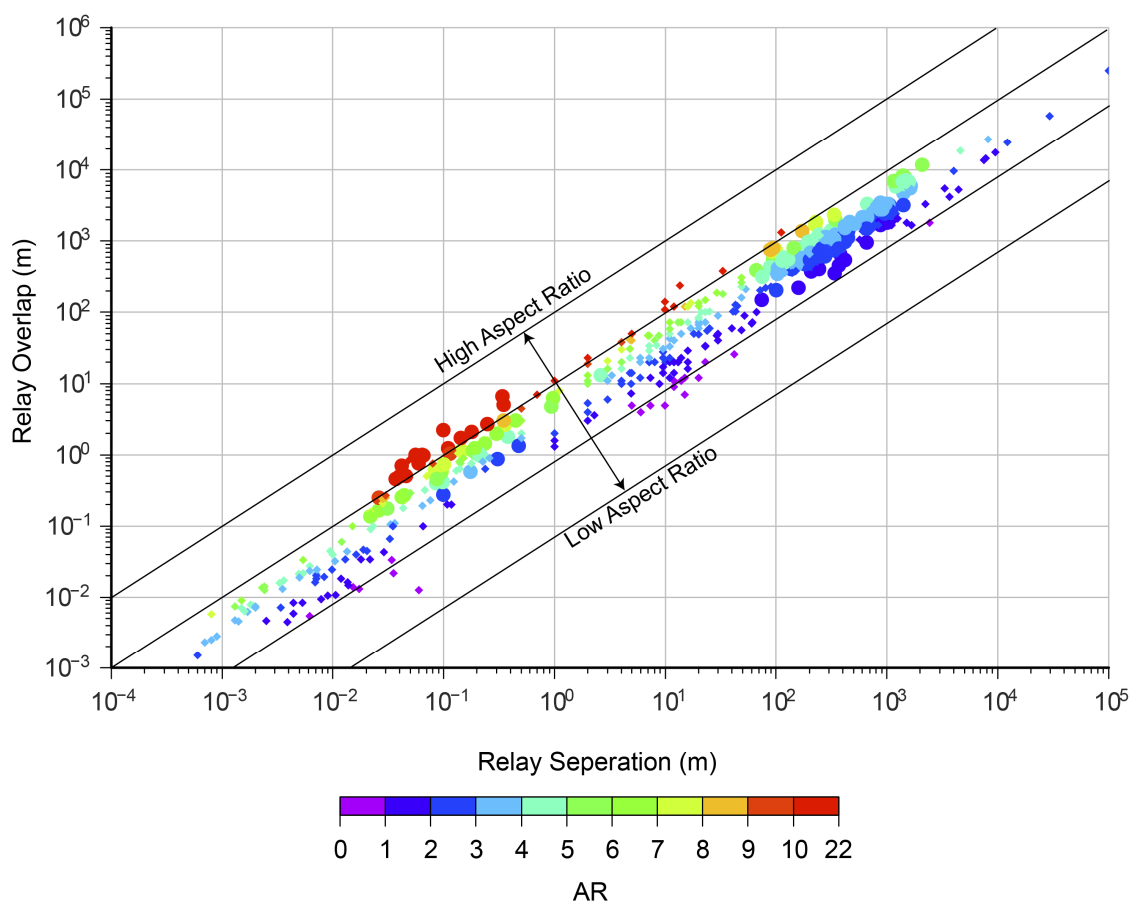
Fig. 5.14. Log log plot of relay overlap versus separation for data collected in this study (circles) and from literature sources (diamonds). Relay ramp measurements collected in this study (circles) show higher AR (reds) at outcrop-scales (i.e. relay ramp separations < 10 m) compared to data collected from seismic datasets (i.e. relay ramps with separations > 100 m). In general, over nearly 9 orders of magnitude there is approximately an equal amount of scatter of measurements about a single power-law trend. Literature sources used in this plot are recorded in appendix 5: Relay table 2.
