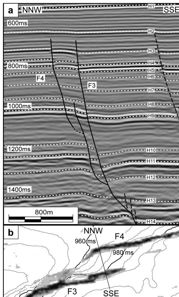
Fig. 4.13. (a) A seismic profile through Laminaria R2 (Fig. 4.6). The separation distances between faults F3 and F4 decreases at 1100 ms TWT and is associated with a shallowing of the fault dip. F4 links at depth with F3 below H12. The amount by which the ramp is rotated towards the mutual hanging wall varies on each horizon. Both fault tips terminate at the same level within the growth sequence. (b) Map view distribution of fault enhanced Ant-Track attributes. The SW tip of F4 has rotated and is shown to cross the ramp. Time depth contours display the internal form of the ramp, which dips towards the SE.
