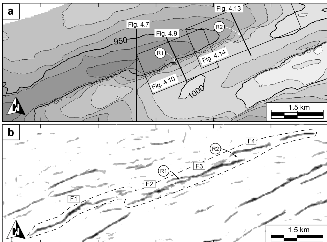
Fig. 4.5. An isochron map for the growth packages from horizon H4 to horizon H2, which are intersected by the studied faults. Horizon H4 is the base of the syn-sedimentary sequence (Fig. 4.4). The changes in accommodation space delimit the location of active faulting at the time of deposition. Relay ramps R1 and R2 are labelled. All fault segments on the NE-SW trending fault-array are active during the same time.
