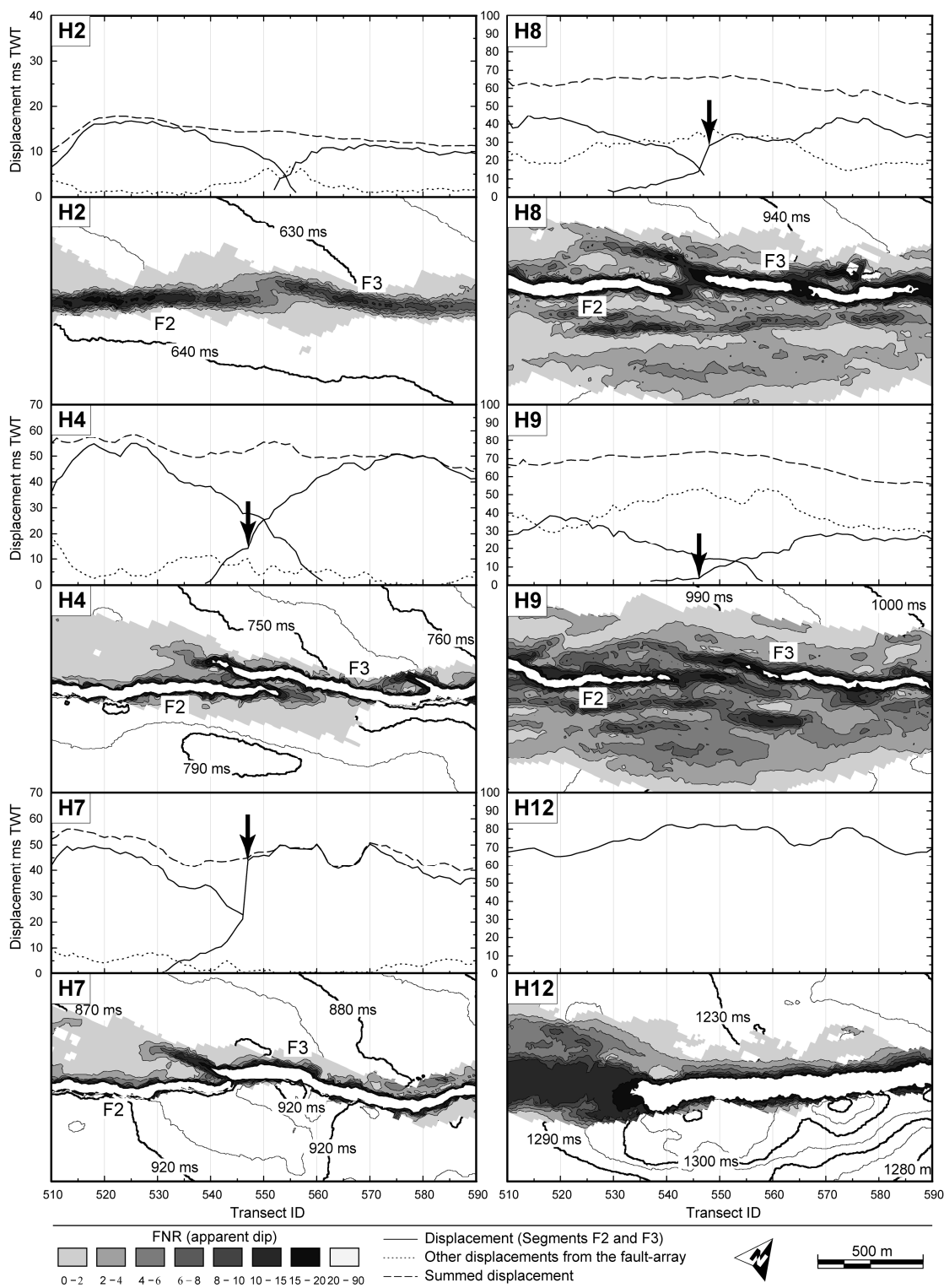
Fig. 4.10. A selection of six mapped horizons that intersect relay R1 (Fig. 4.9). For each horizon there is a detailed map view image showing the distribution of continuous deformation (FNR). Above which are the corresponding displacement distance profiles, which show the amount of displacement occurring across the areas depicted in map view (shaded areas). Displacement is split into the vertical offsets on fault scarps F2, F3, and all other structures, which can include both rotated horizons and minor faults in the footwall and hanging wall. At all levels within the relay zone the displacement distance profiles are geometrically coherent. See text for detailed descriptions of each horizon.
