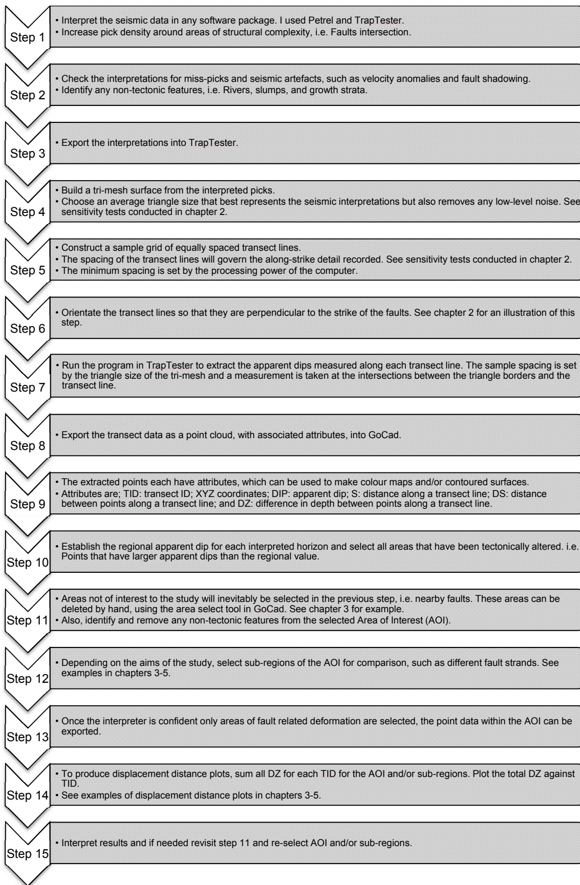
Fig. A3. Workflow for building and a digital surface from seismic data and extracting FNR data for interpretation.
