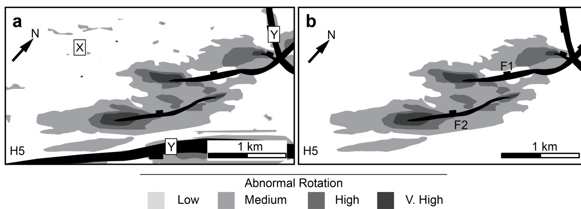
Fig. 2.9. (a) Areas of abnormal rotation where all apparent dips above the defined background regional values are selected, resulting in the selection of miss-picks and artefacts (X), and geometries on adjacent faults (Y). (b) Features, such as X and Y are removed to leave the abnormal rotations (FNR) attributed to the studied fault-array (F1 and F2).
