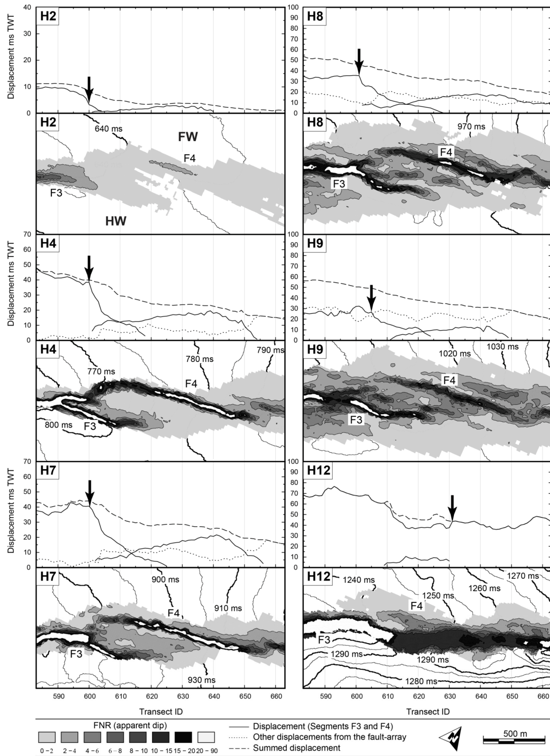
Fig. 4.14. A selection of six mapped horizons that intersect relay R2 (Fig. 4.13). For each horizon there is the map view distribution of FNR and the corresponding displacement distance profiles. Displacement is split into the vertical offsets on fault scarps F3, F4, and all other structures, which can include both rotated horizons and minor faults in the footwall, hanging wall, and relay ramp. As with Laminaria R1, Laminaria R2 remains geometrically coherent on every horizon. See text for a detailed description of each horizon.
