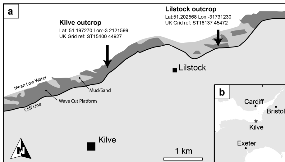
Fig. 5.5. (a) Outcrop locations from Kilve and Lilstock. (b) Location of Kilve in the UK.
