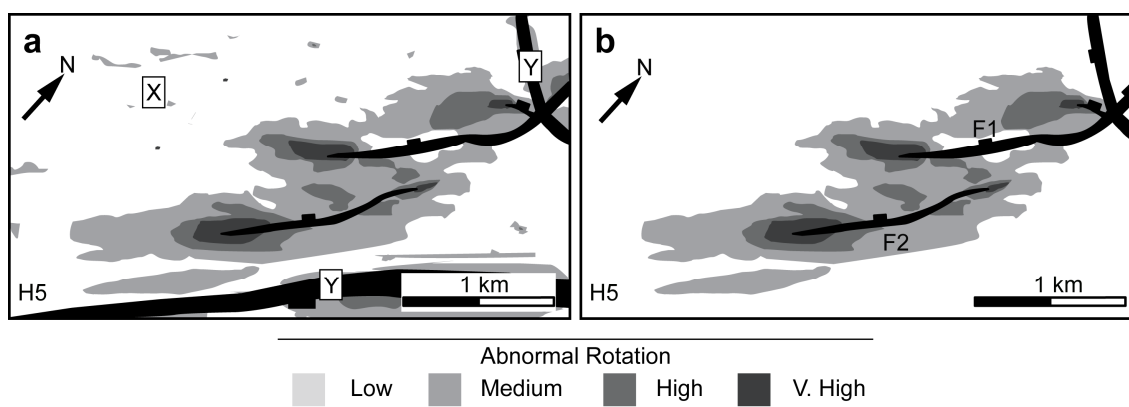
Fig. 3.8. (a) Areas of abnormal rotation where all apparent dips above the defined background regional values are selected, resulting in the selection of miss-picks and artefacts (X), and geometries on adjacent faults (Y). (b) These features are removed to leave the abnormal rotations attributed to the studied fault-array.
