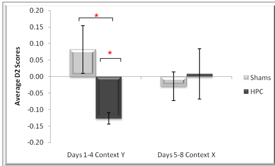
Figure 4.8: Average D2 Scores What-Where Days 1 to 4 (Y) and Days 5 to 8 (X) (± SEM)
