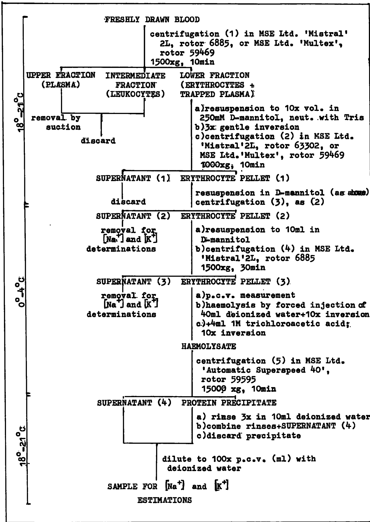
FIG. V-1. PREPARATION OF ERYTHROCYTES FOR [Na + ] i AND [K + ] i ESTIMATIONS.
