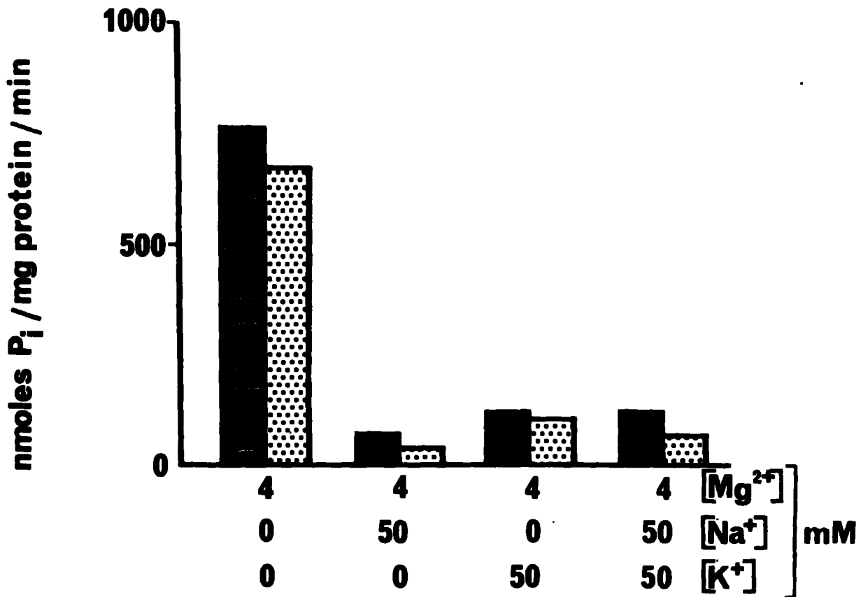
FIG. III-9. EFFECT OF 5 \times 10^{-4} M OUABAIN UPON ATP HYDROLYSIS IN THE PRESENCE OF Mg^{2+} , Na^+ AND K^+ FOR A D-MANNITOL-EXTRACTED RAT SKELETAL MUSCLE MICROSOMAL PREPARATION.
