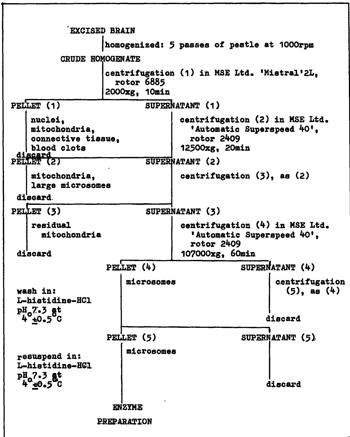
FIG. VI-1. PROCEDURE FOR THE EXTRACTION OF RAT BRAIN MICROSOMES.
