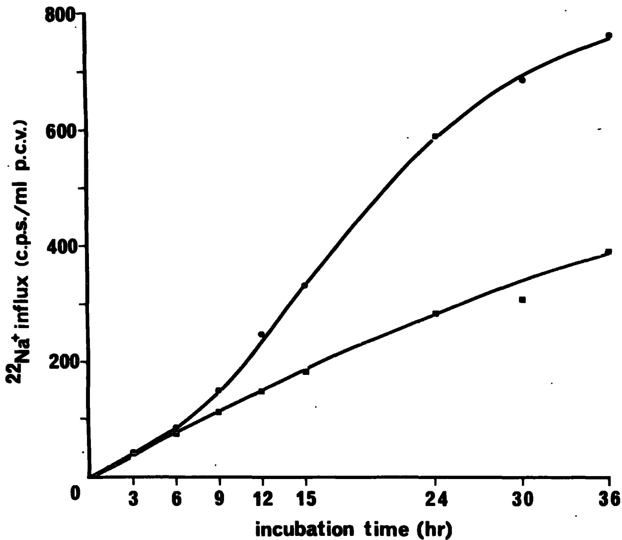
FIG. V-4. INFLUENCE OF 1 \times 10^{-5} \text{M} TANNIC ACID UPON ^{22}\text{Na}^+ LOADING OF RAT ERYTHROCYTES.
