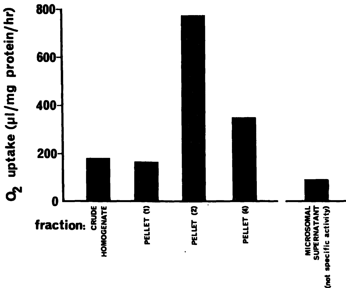
FIG. III-10. SUCCINATE DEHYDROGENASE ACTIVITY IN RAT SKELETAL MUSCLE FRACTIONS.
