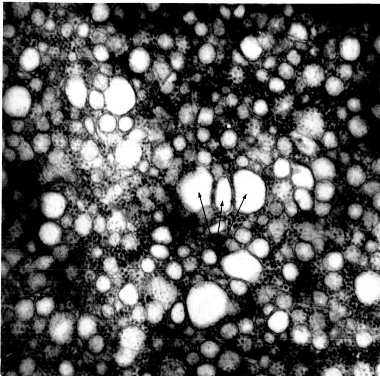
FIG. III-16. ELECTRONMICROGRAPH SHOWING THE GENERAL APPEARANCE OF THE 10 000-107 000xg FRACTION OF A RAT SKELETAL MUSCLE HOMOGENATE.
