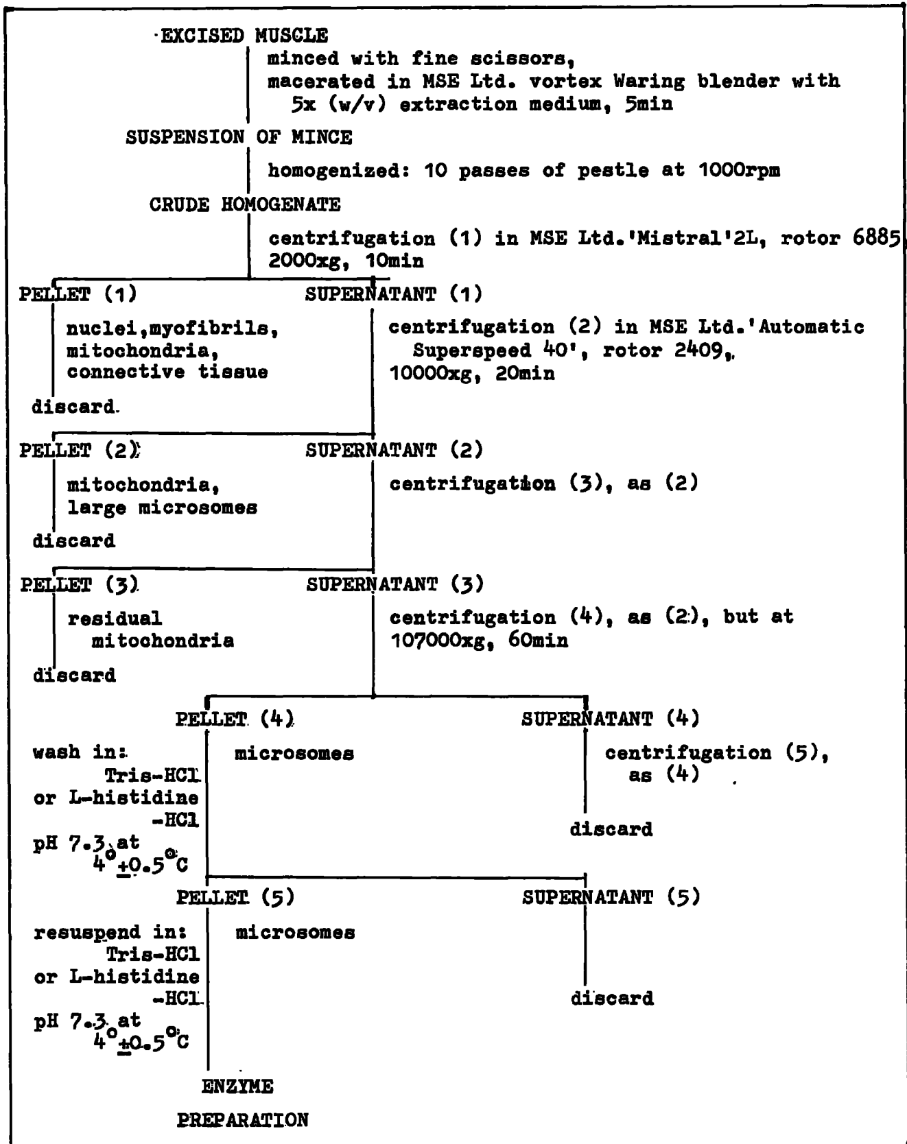
FIG. III-1. PROCEDURE FOR EXTRACTION OF SKELETAL MUSCLE MICROSOMES.
