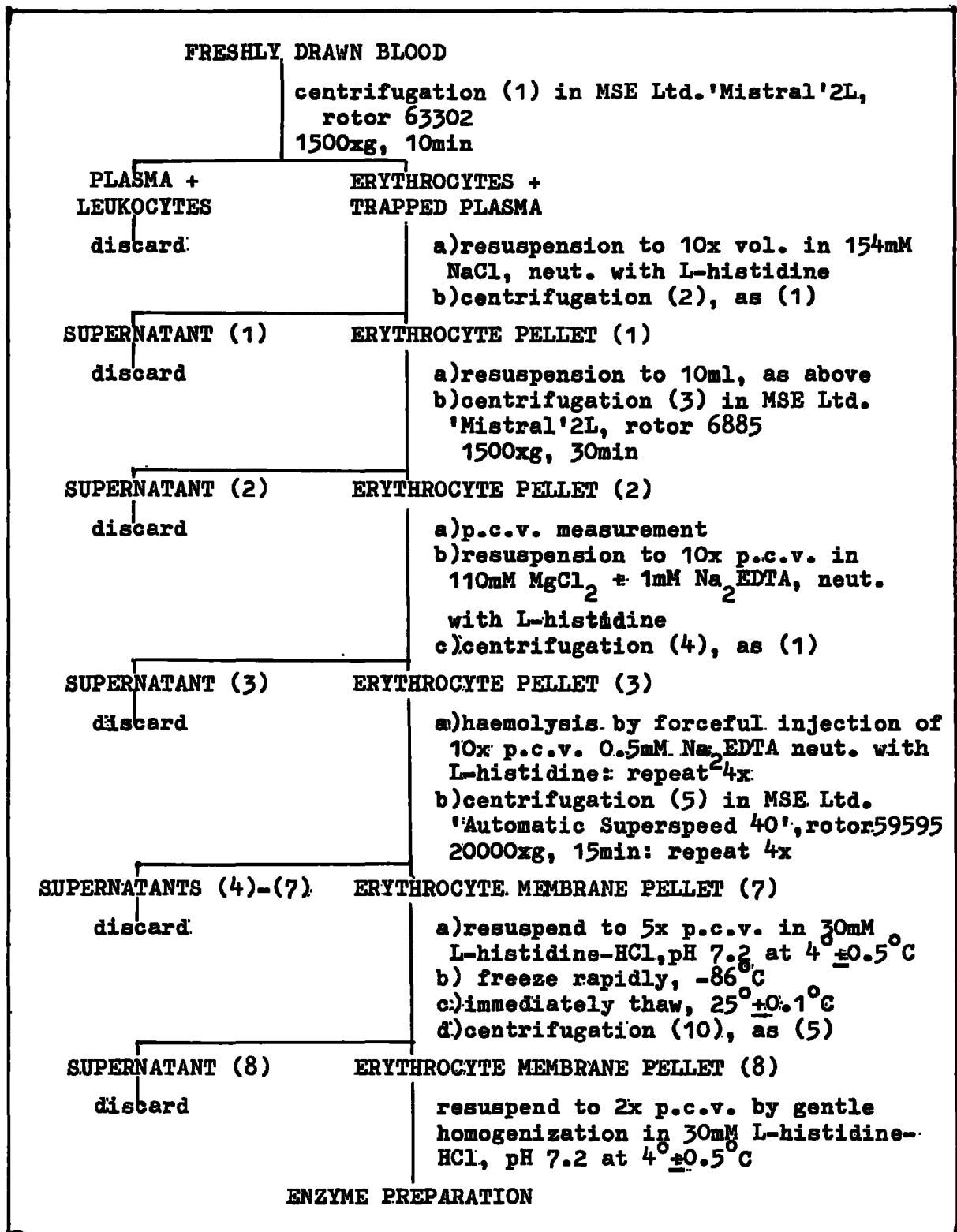
FIG. V-12. PREPARATION OF ERYTHROCYTE MEMBRANE FRAGMENTS.
