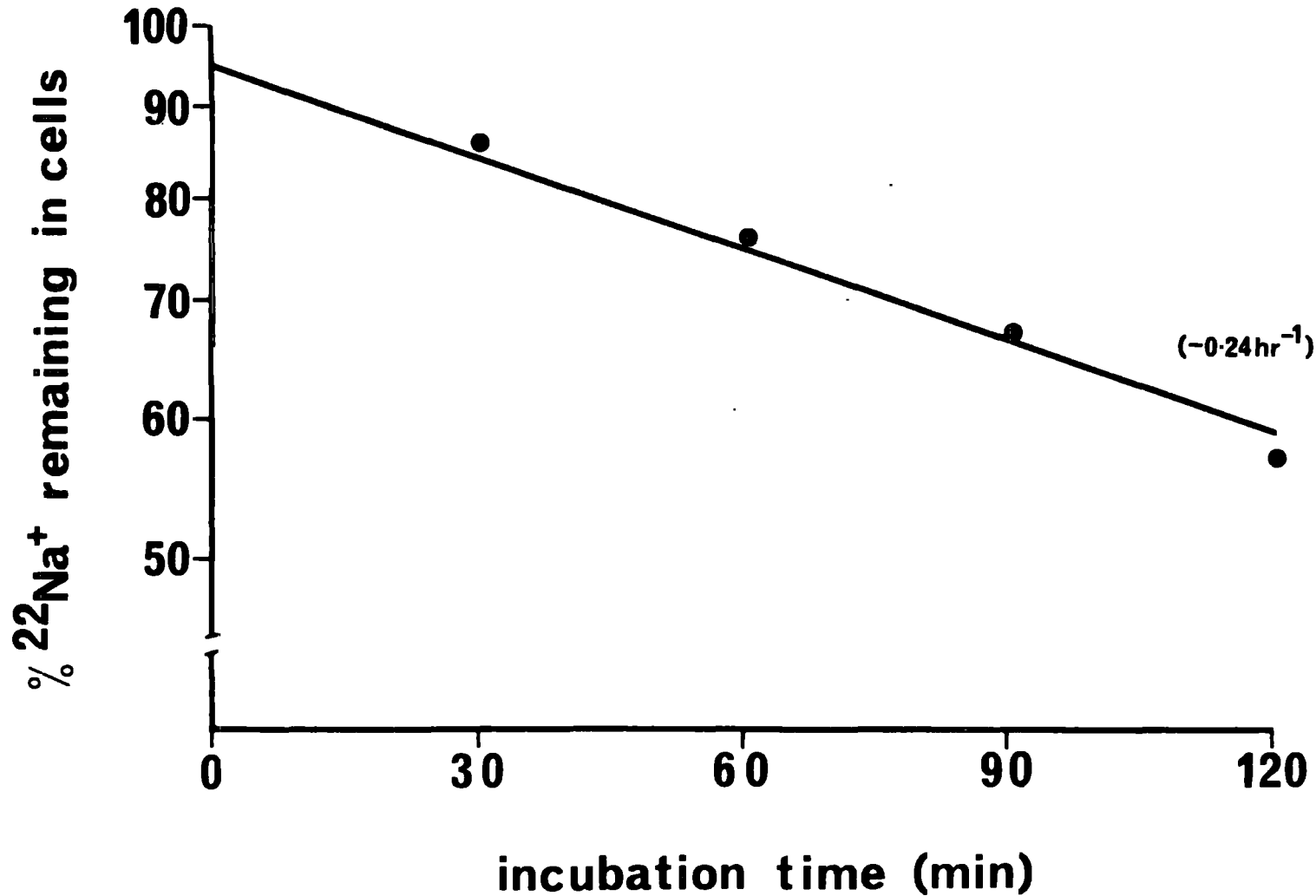
FIG. V-5. ^{22}\text{Na}^+ EFFLUX FROM NORMAL HUMAN ERYTHROCYTES.
