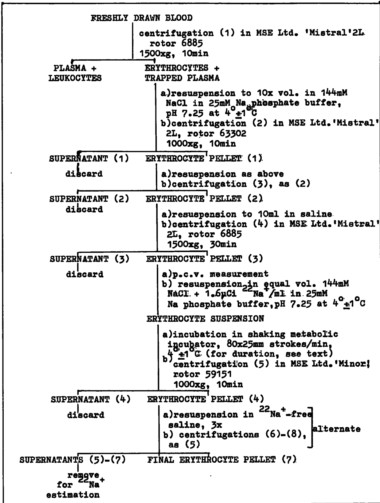
FIG. V-2. PREPARATION OF 22 Na + -LOADED ERYTHROCYTES.
