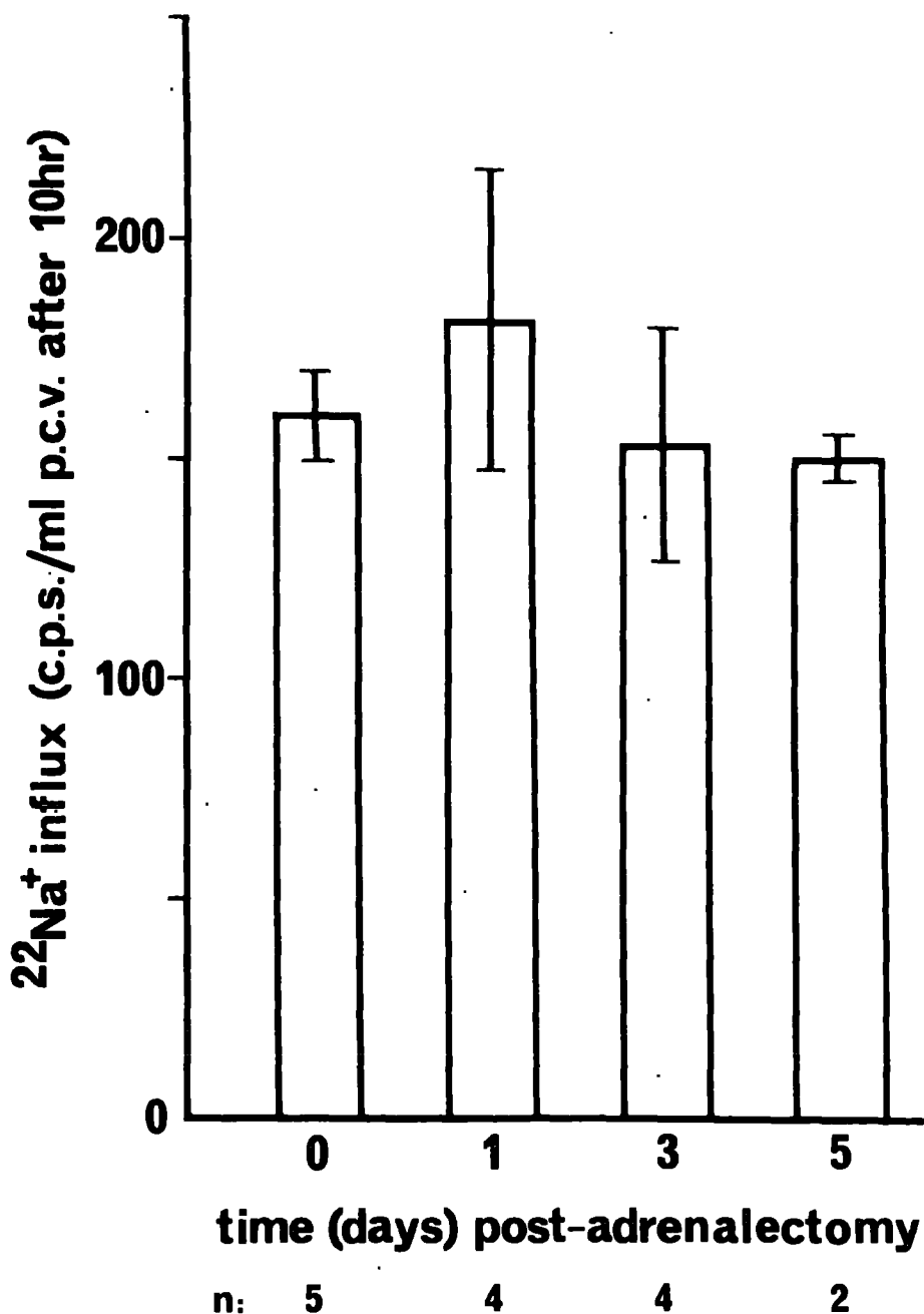
FIG. V-3. INFLUENCE OF ADRENALECTOMY UPON ^{22}\text{Na}^+ LOADING OF RAT ERYTHROCYTE
