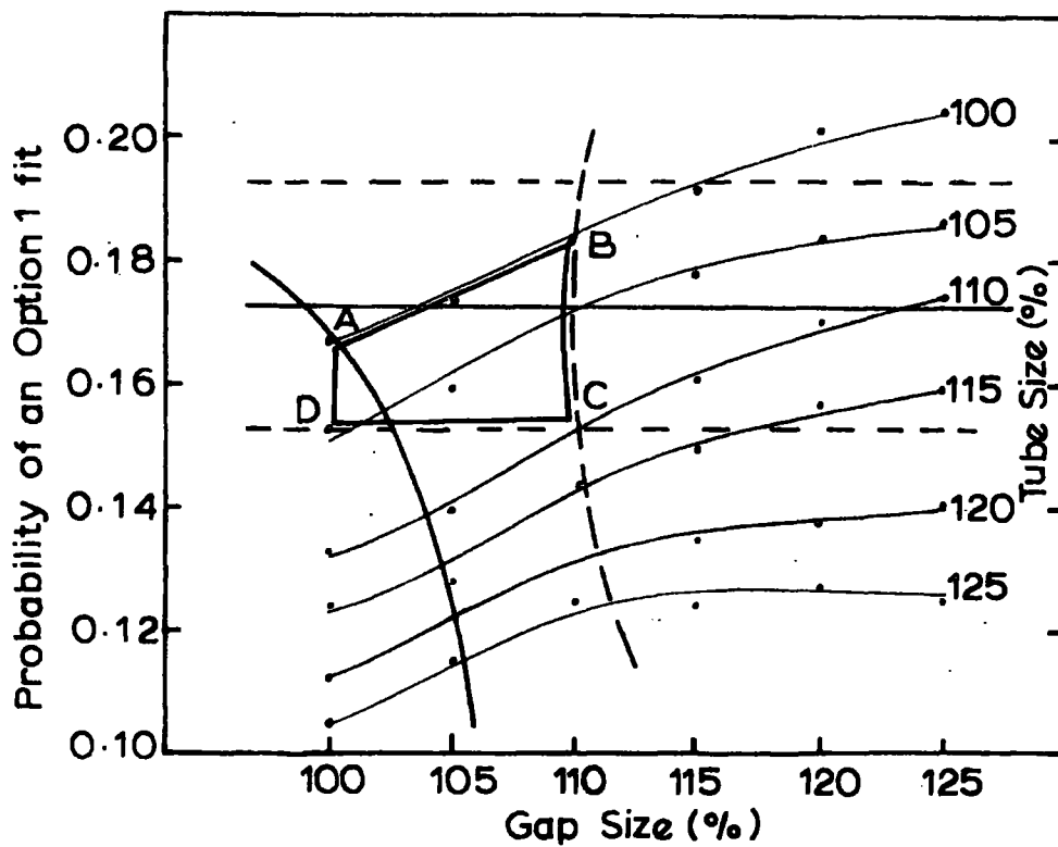
Figure 5.9 The Limits which can be set on the Gap and Tube Sizes.
