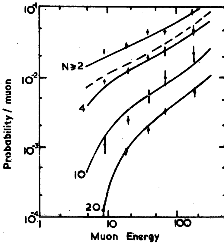
Figure 7.6 The Burst Size Probability for Muons in Iron.
