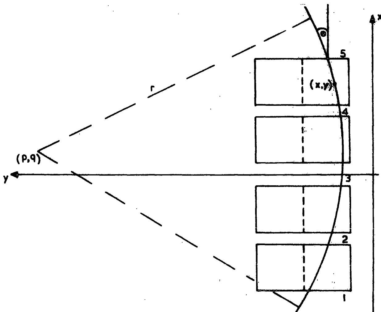
Figure 3.9 The Co-ordinate Frame of the Spectrograph.
