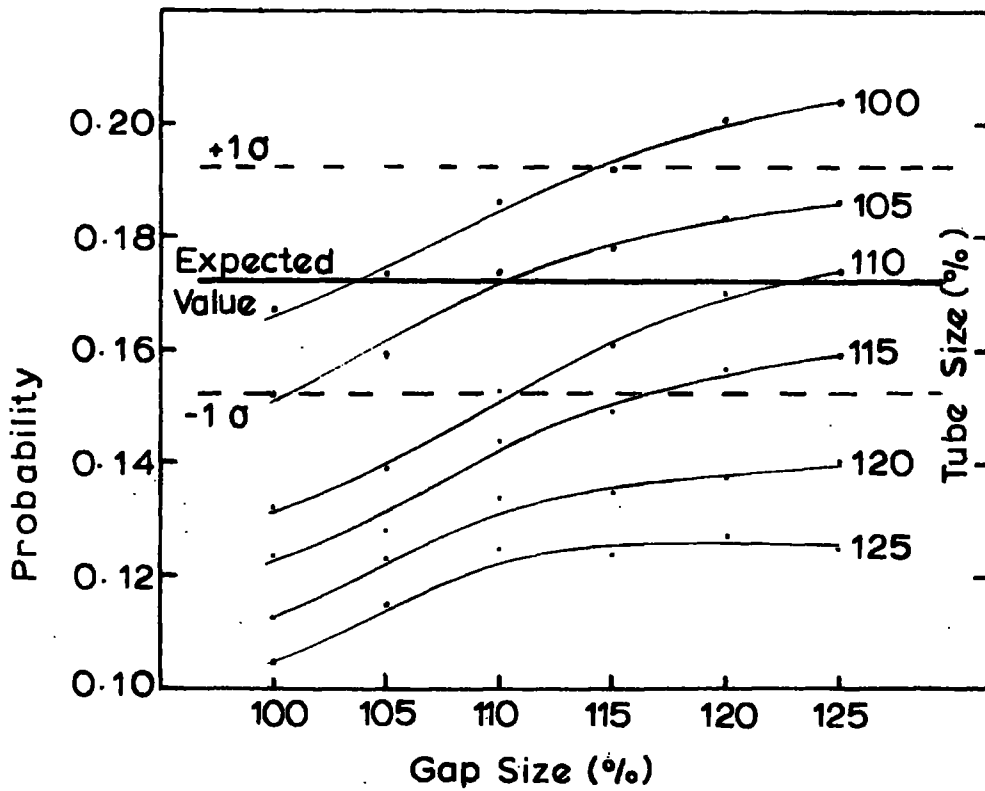
Figure 5.7 The Probability of an Option 1 Fit as a Function of Tube and Gap Size.
