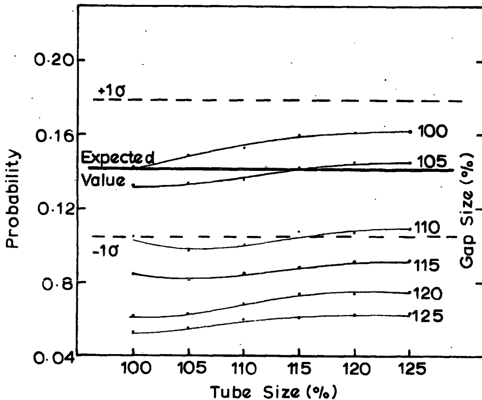
Figure 5.8 The Probability of an Option 2 Fit as a Function of Tube and Gap Size.
