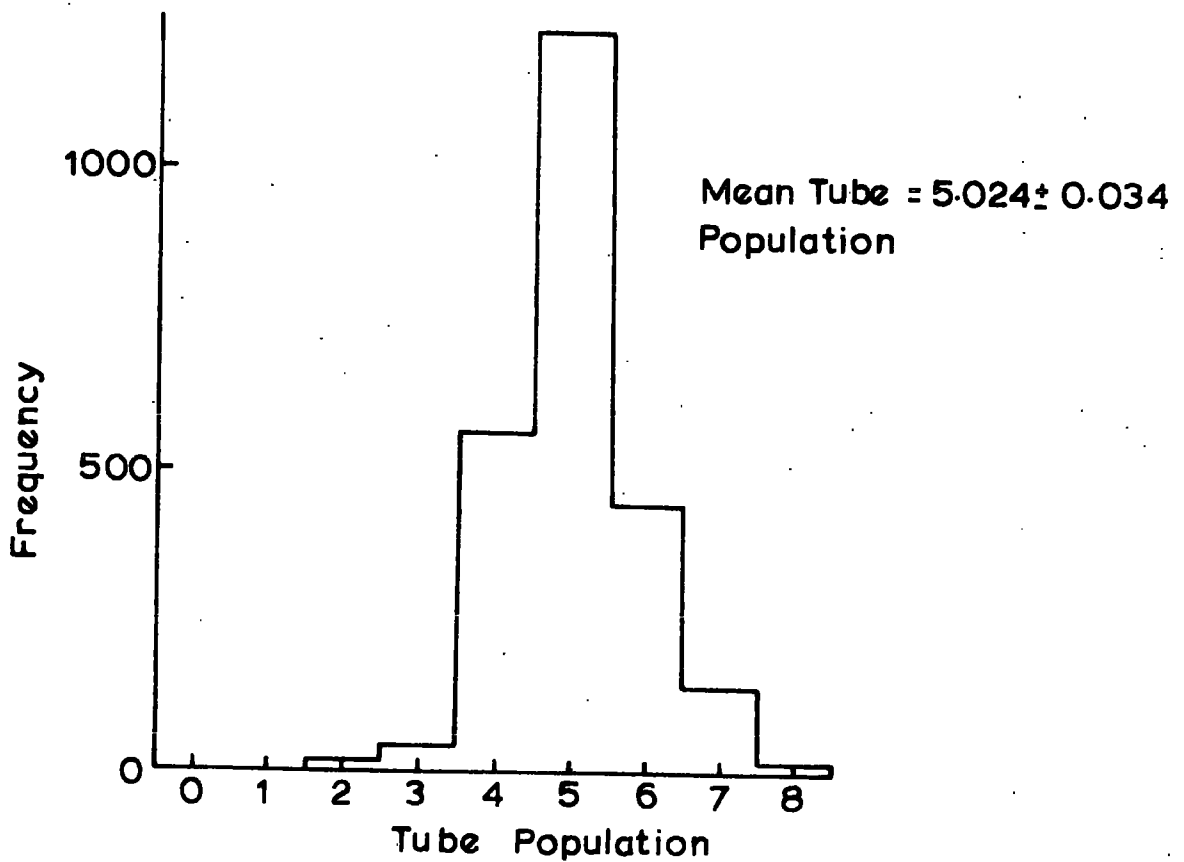
Figure 5.6 The Tube Population Distribution
