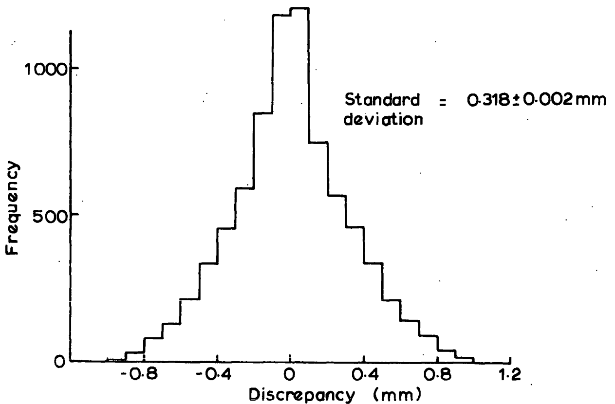
Figure 5.10 The Frequency Distribution of the Discrepancies between the True and Computed Trajectories in a Tray.
