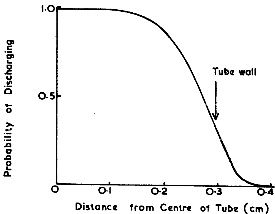
Figure 3.2 The Flash-tube Discharge Probability Function of Bull et al. (1962)
