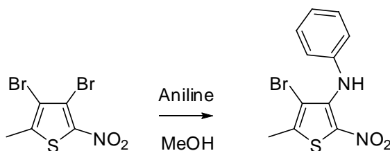
Scheme 1.48
