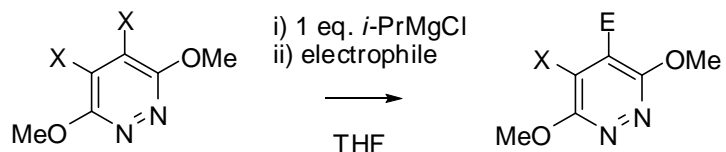
Scheme 1.21
