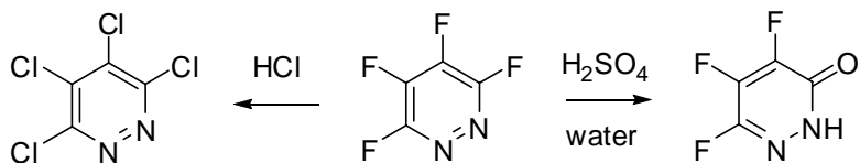
Scheme 2.6
