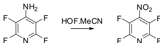
Scheme 3.8
