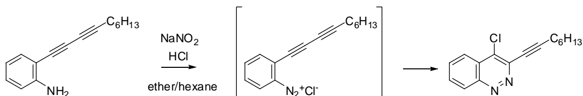
Scheme 1.5
