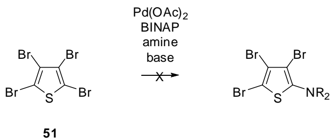
Scheme 4.10
