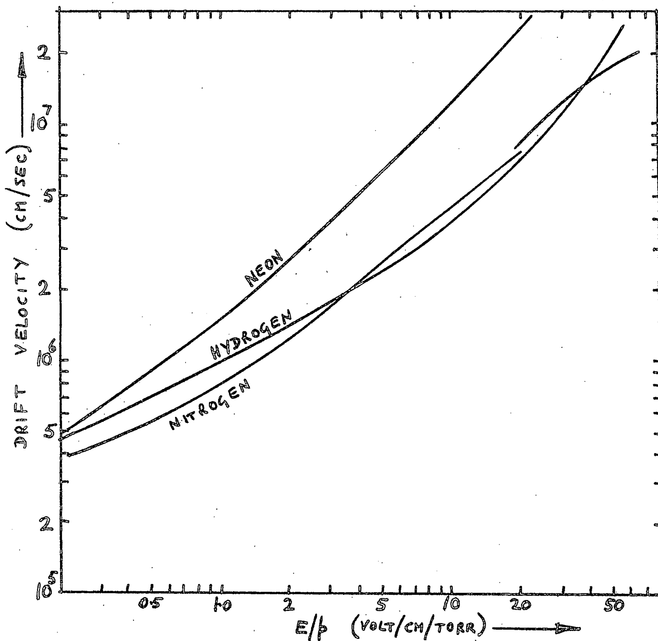
FIG 8.5 DRIFT VELOCITIES OF ELECTRONS IN HYDROGEN (30,34) NITROGEN (30,35) AND NEON (35)
