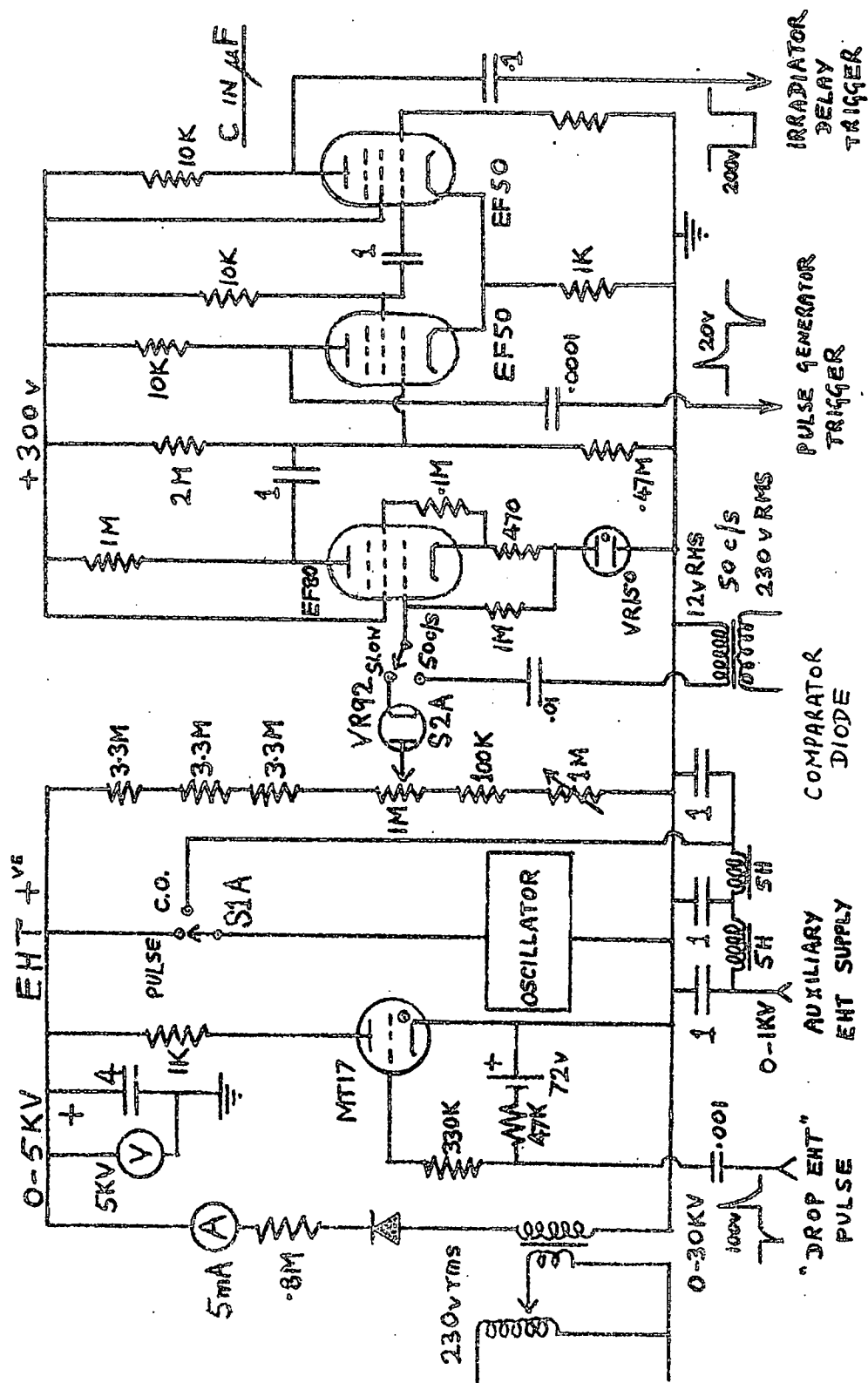
Fig 4.4 EHT AND COMPARATOR CIRCUIT
