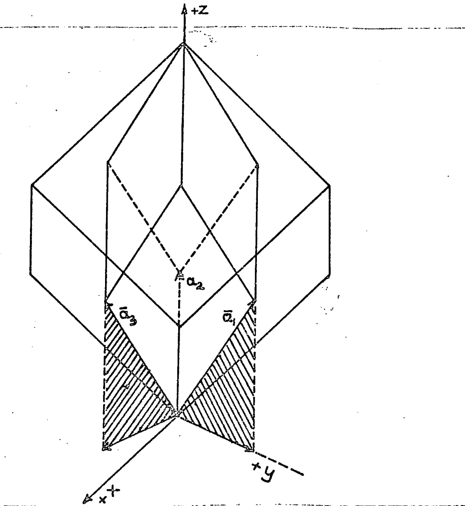
Figure (2-1) : The relationship between the cubic lattice and the rhombohedral unit cell of the A7 structure.
