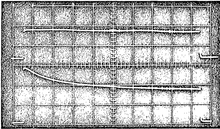
Figure 2. Receiver output display: upper trace, off magnetic resonance; lower trace, on magnetic resonance. 0.2 at. % Cr ruby at 4.2°K. Horizontal scale 2 msec per division.
