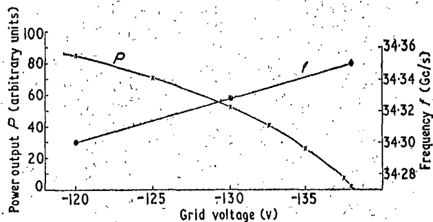
Figure 4. Grid characteristics of the klystron type R5146 taken at constant reflector voltage.
