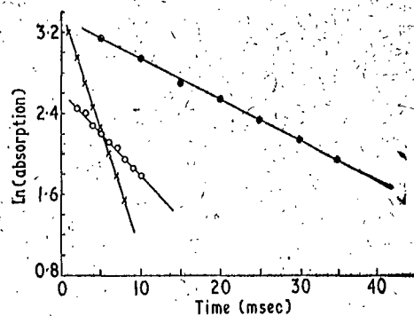
Figure 3. Relaxation data derived from pulse-response traces: open circles, -\frac{3}{2} to -\frac{1}{2} transition, 0.2 at. % Cr ruby, T_1 = 12.0 msec; full circles, -\frac{1}{2} to +\frac{1}{2} transition, 0.052 at. % Cr ruby T_1 = 24.5 msec; crosses, -\frac{1}{2} to +\frac{1}{2} transition, 0.2 at. % Cr ruby, T_1 = 3.5 msec. All measurements taken at 35.5 Gc/s, 4.2°K, \theta = 90^\circ .
