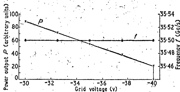
Figure 5. Grid characteristics of the klystron type 8RK19 taken at constant reflector voltage.
