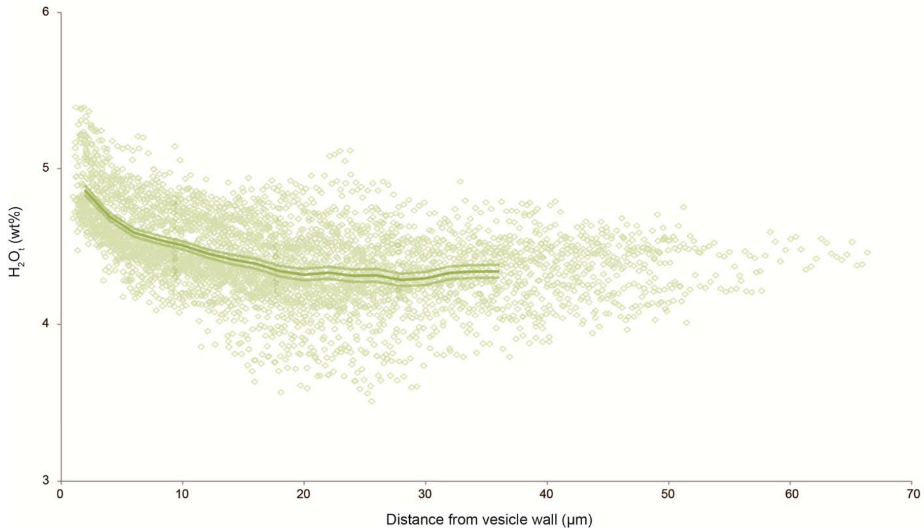
Fig. A2.3 Full extracted H_2O_1 dataset and calculated mean H_2O_1 concentration profile for sample ABG6
