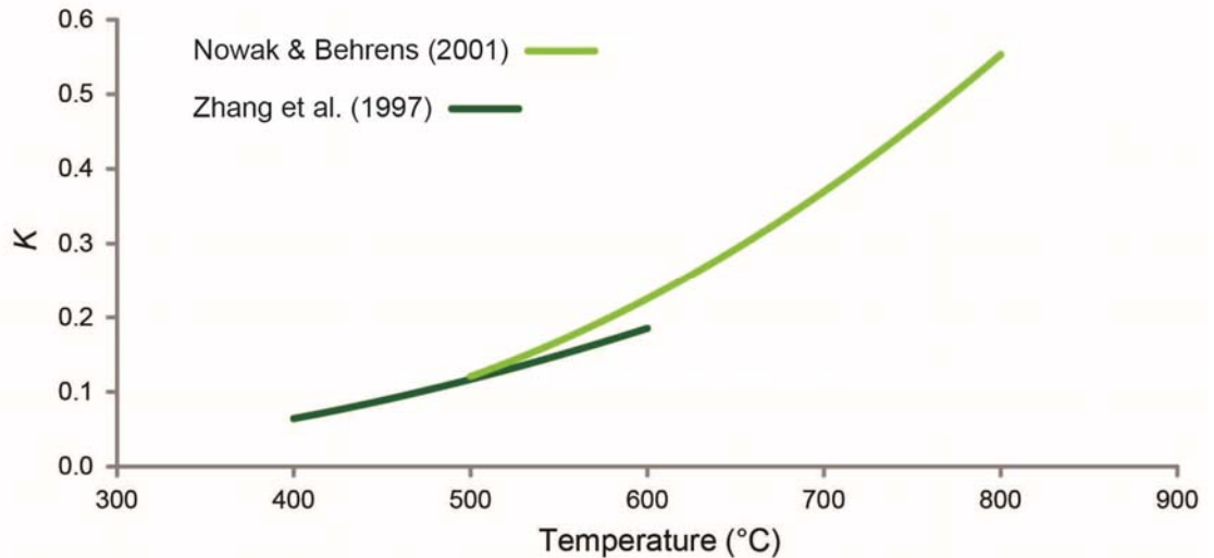
Fig. 2.7 Temperature-dependence of equilibrium H 2 O speciation constant K
