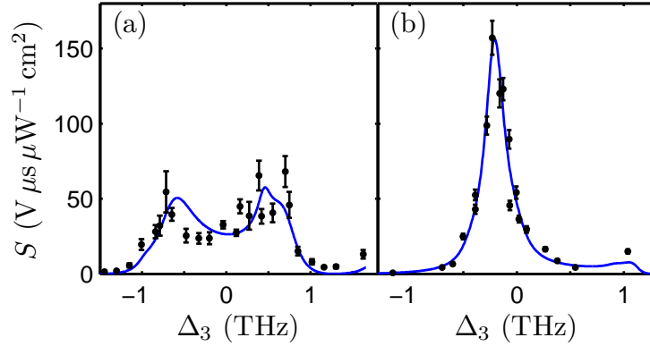
Figure 5.5: (a) The autoionization spectrum of the 5s19d\ ^1D_2 state. (b) The autoionization spectrum of the 5s20s\ ^1S_0 state. Solid lines are six-channel MQDT model fits, and the fit parameters are listed in tables D.2 and D.1.
