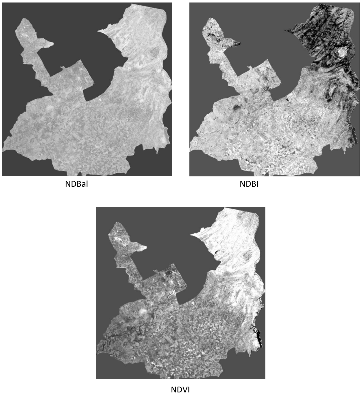
Figure 6.2: Application of different Indices on Landsat TM 1998
